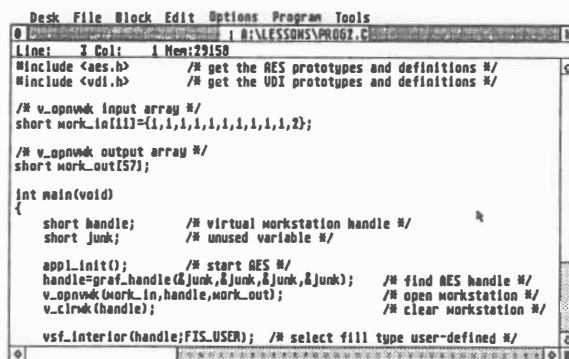
The PROG2.C Program
