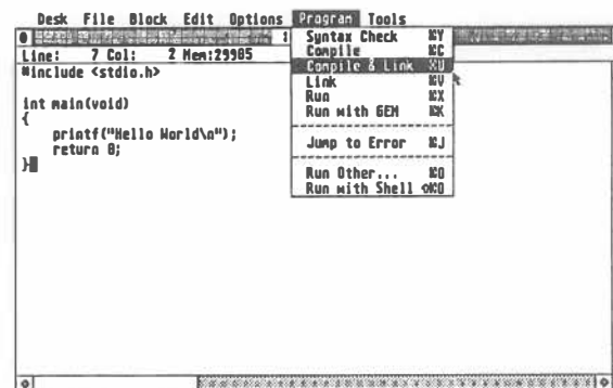
The Program menu before Compile & Link
