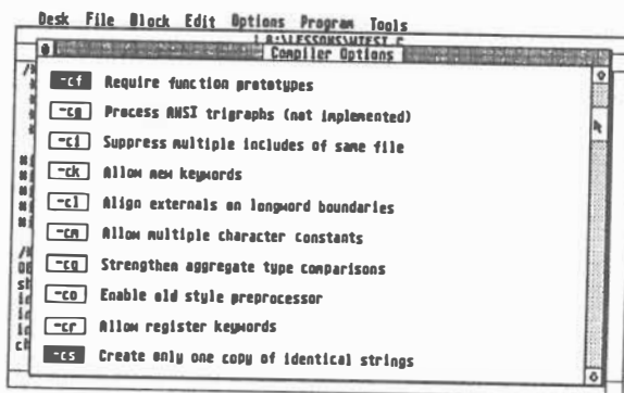
The Compiler Options list
