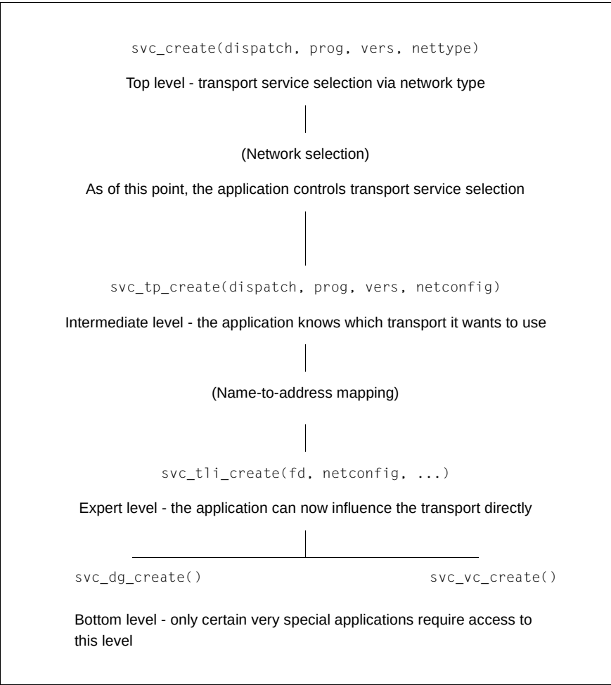
Figure 3: Lower levels of RPC, server end
