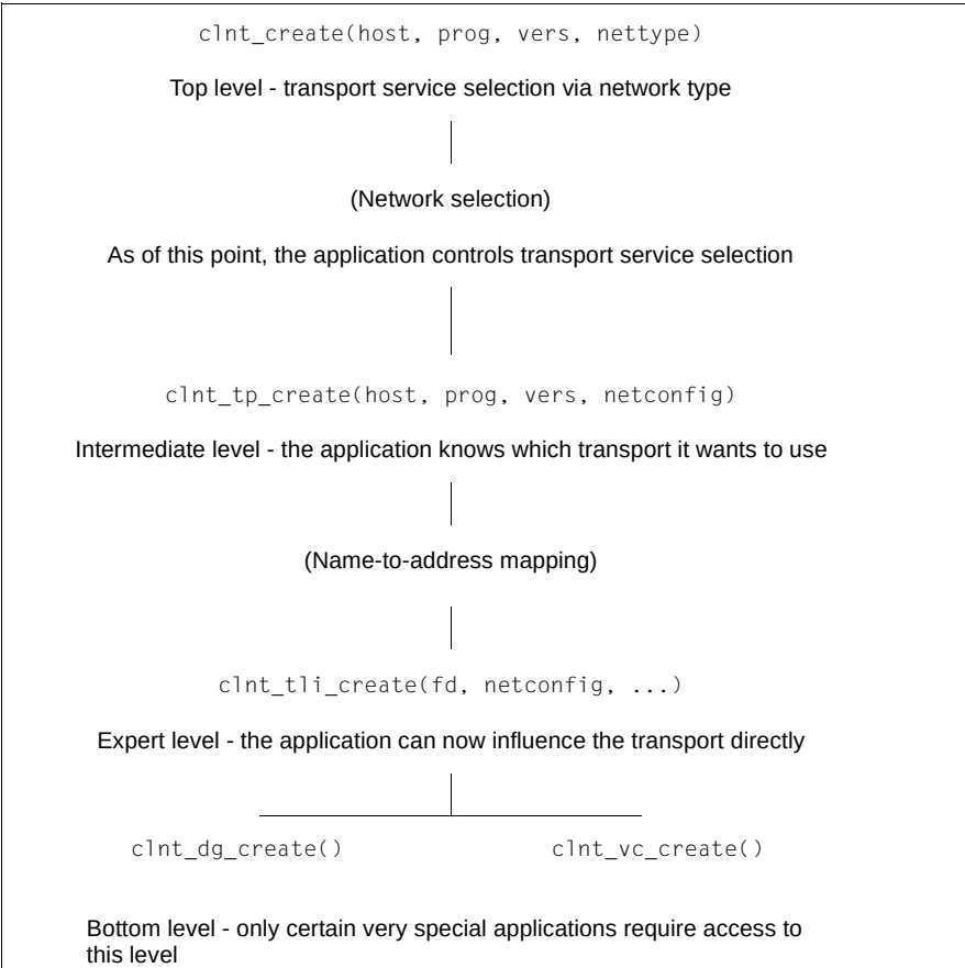
Figure 2: Lower levels of RPC, client end
