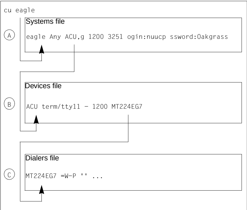
Figure 17: Links between the Systems, Devices and Dialers files
