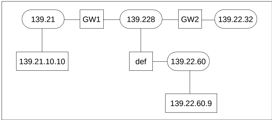
Figure 6: Best match algorithm - restrictions
