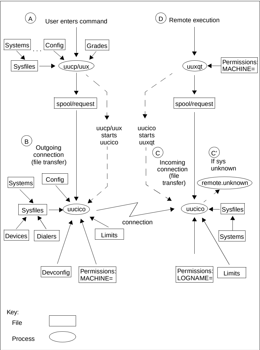
Figure 16: How the Basic Network Utilities work
