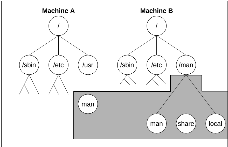
Figure 11: Mounting a remote resource
