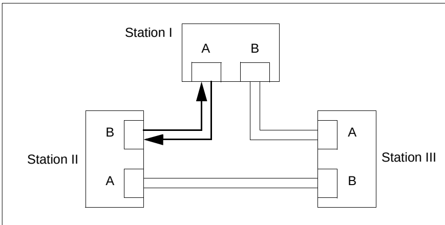
Figure 24: Wrapping in the event of a station failing (station III)
