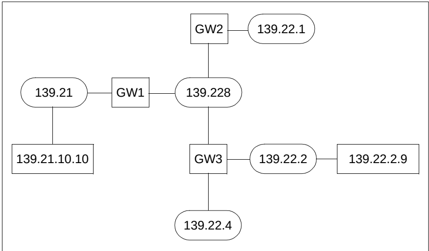
Figure 5: Best match algorithm
