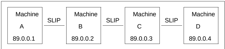
Figure 29: Routing with SLIP connections
