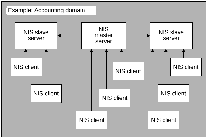
Figure 12: NIS servers and NIS clients
