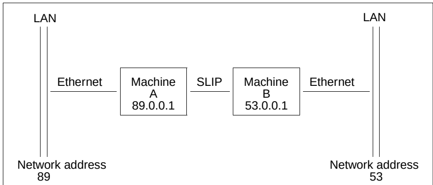
Figure 30: Routing with coupling of two Ethernet networks
