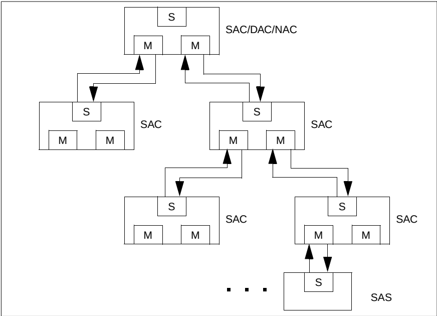
Figure 22: Tree structure
