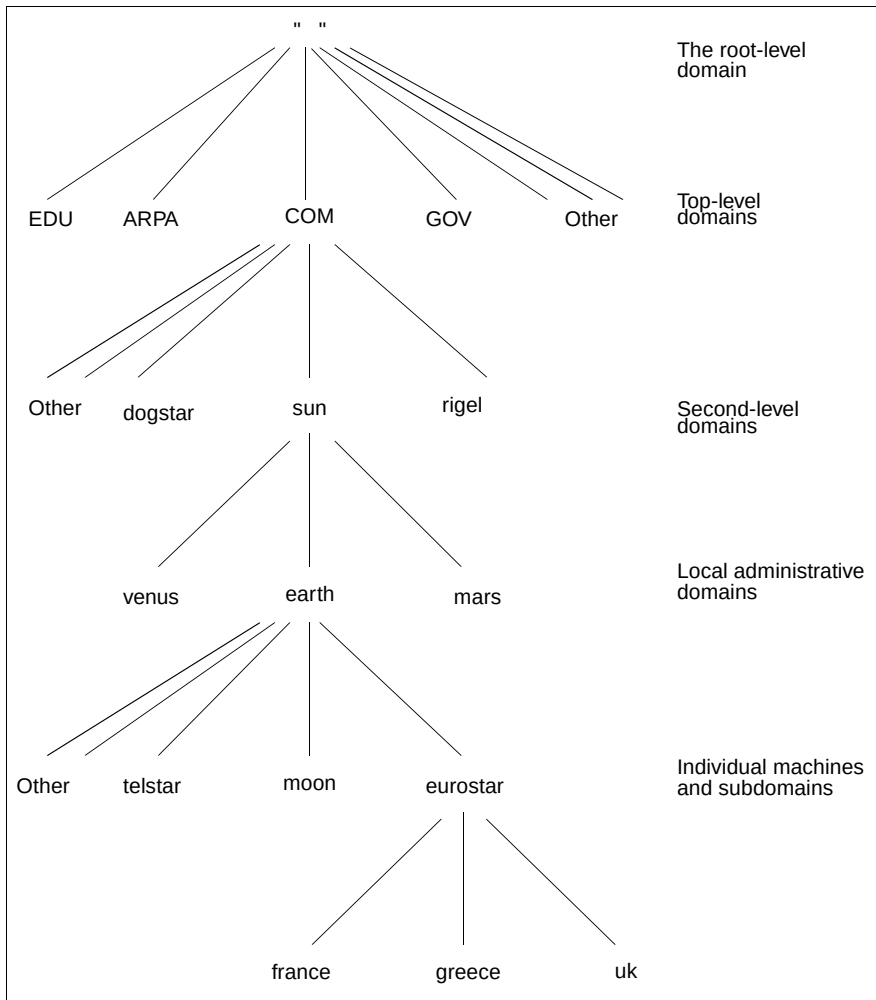
Figure 3: Example of an Internet domain hierarchy
