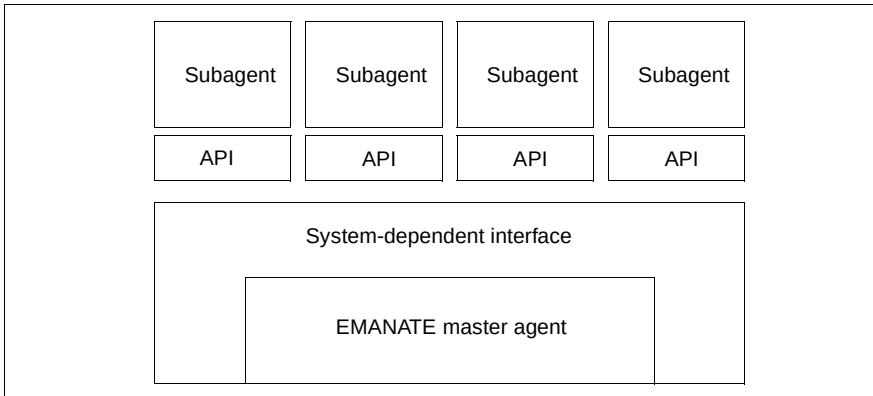
Figure 13: EMANATE agent architecture
