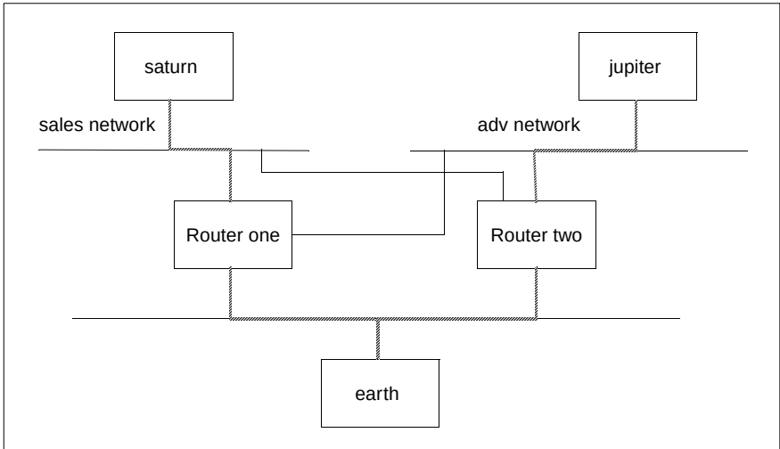
Figure 7: Example of a network configuration with several routers
