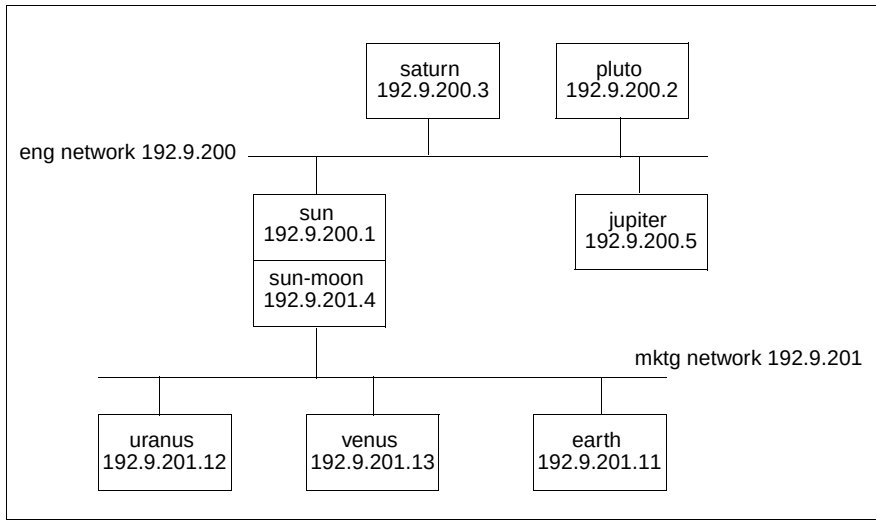
Figure 4: Sample configuration: static routing
