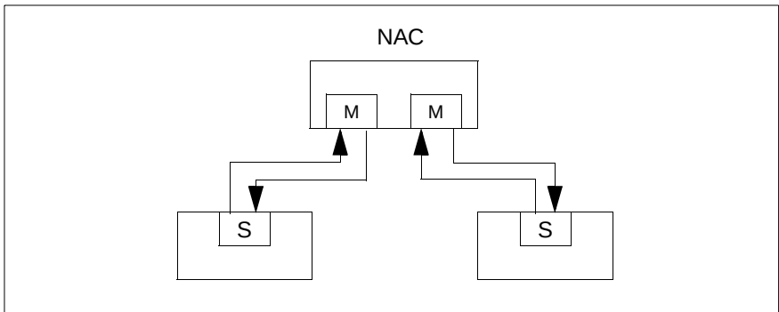
Figure 23: Null attachment concentrator
