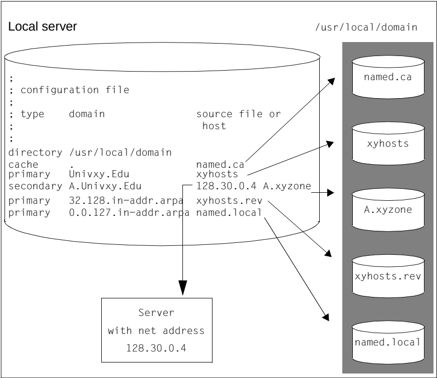
Figure 9: Configuration file and data files
