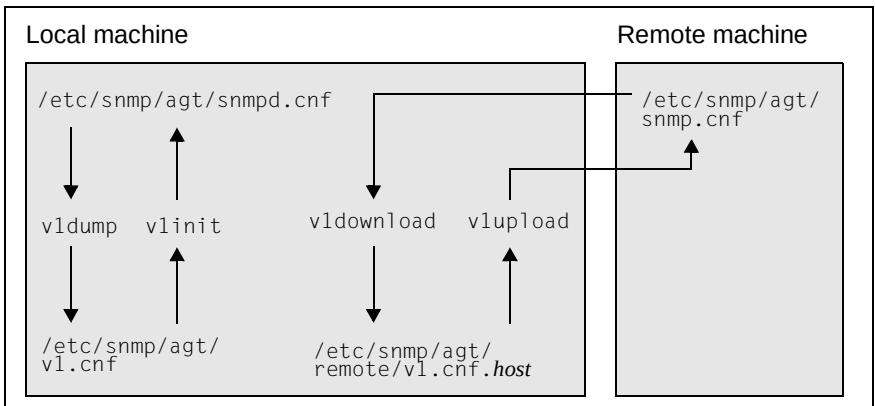
Figure 15: Interaction of tools for generating EMANATE configuration files
