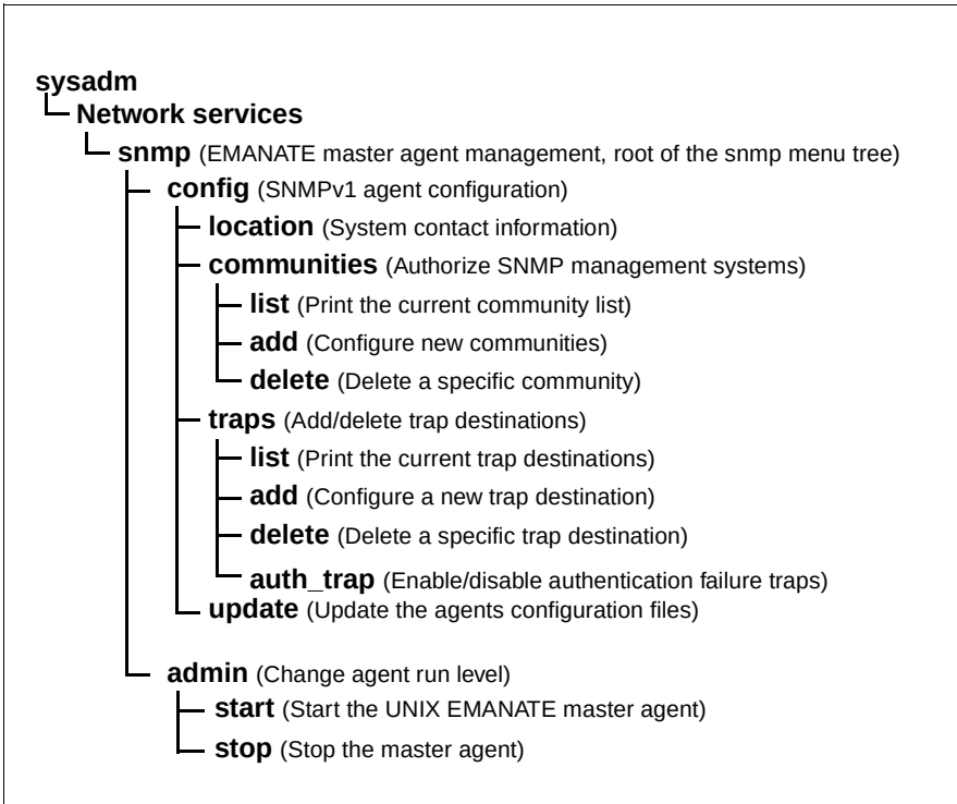
Figure 14: snmp menu tree in sysadm
