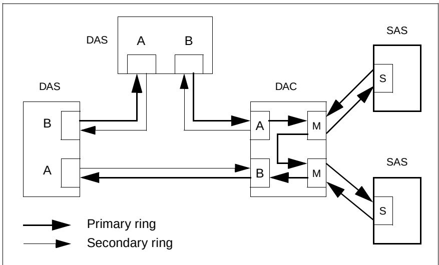
Figure 21: Dual attached stations and a dual attached concentrator
