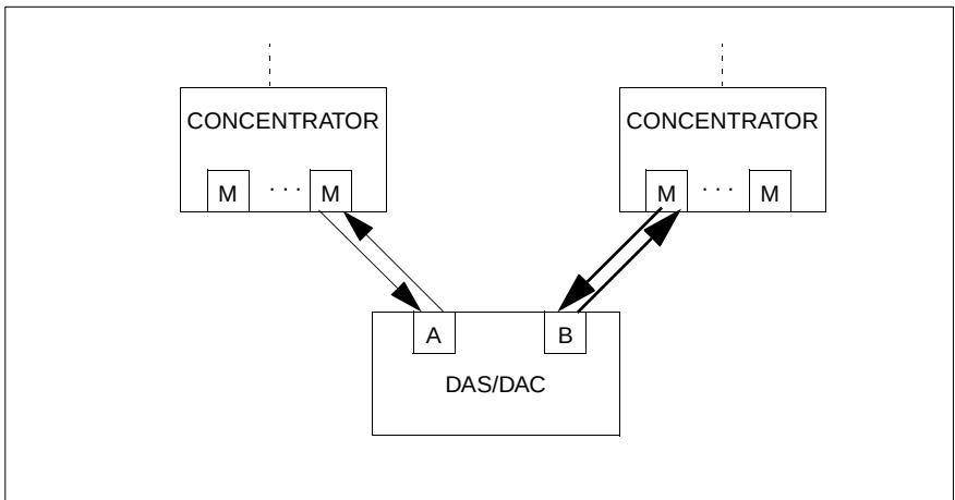
Figure 25: Dual homing
