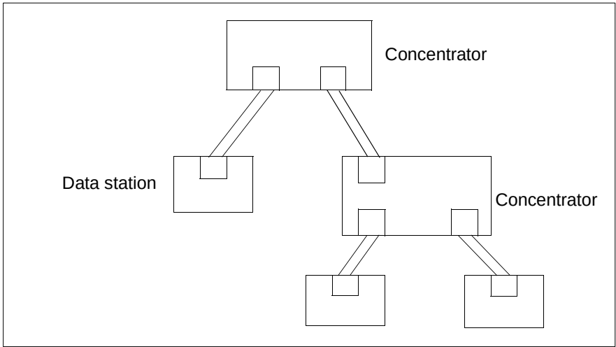
Figure 20: Components of an FDDI ring
