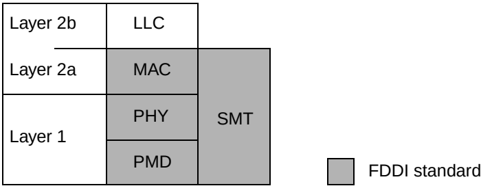
Figure 19: FDDI ISO layers
