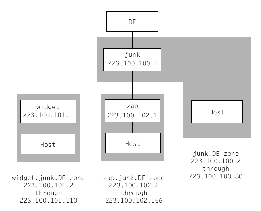
Figure 10: The sample network
