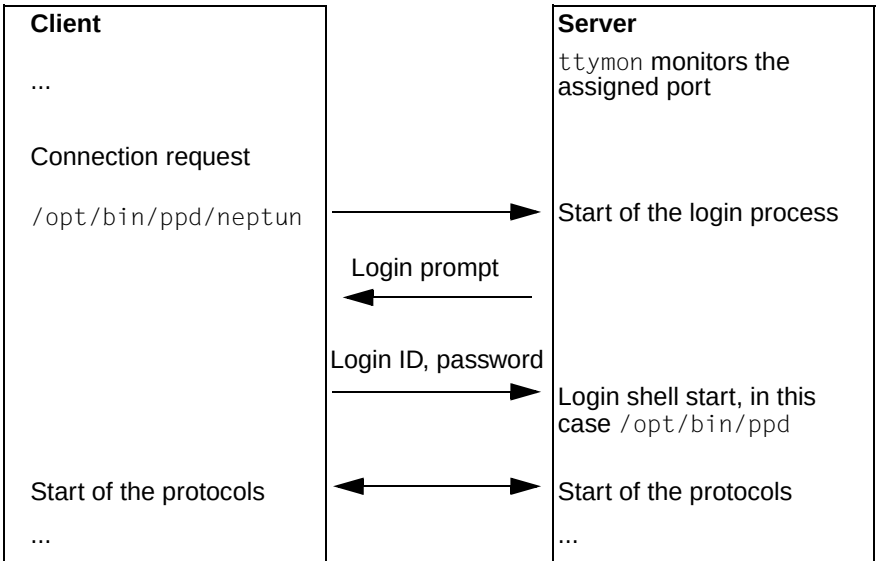
Figure 31: Establishing a connection between a PPP client and server
