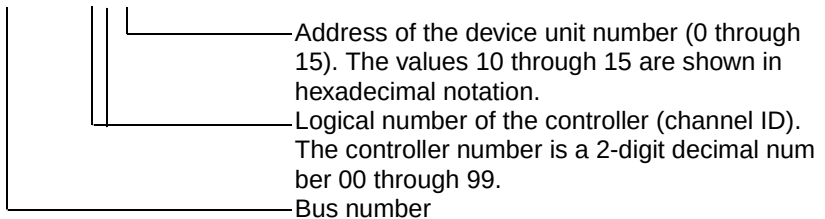
Figure 27: Syntax of the logical names used for hard disks
