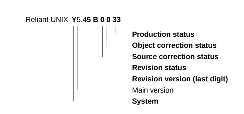
Figure 11: Structure of the operating system names for Reliant UNIX
