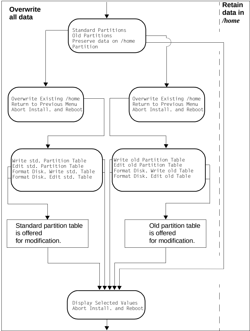
Figure 14: Formatting/partitioning dialog sequences
