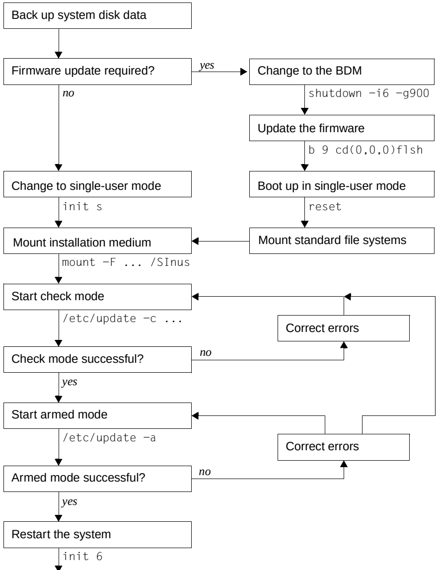
Figure 17: Performing an update installation in a 64-bit environment
