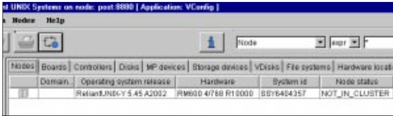
Figure 19: Example: Window showing an “empty” administration domain (excerpt, approx. fig.)
