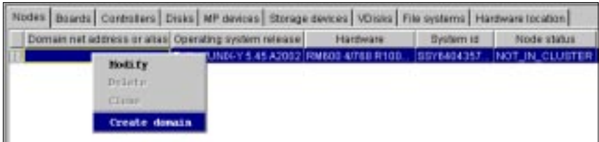
Figure 20: Example: Creating an administration domain and the first node (excerpt, approx. fig.)
