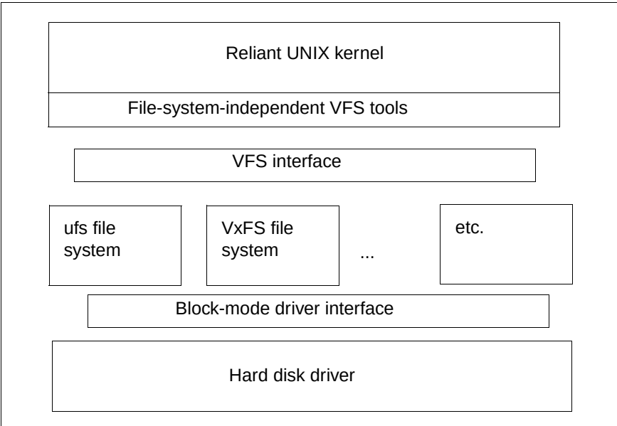
Figure 2: Modular file system integration in Reliant UNIX
