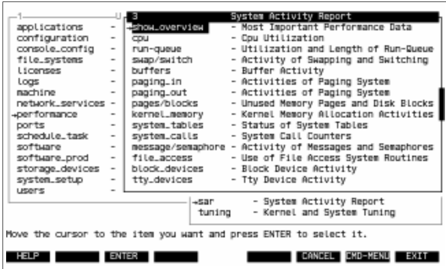
Figure 8: Selecting system activity reporting with sysadm (example)
