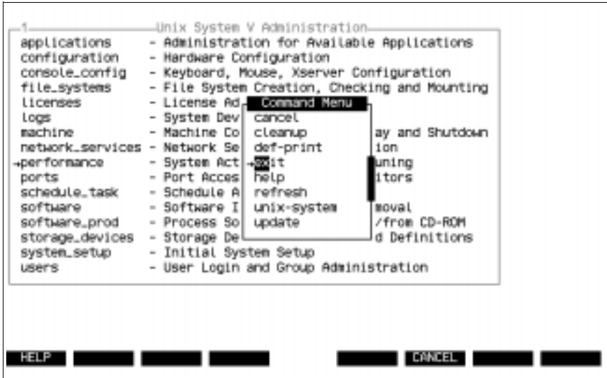
Figure 10: Typical sysadm command menu
