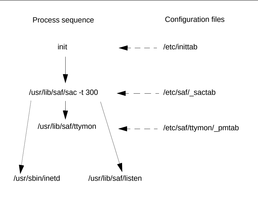
Figure 5: Port monitoring model
