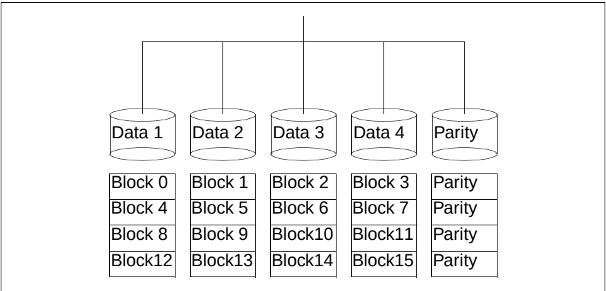
Figure 14: RAID level 4
