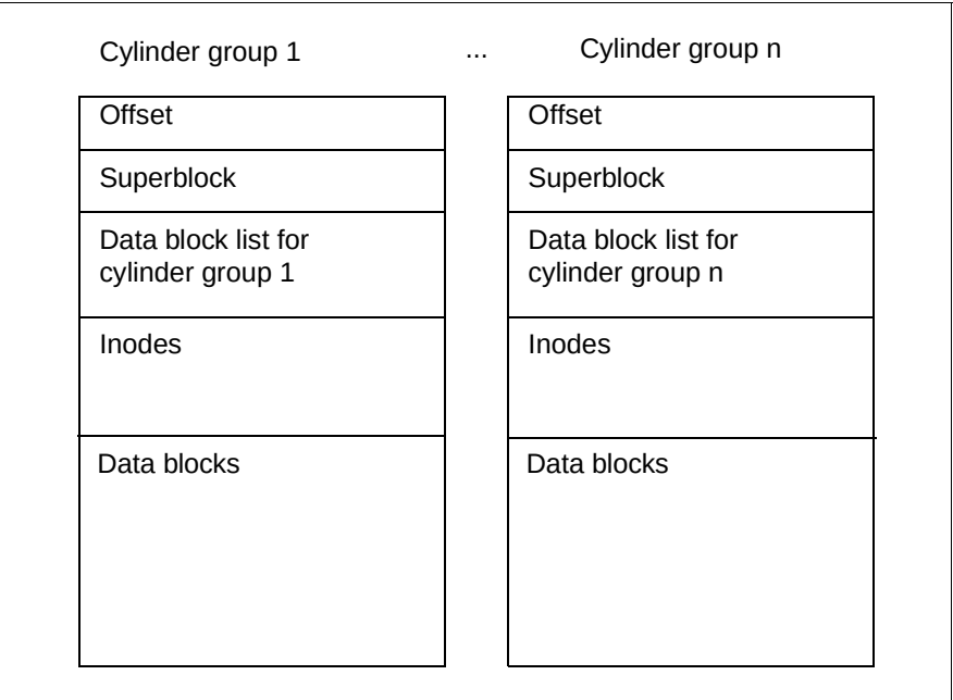
Figure 4: File system types: ufs
