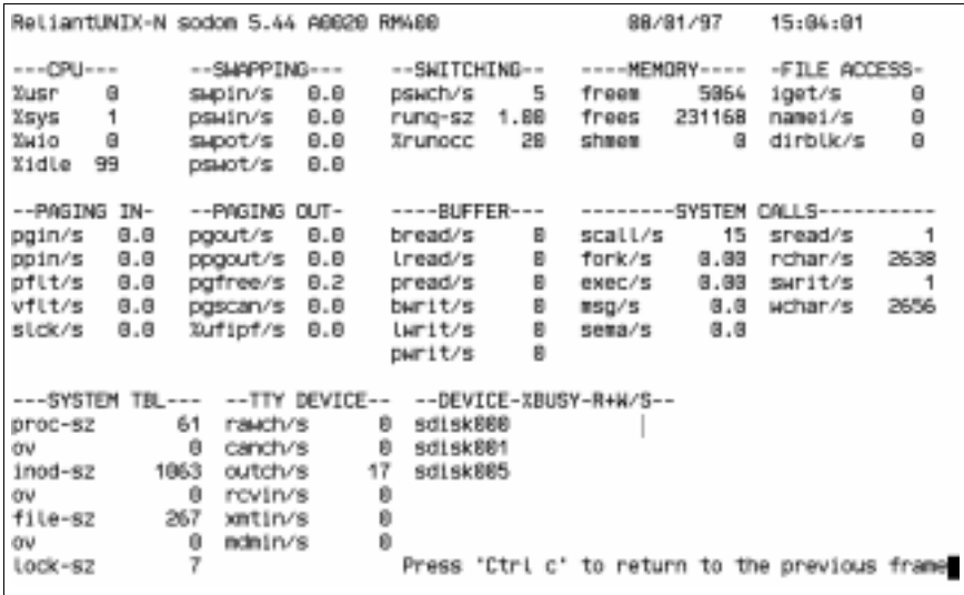
Figure 9: System activity reporting with sysadm (example)
