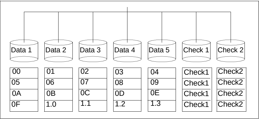
Figure 12: RAID level 2
