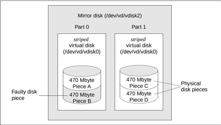
Figure 6: Faulty mirror disk design
