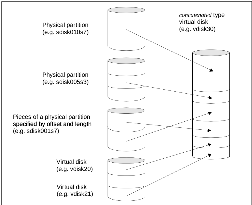
Figure 2: Composition of a concatenated type virtual disk
