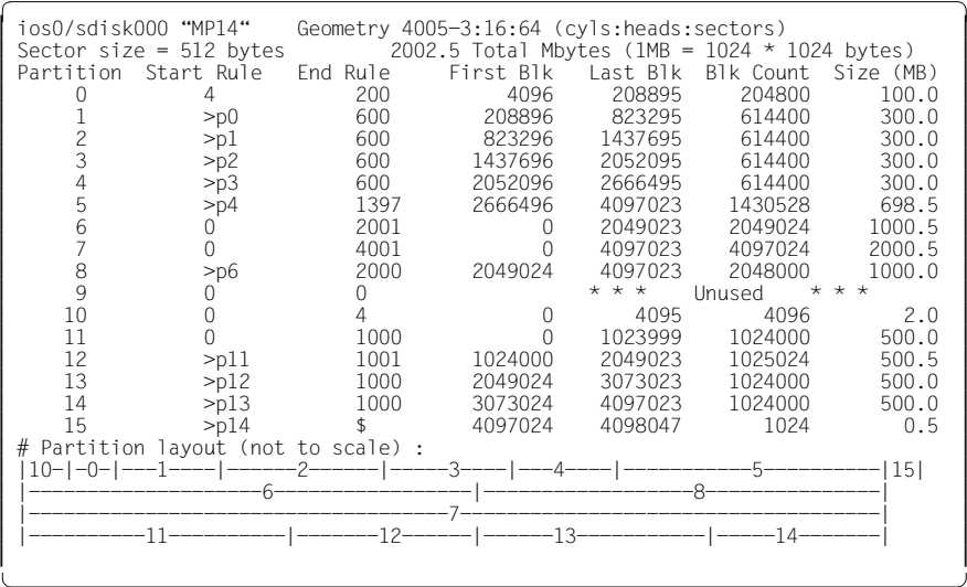
Figure 10: Screen output of dkpart
