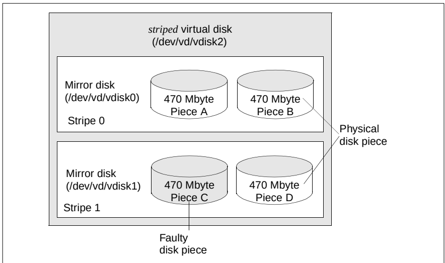
Figure 7: Correct design of a mirror disk
