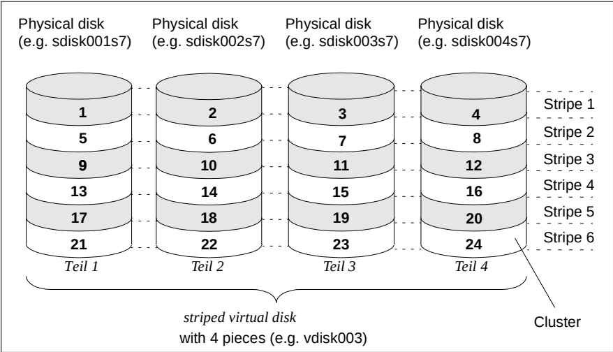
Figure 3: Structure of a striped virtual disk
