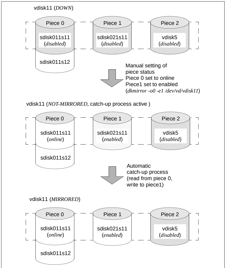
Figure 9: Behavior of a mirror disk when initializing the status of its pieces
