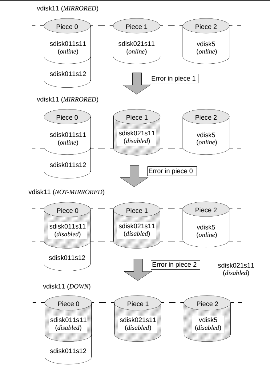
Figure 8: Behavior of a mirror disk in the event of errors in individual pieces
