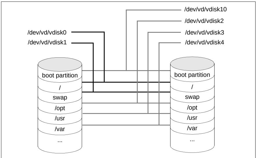
Figure 11: Sample configuration of a root mirror disk
