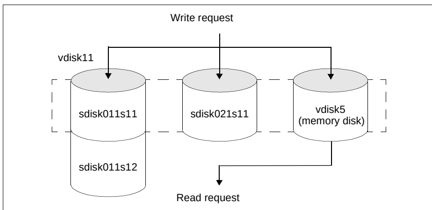
Figure 5: Writing to and reading from a mirror disk
