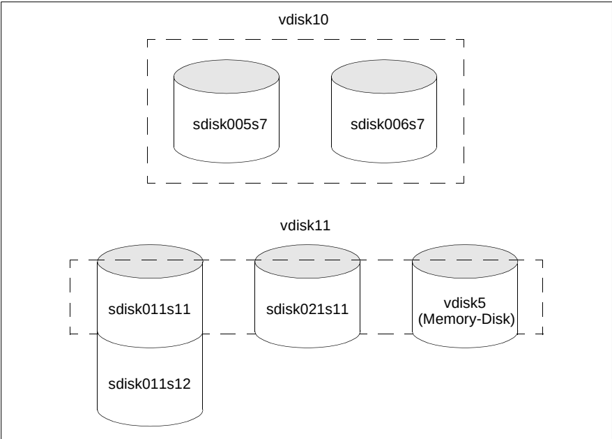
Figure 4: Structure of mirror disks
