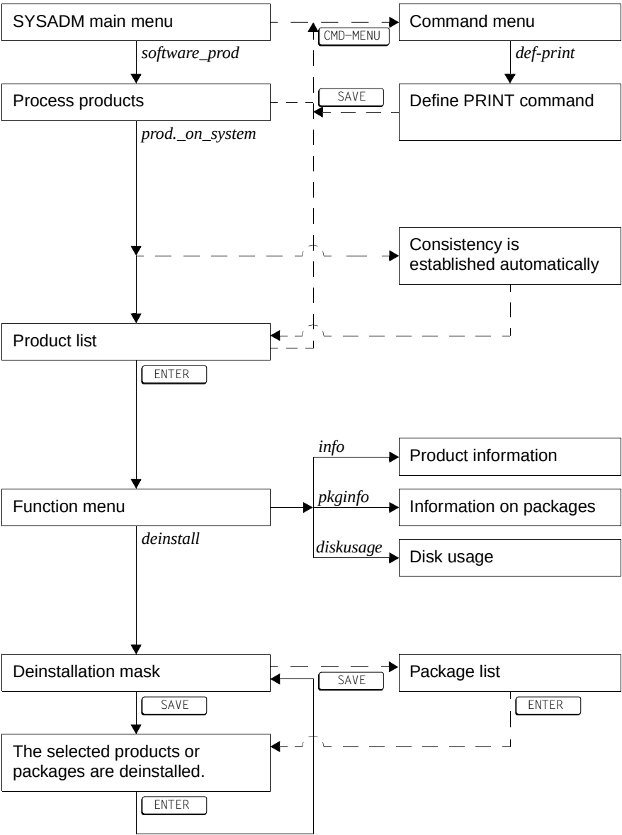
Figure 4: Overview of SYSADM – software_prod – products_on_system
