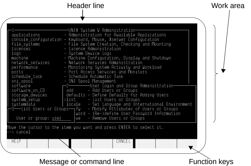
Figure 1: Layout of the SYSADM screen
