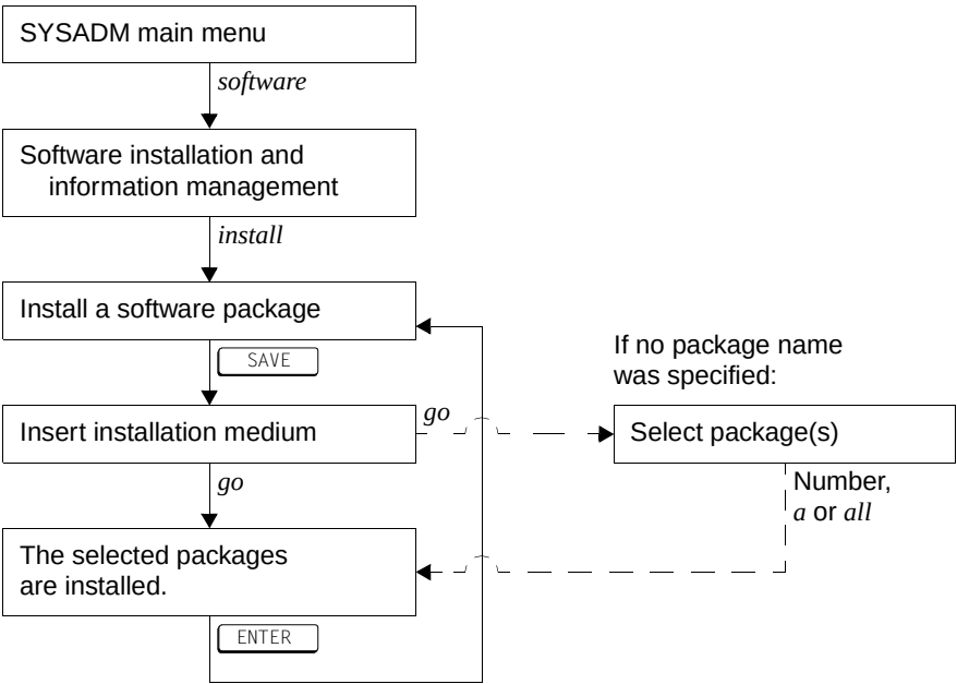
Figure 5: Overview of SYSADM – software – install
