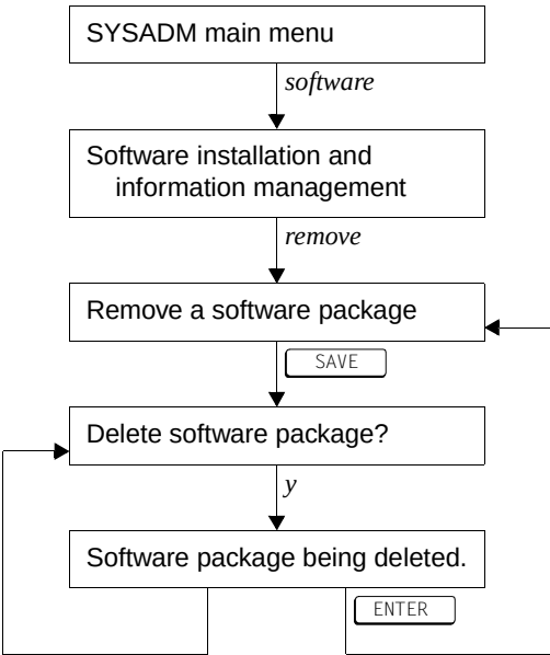
Figure 6: Overview of SYSADM – software – remove
