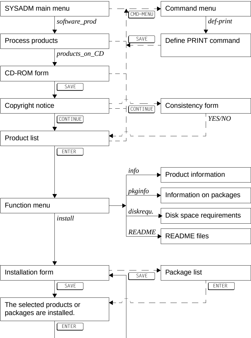
Figure 3: Overview of SYSADM – software_prod – products_on_CD
