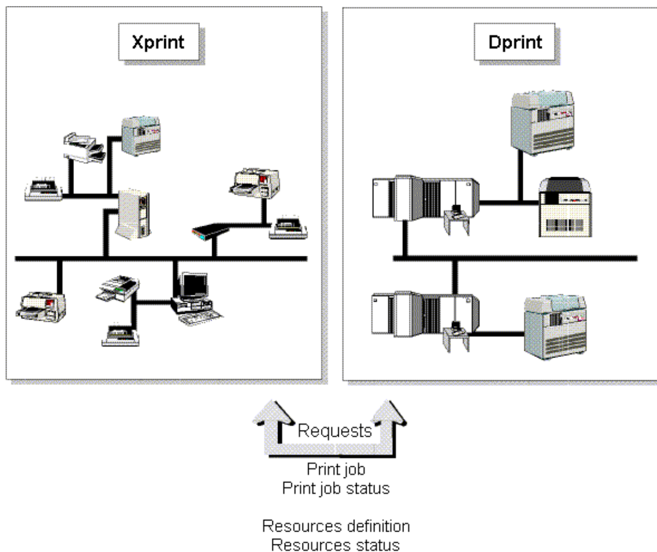
Figure 16: Gateway connection to DPRINT spoolers
