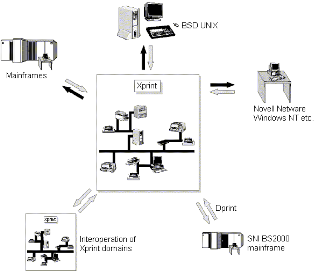
Figure 12: Interoperation with other spooler systems
