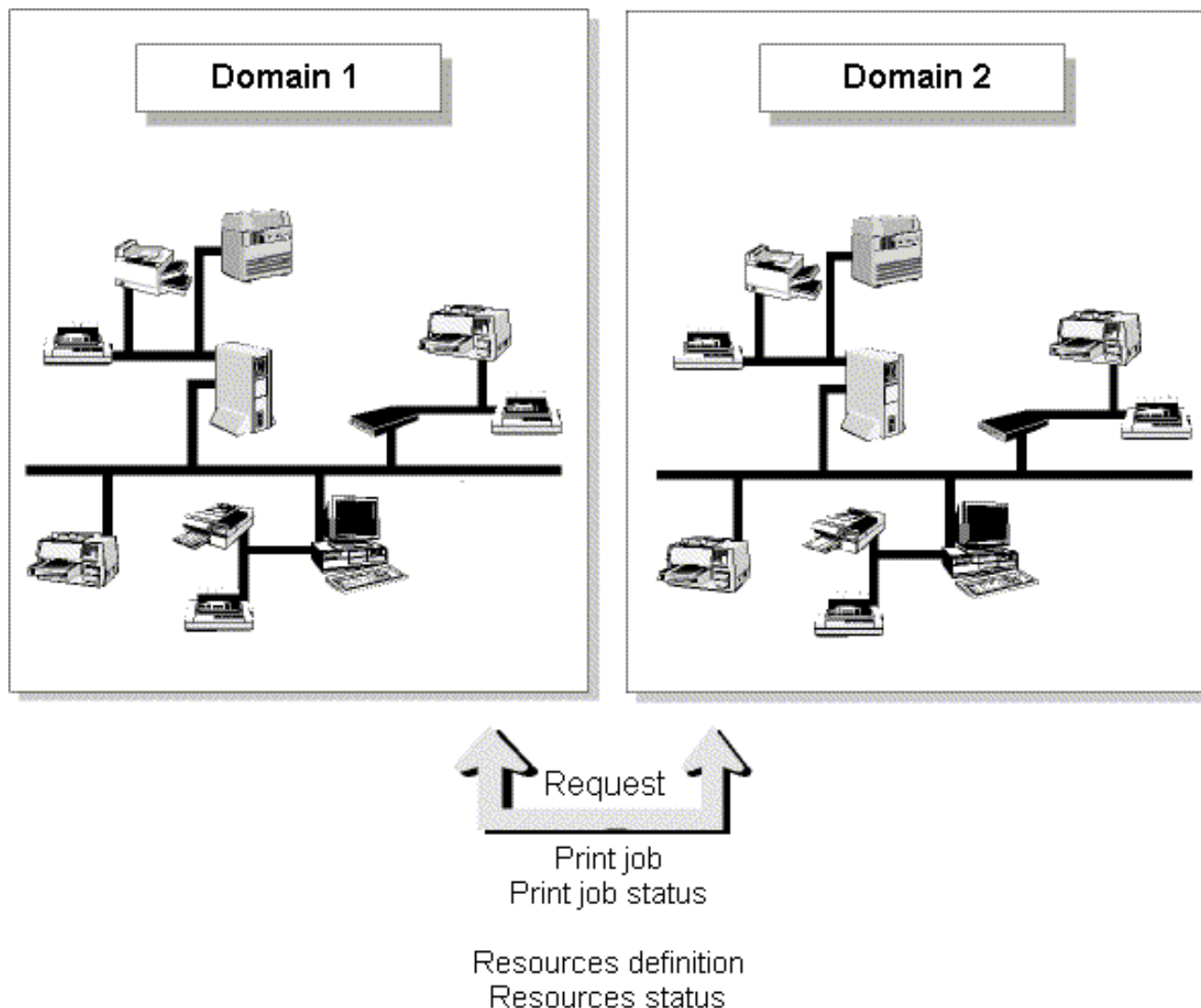
Figure 15: Gateway connection to another printer domain
