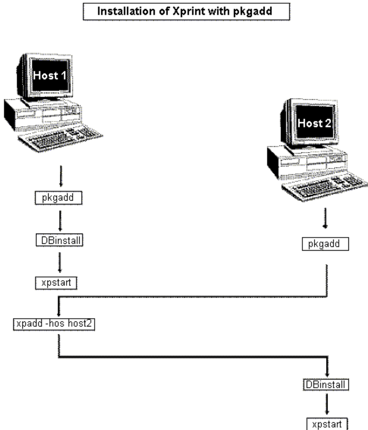
Figure 18: Installation process (Reliant UNIX users)
