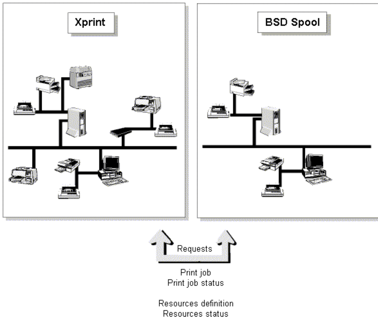
Figure 14: Structure of a gateway connection
