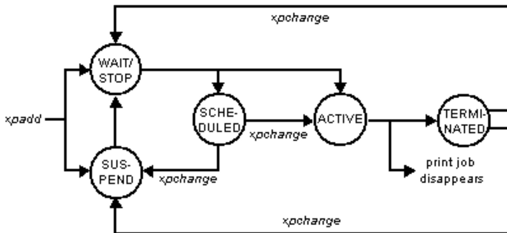
Figure 8: States of print jobs
