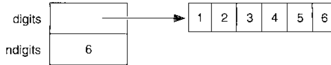
Figure 2-4 A diagram of the BigInt data structure for the number 654321
