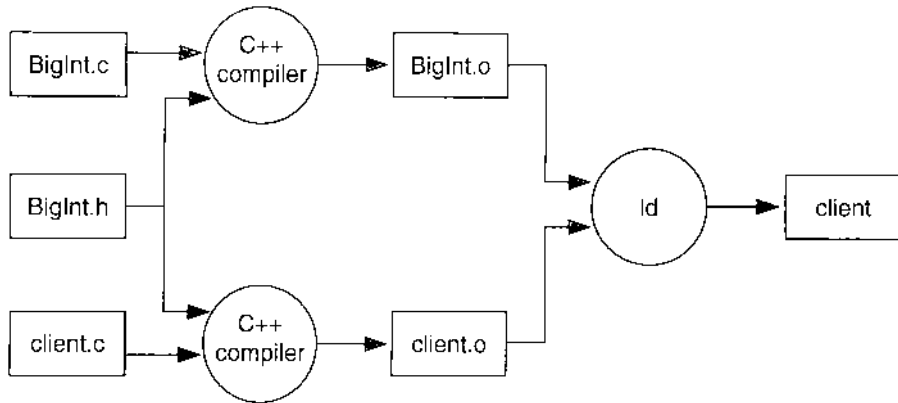
Figure 2-3 Combining the specification ( BigInt.h ) and implementation ( BigInt.c ) of an abstract data type ( BigInt ) with the source code of a client program ( client.c ) to produce an executable program ( client ).
