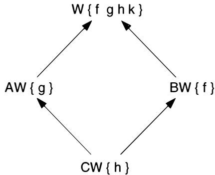
Figure 1-1 A directed acyclic graph
