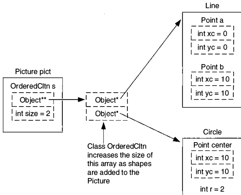
Figure 2-8 The data structure of a simple picture. Instances of OOPS library classes are shown as dashed rectangles.
