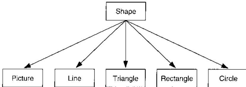
Figure 2-7 Improved organization of classes for a graphics package
