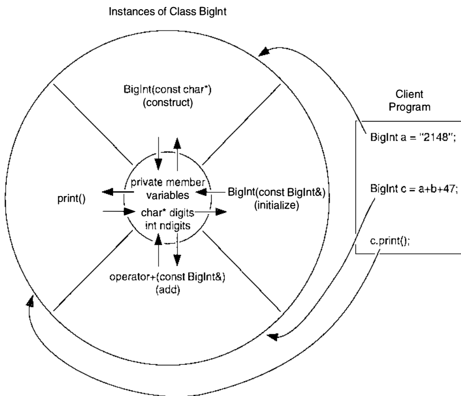
Figure 2-5 Client programs can access the private member variables of an instance of a class only by calling public member functions of the class
