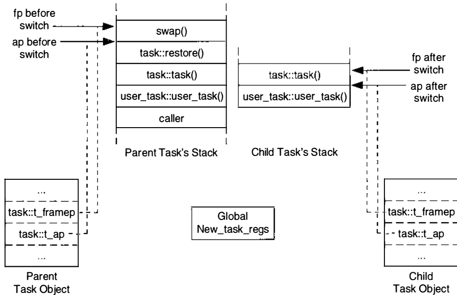
Figure 2-4 A task switch to a new child (DEDICATED)
