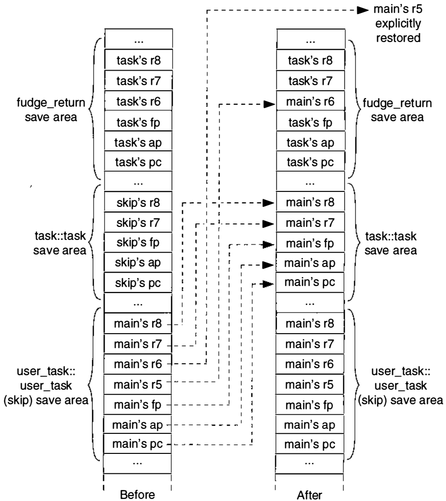
Figure 2-6 Fudging when user_task::user_task() uses more registers than task::task
