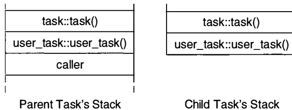
Figure 2-3 Creating a new task's stack
