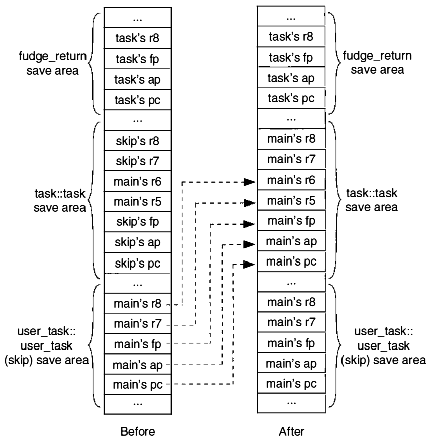
Figure 2-5 A 3B2 stack before and after fudging
