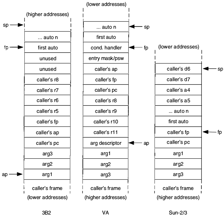
Figure 2-1 Stack frames on a 3B2, a VAX, and a sun-2/3 for a function taking 3 arguments and saving 4 registers
