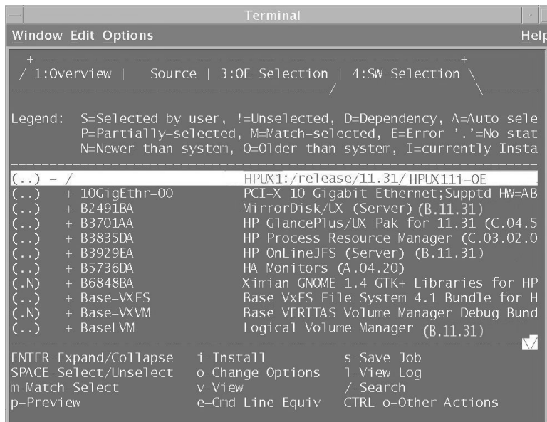
Figure 6-5 Software Selection Tab
