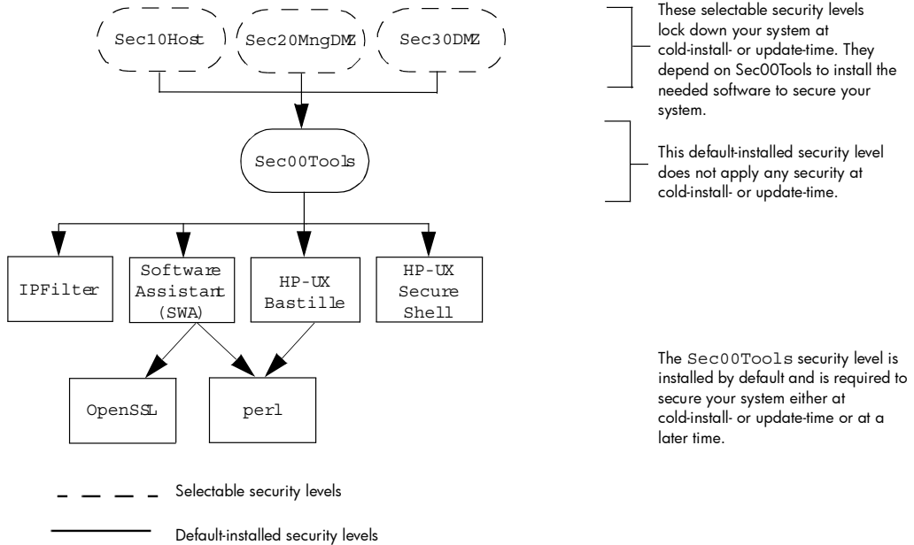
Figure 3-1 Install-time Security Software Dependencies
