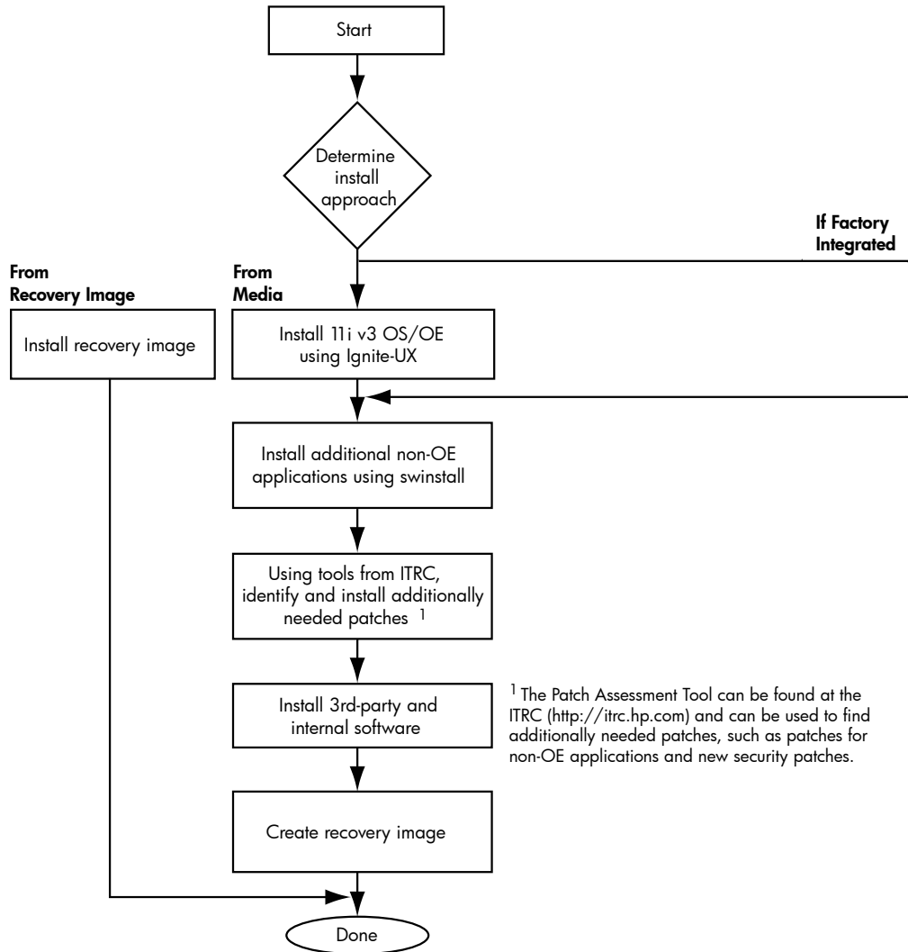
Figure 5-1 Cold-installing HP-UX 11i v3
