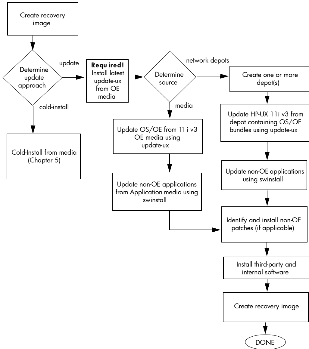
Figure 6-1 Updating to HP-UX 11i v3
