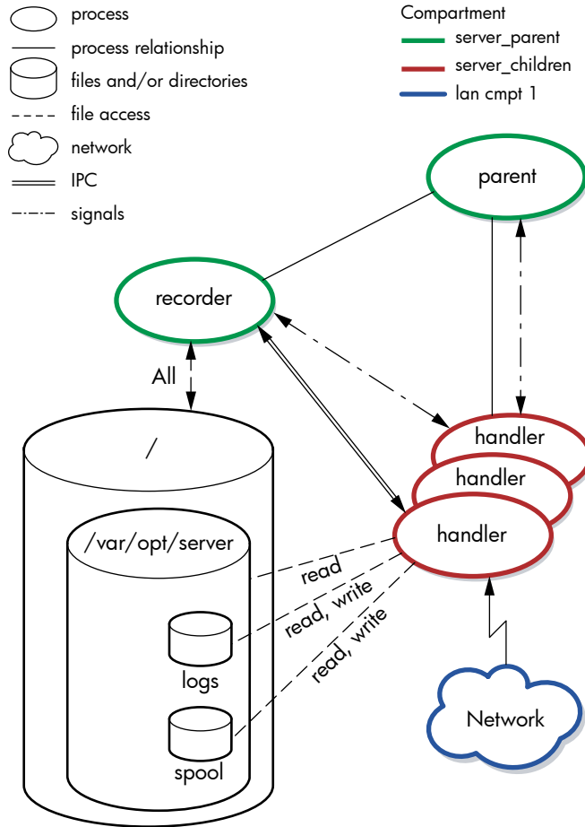
Figure 7-1 Compartment Architecture
