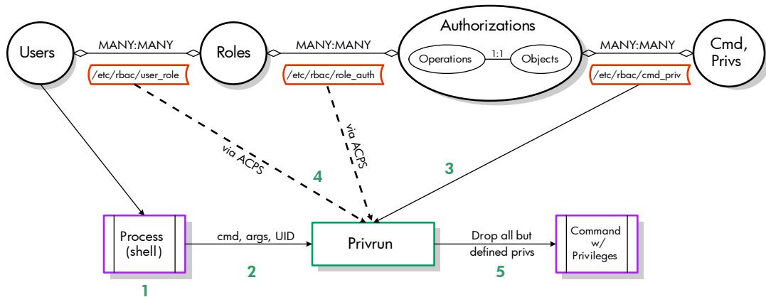
Figure 9-2 Example Operation After Invoking privrun
