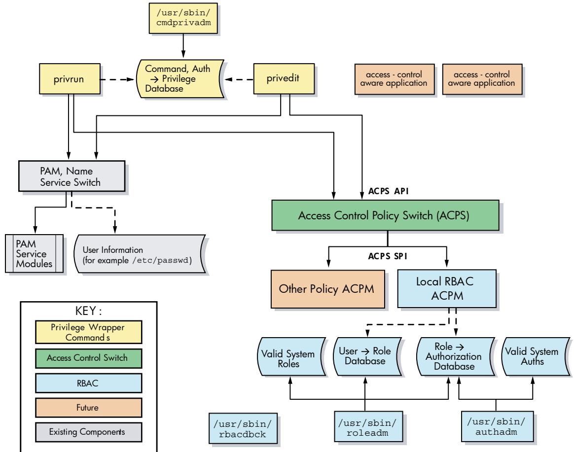
Figure 9-1 HP-UX RBAC Architecture
