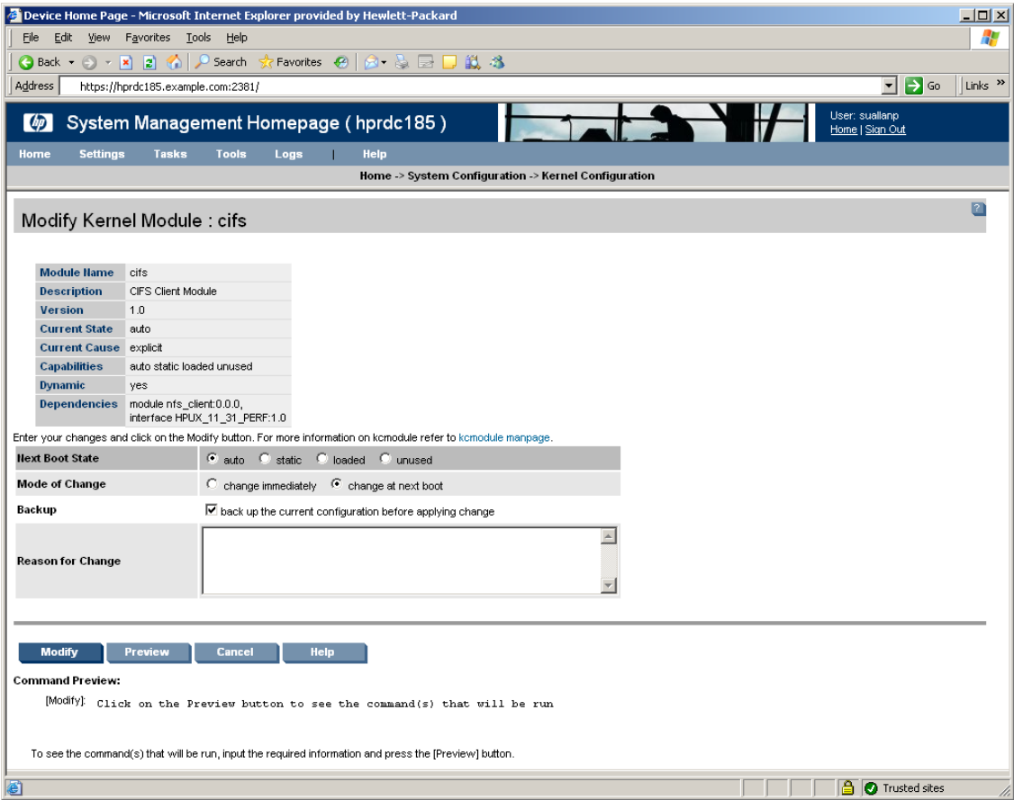
Figure 10-4 Modify Kernel Module
