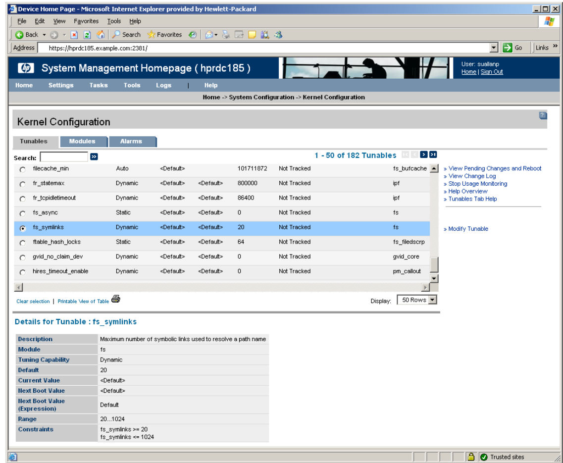
Figure 10-6 Kernel Configuration Tunable Details
