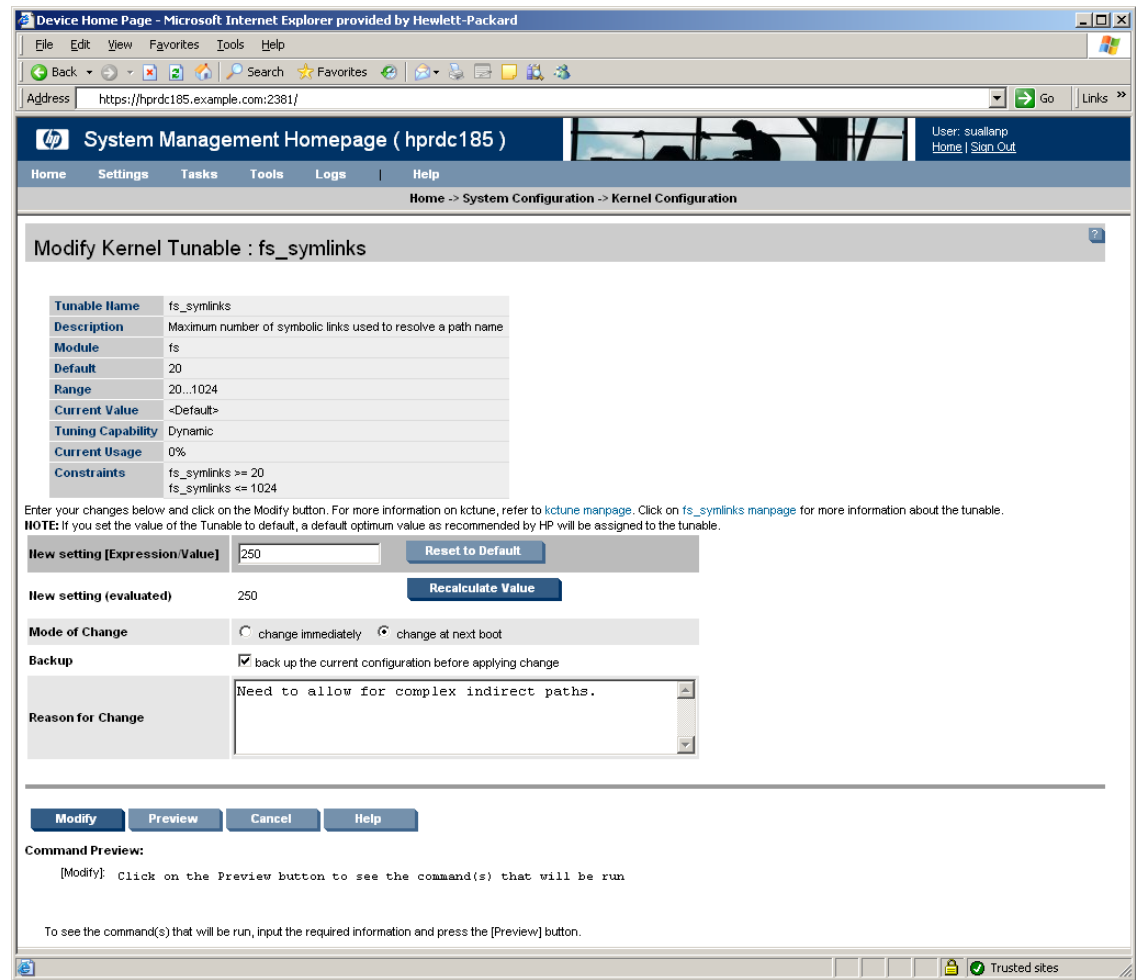
Figure 10-7 Modify Kernel Tunable
