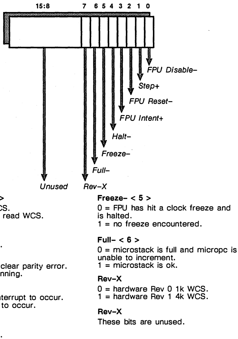
Figure A-3. The PEB Diagnostics Register
