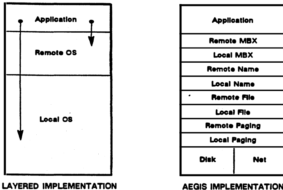
Figure 1-1. Styles of Local/Remote Implementations
