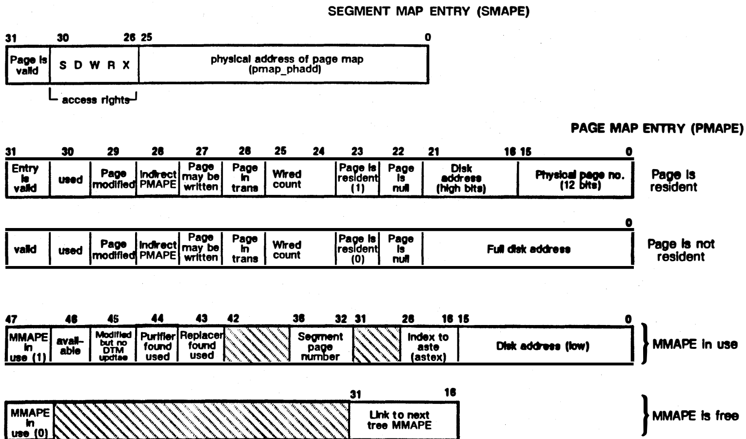
Figure 11-7. Physical Page Data Structures (Forward-Mapped)
