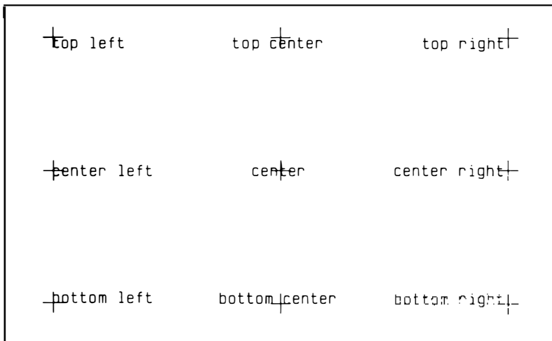
FIGURE 5-6 Text Alignment
