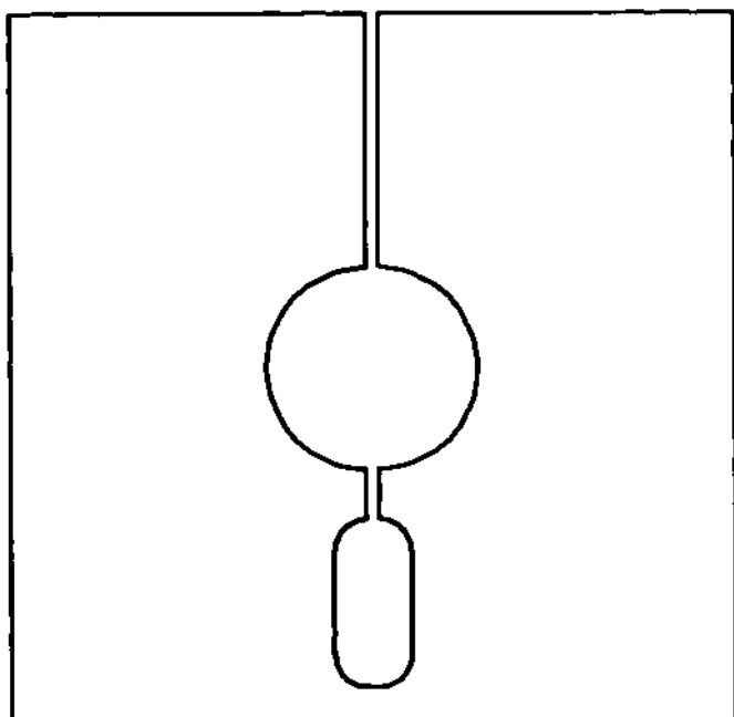
FIGURE 5-4 Polyline
