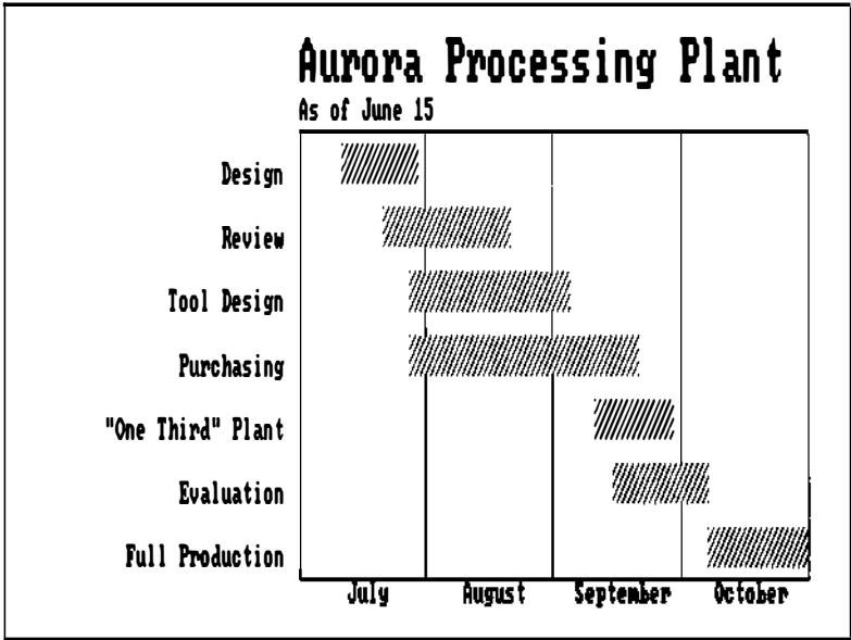
FIGURE 2-2 Gantt Chart
