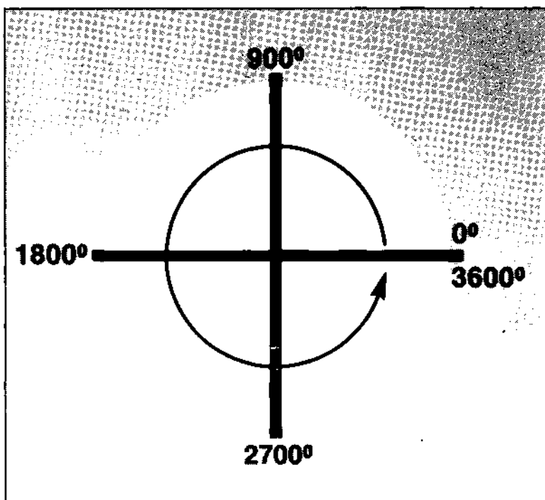
FIGURE 5-1 Angle Specification
