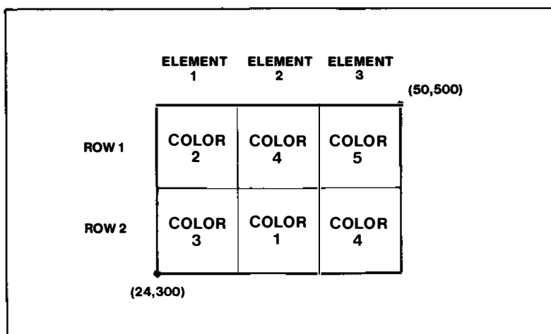
FIGURE 5-2 Cell Array
