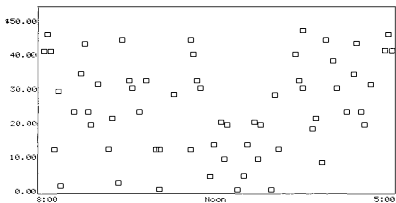
FIGURE 5-5 Polymarkers
