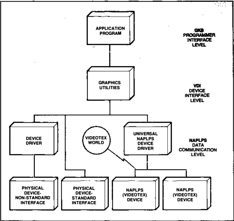
FIGURE 1-1 Graphics Standards
