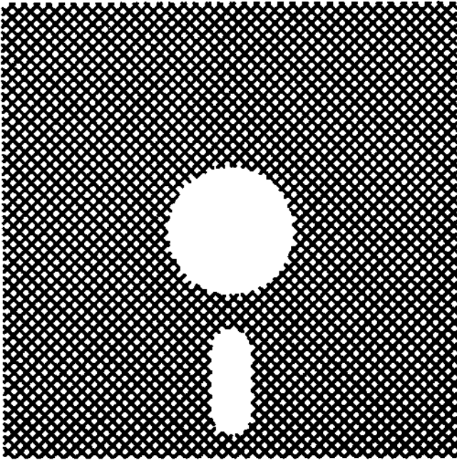
FIGURE 5-3 Filled Area
