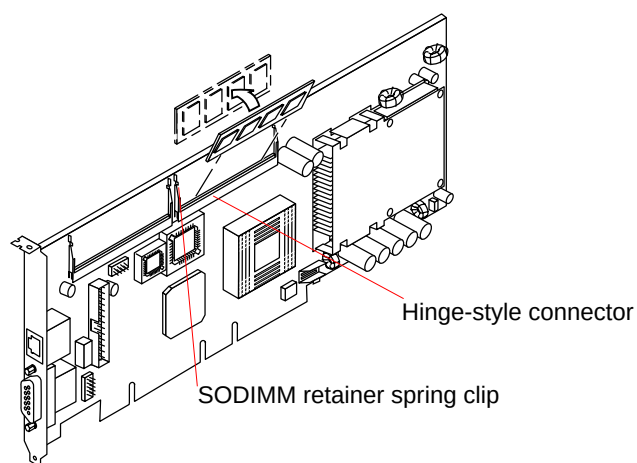
FIGURE 2 SODIMM Installation
