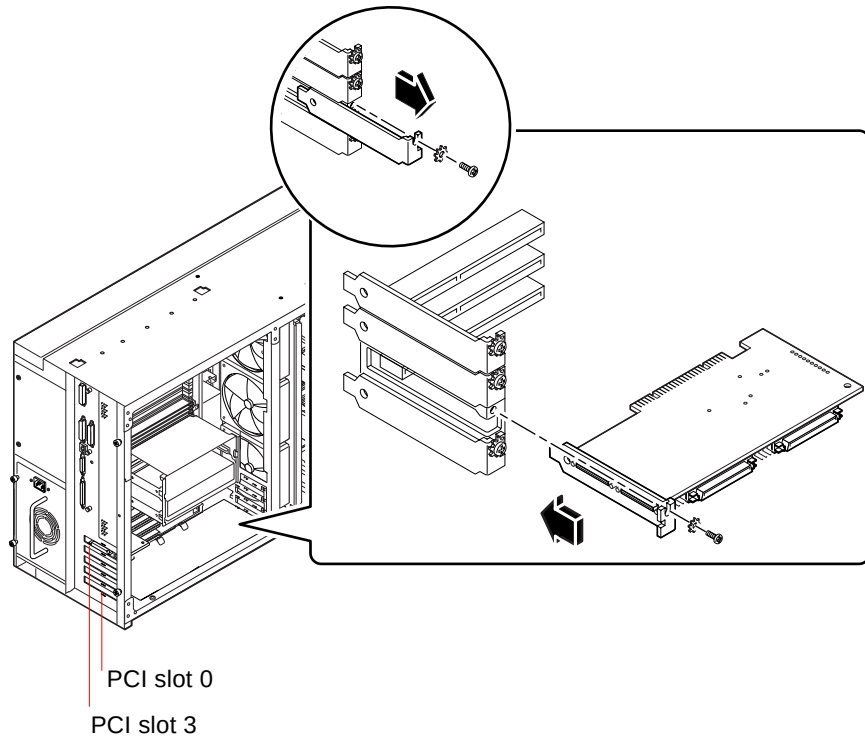
FIGURE 1-9 Sun Enterprise 250 System PCI Slots
