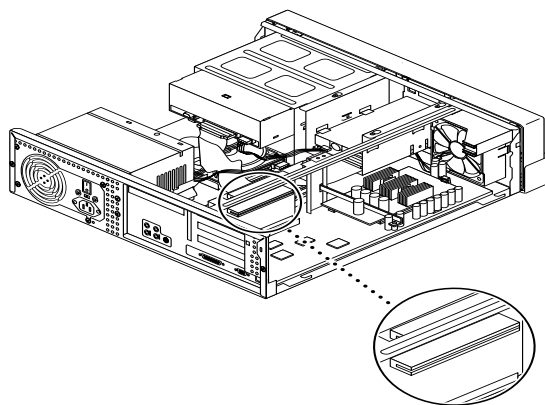
FIGURE 1 Ultra 5 PCI Slots
