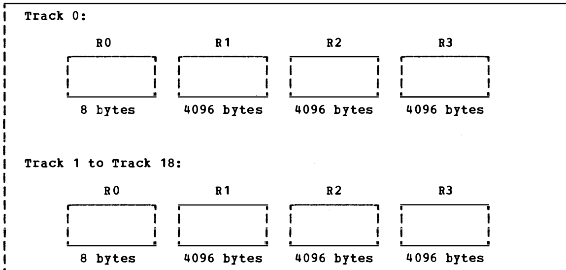
Figure 7. Format of 3330 Cylinders for Use by CP
