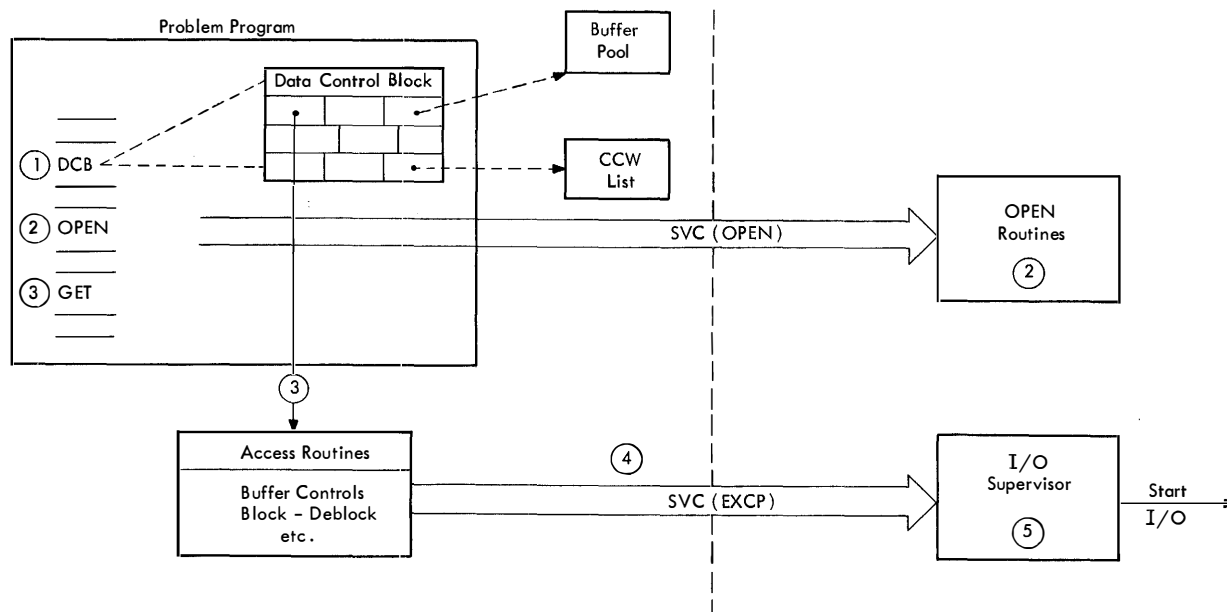
Figure 19. Actual Program Flow That Starts on Input/Output
