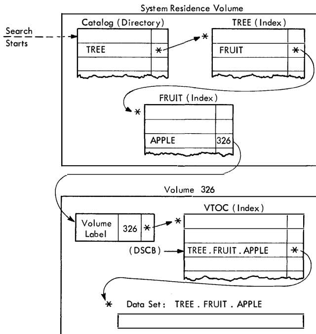
Figure 11. Catalog Search Procedure
