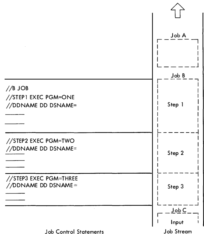
Figure 5. The Input Job Stream
