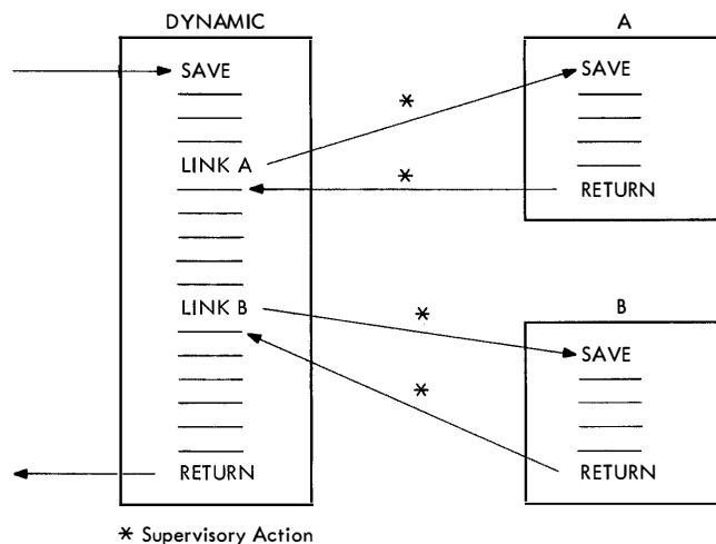
Figure 24. The LINK Operation
