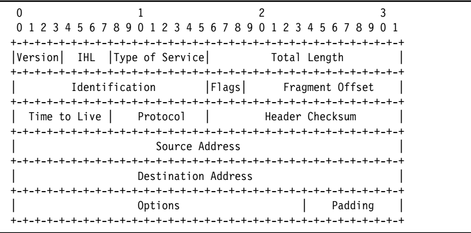
Example 2-1 IP header
