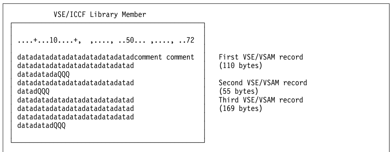
Figure 18. Illustration of Segmenting VSE/VSAM Records in VSE/ICCF Member
