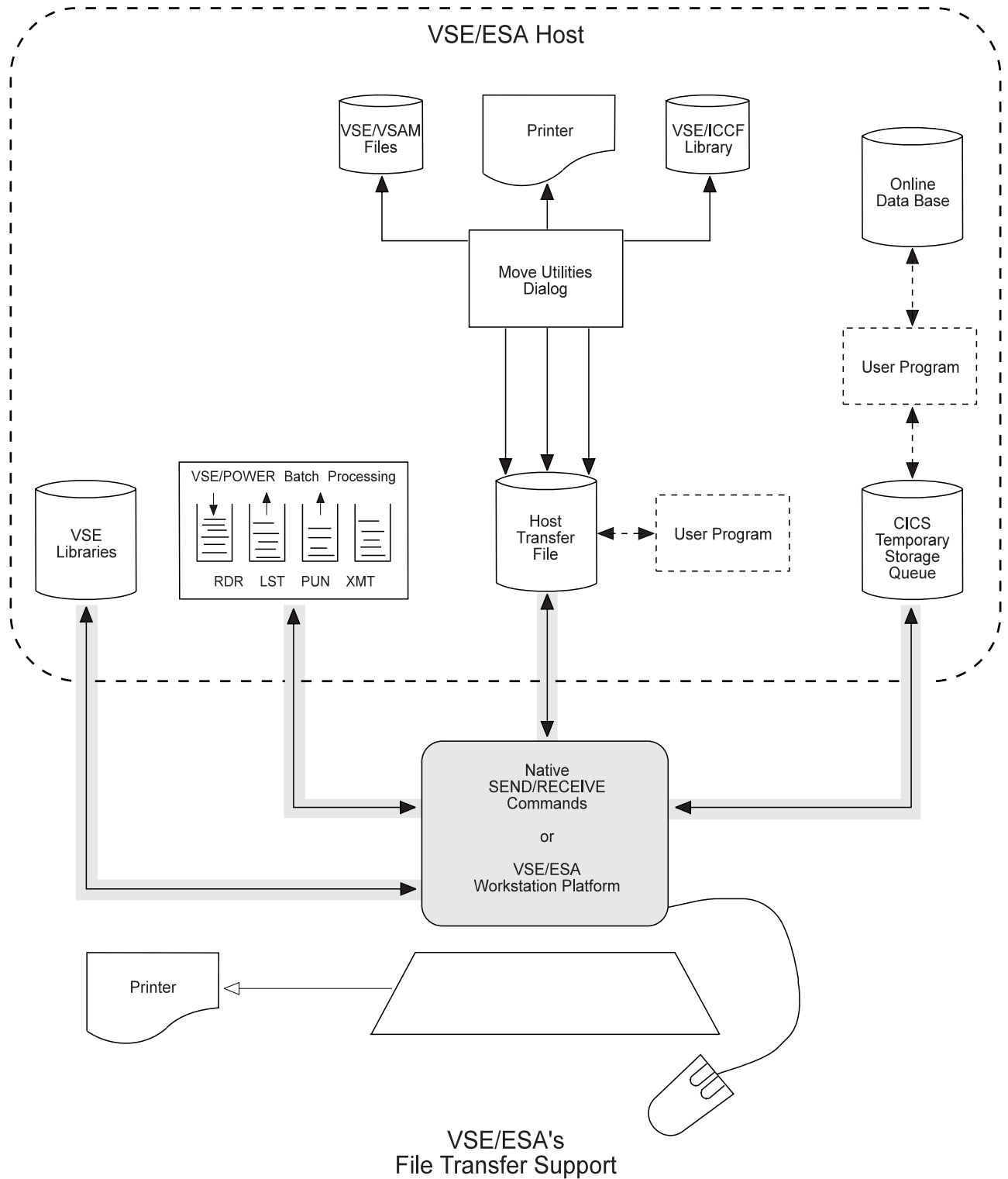
Figure 60. Data Paths of Data Conversion
