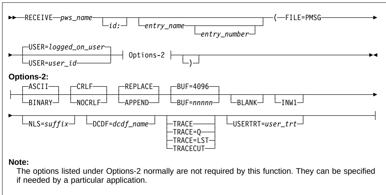
Figure 86. Receive Job Completion Messages - FILE=PMSG
