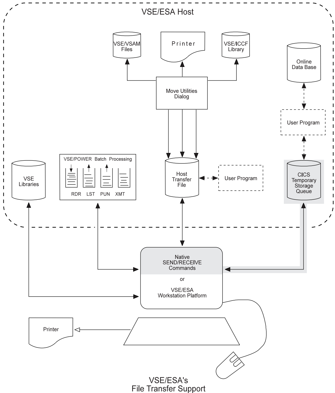
Figure 54. Transferring Data To and From CICS
