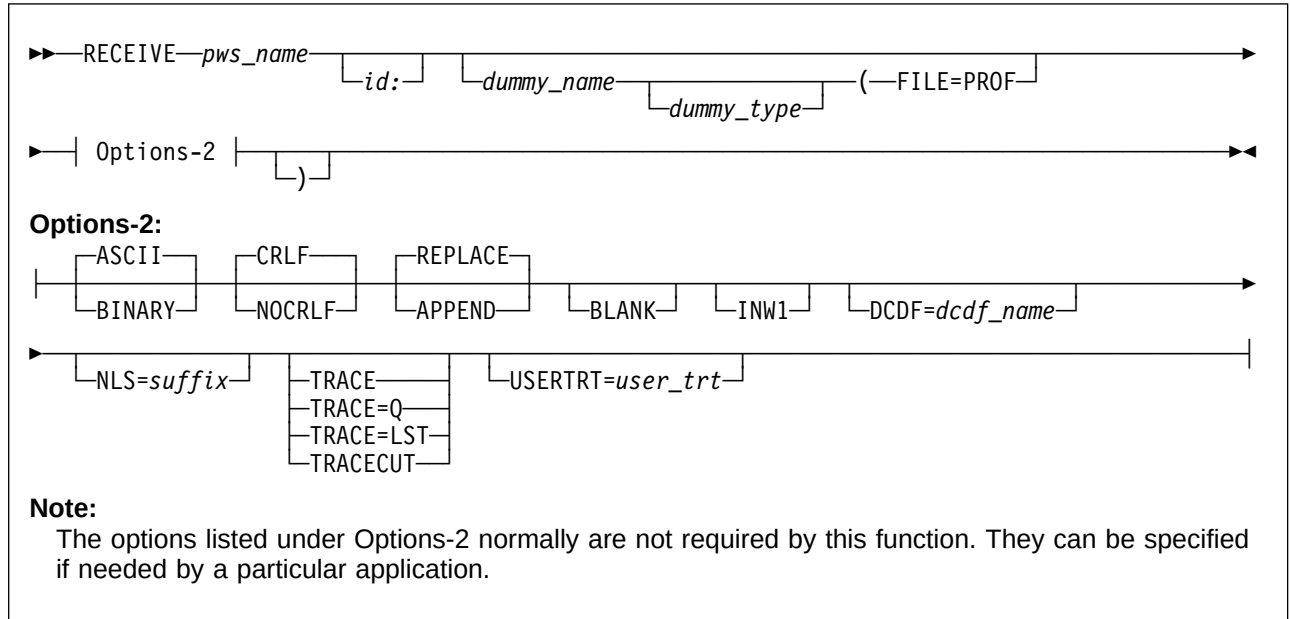
Figure 88. Service Function - Receive Host User Profile - FILE=PROF
