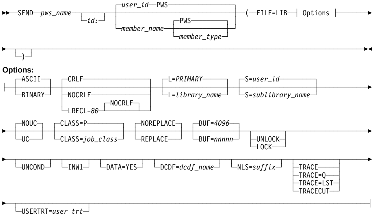
Figure 29 (Part 1 of 2). Send/Receive Workstation Files (fixed-format, string, phase) to/from a VSE Sublibrary
