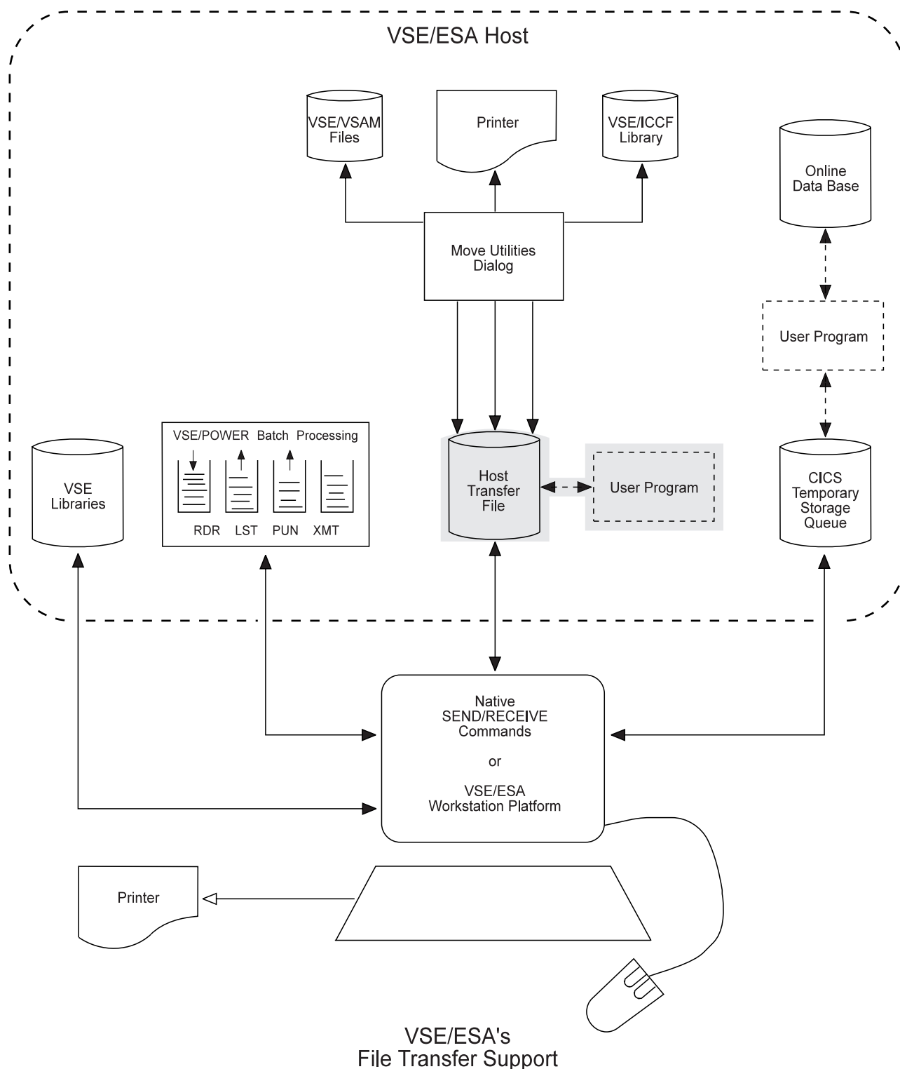
Figure 49. Data Paths of the Application Program Interface of the HTF
