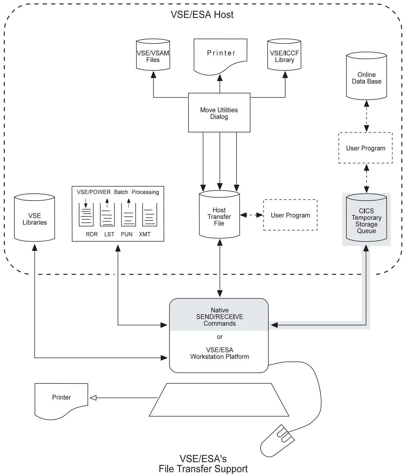
Figure 23. Transferring Data To and From CICS TS
