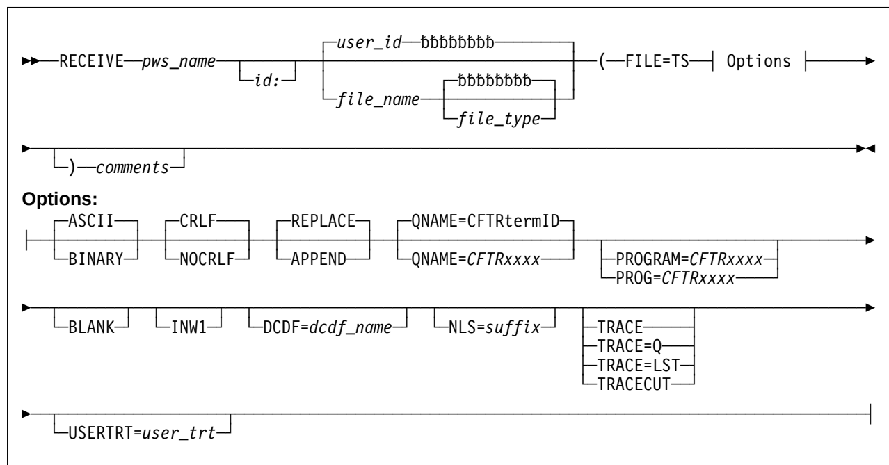
Figure 59 (Part 2 of 2). Send/Receive Workstation Files to/from CICS Temporary Storage Queues - FILE=TS
