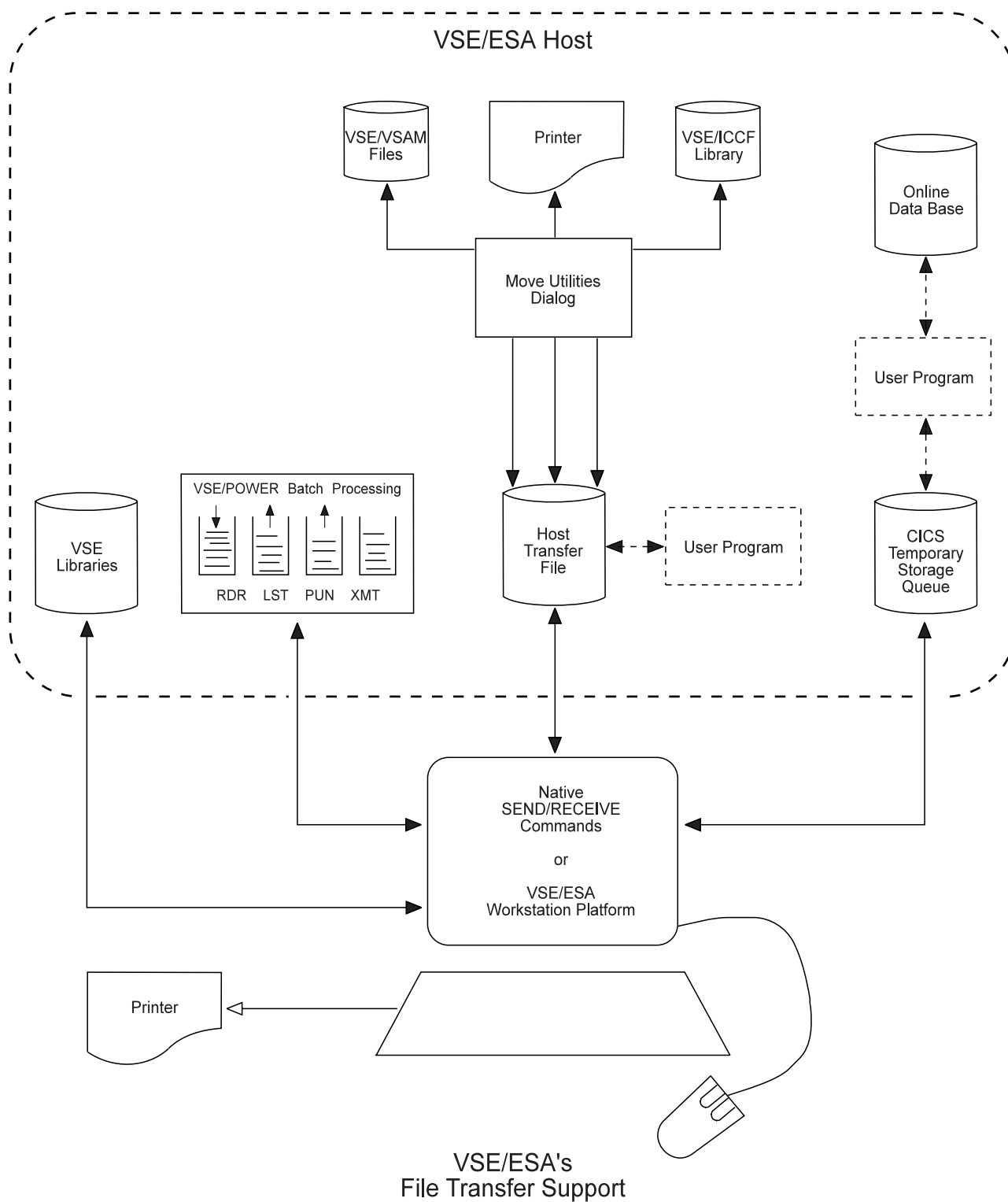
Figure 19. Major Data Paths of VSE/ESA's Workstation File Transfer Support
