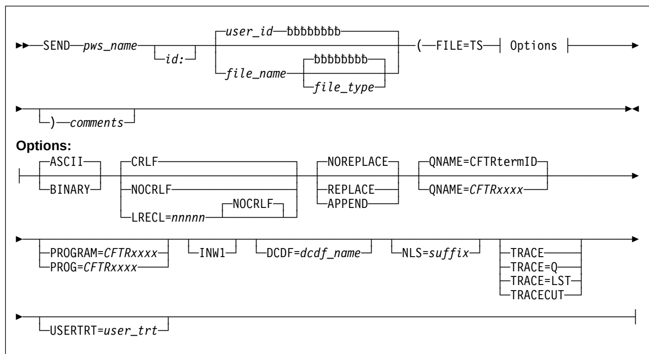
Figure 59 (Part 1 of 2). Send/Receive Workstation Files to/from CICS Temporary Storage Queues - FILE=TS
