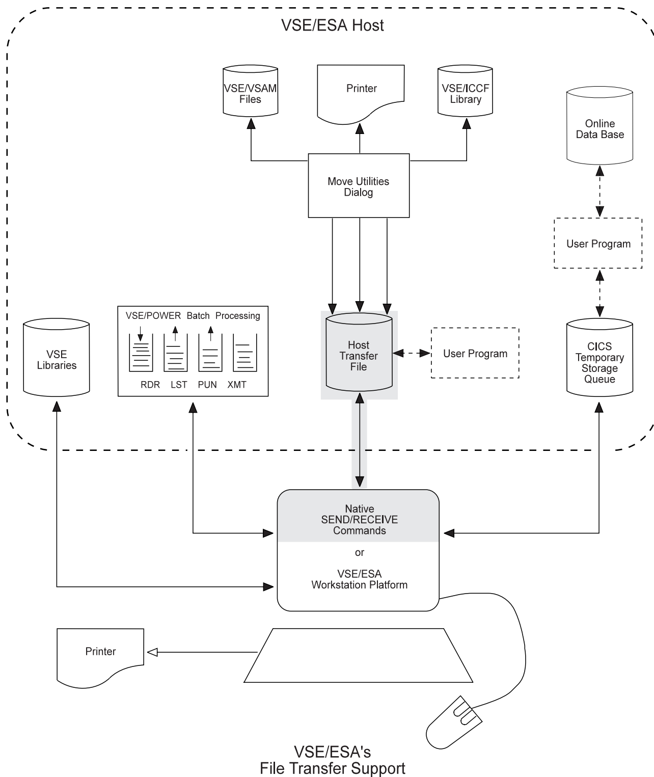
Figure 37. Transferring Data To and From the Host Transfer File
