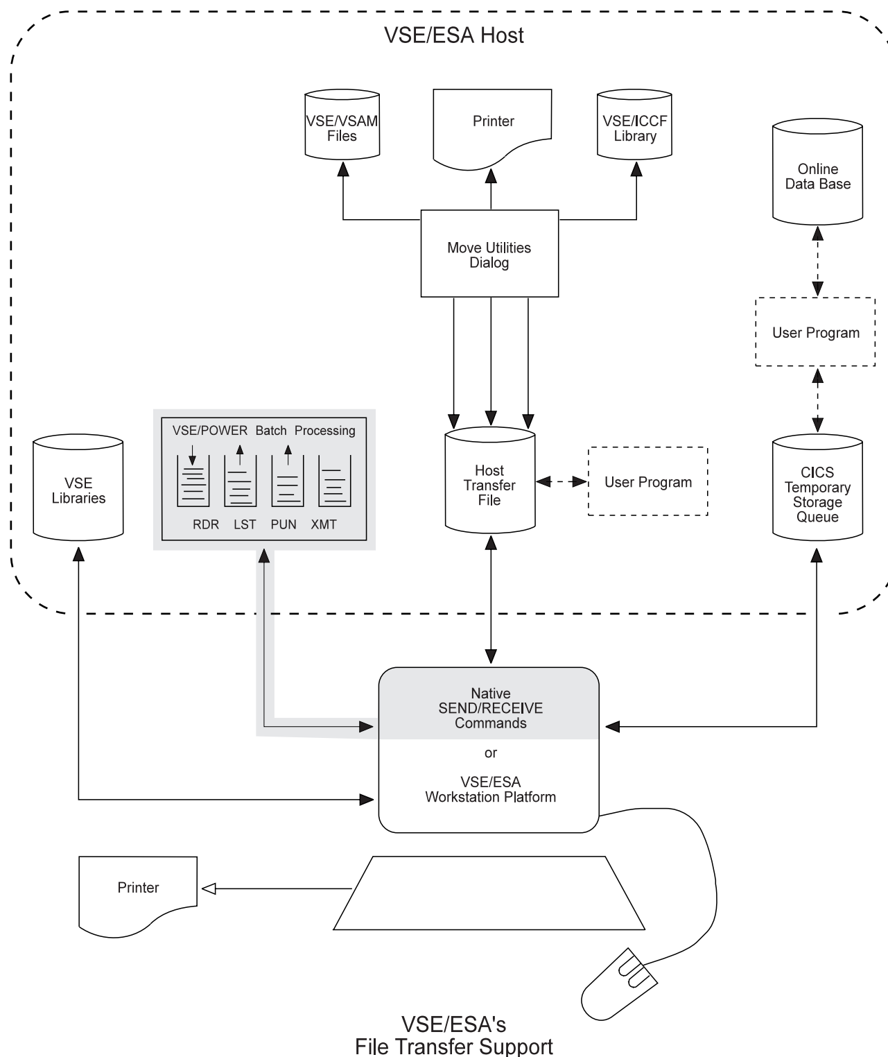
Figure 21. Transferring Data To and From VSE/POWER
