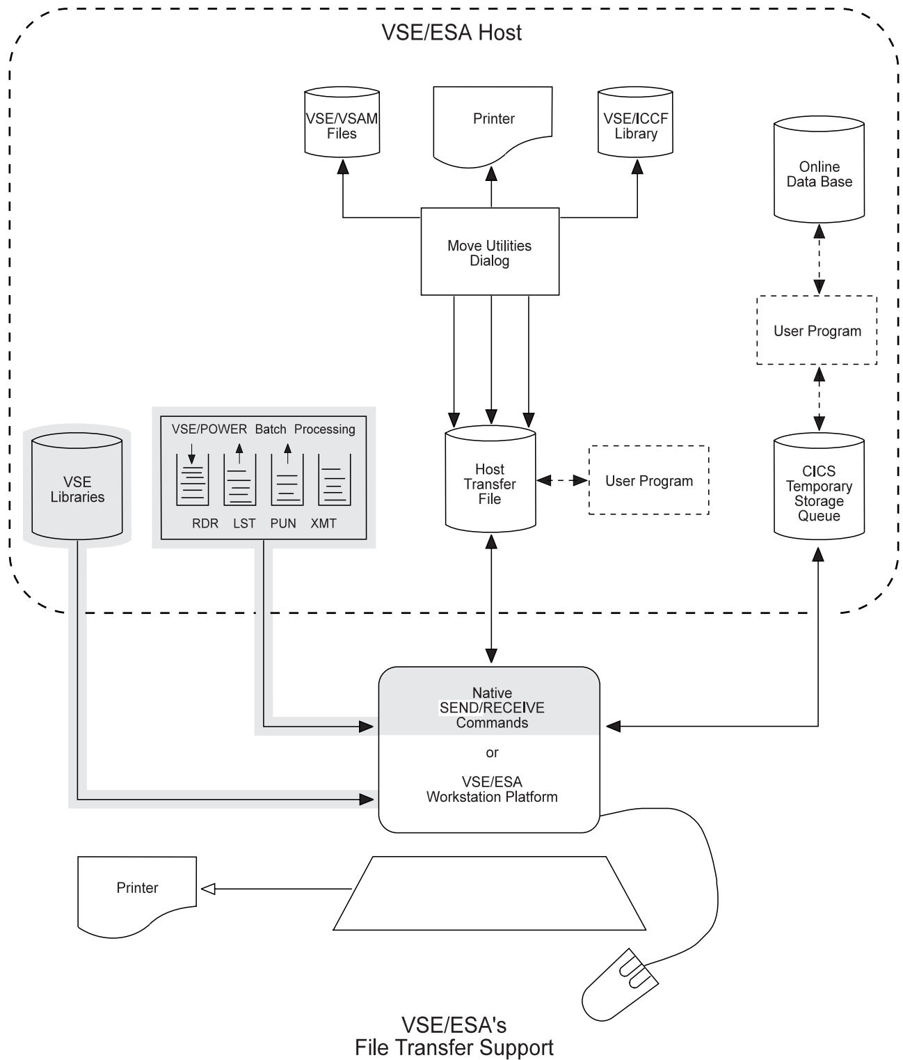
Figure 74. Data Paths of Service Functions
