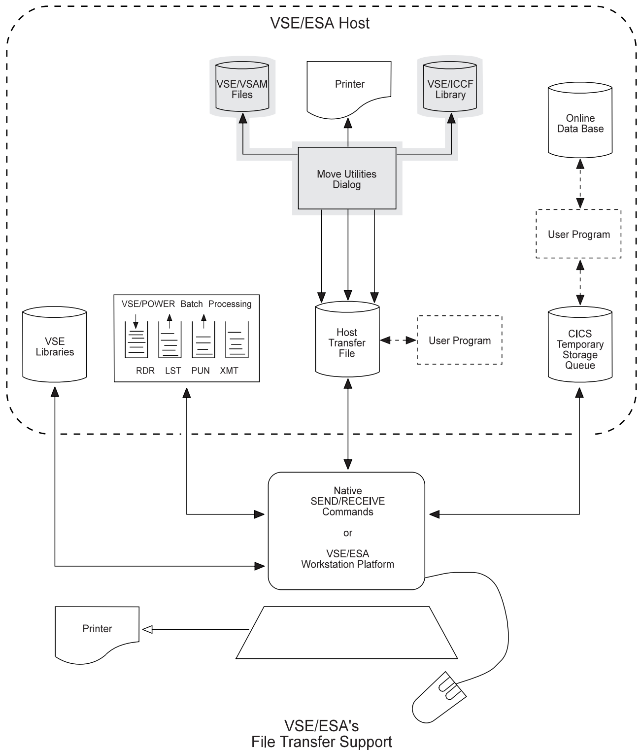
Figure 46. Data Paths of the User Exits of the Move Utilities
