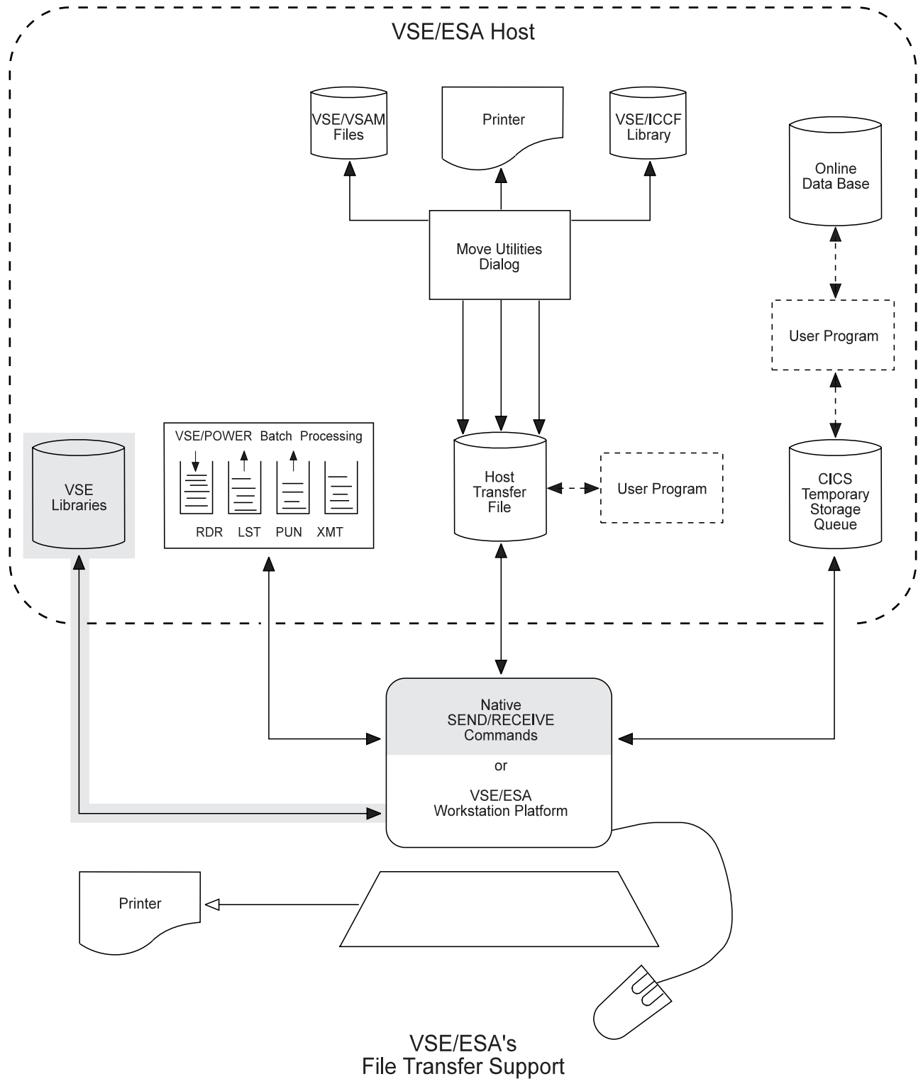
Figure 26. Transferring Data To and From the VSE Libraries
