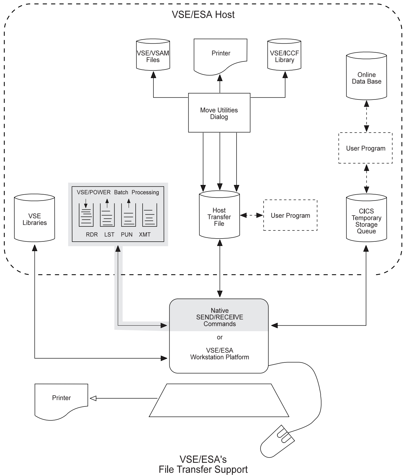
Figure 30. Transferring Data To and From VSE/POWER
