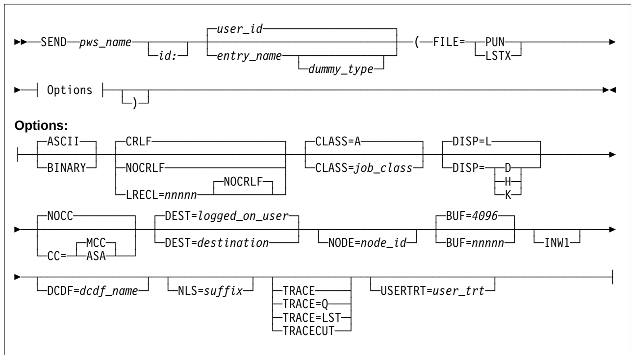
Figure 34. Send a Workstation File to the VSE/POWER PUN/LST Queue - FILE=PUN/LSTX
