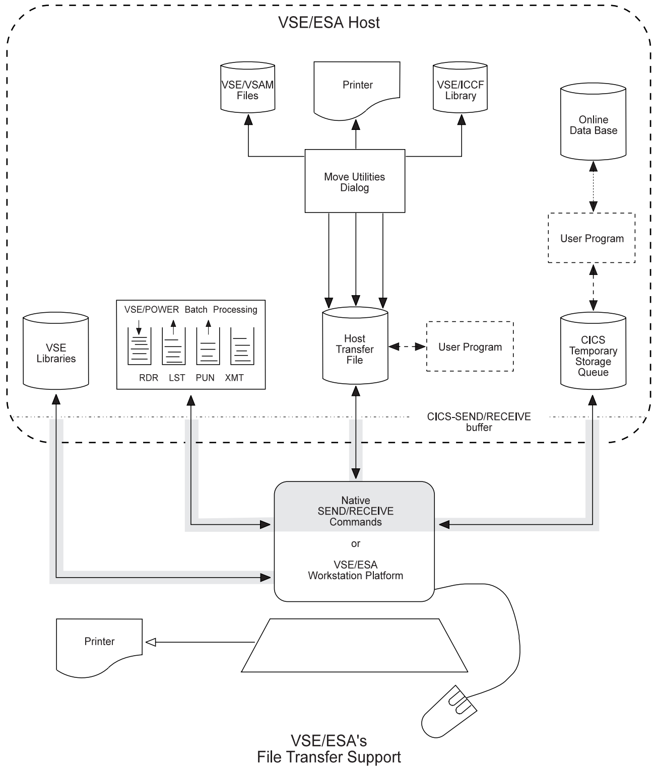
Figure 69. Data Paths of the File Transfer Trace
