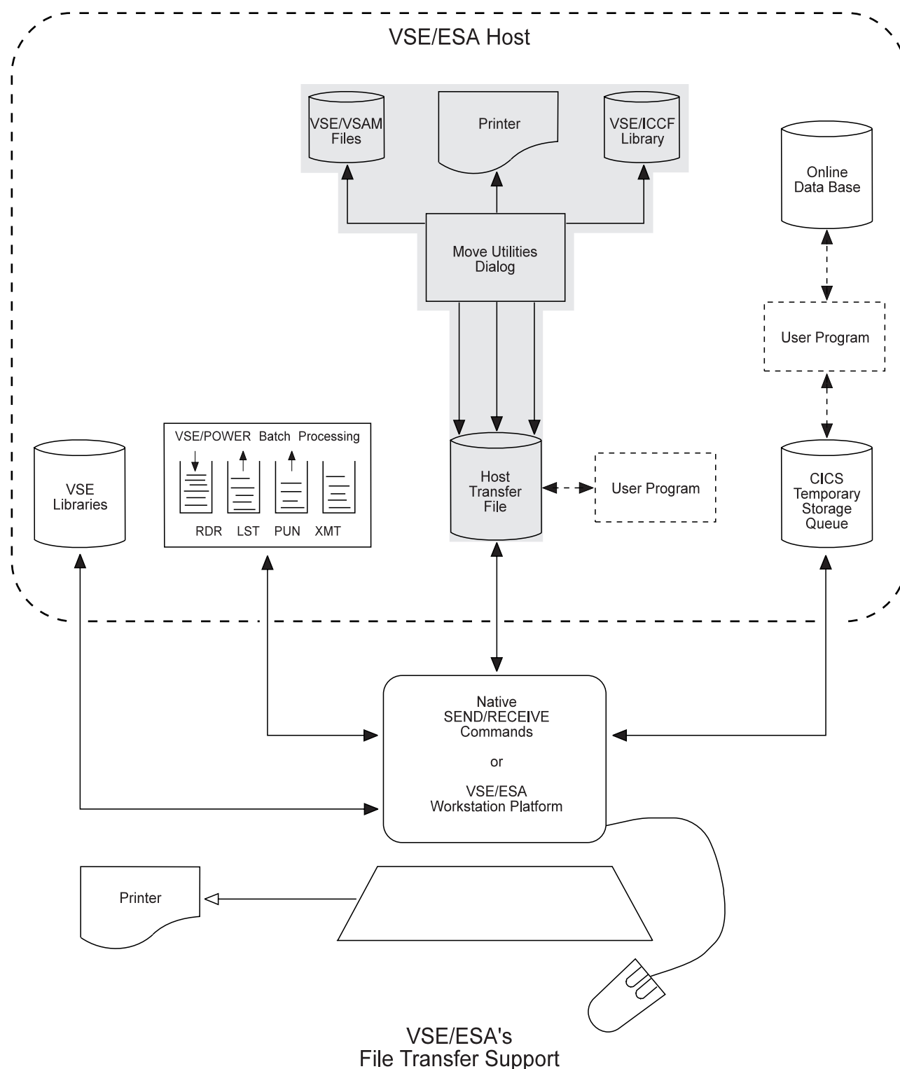
Figure 39. Data Paths of the Move Utilities
