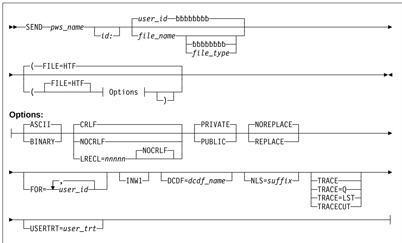
Figure 53 (Part 1 of 2). Send/Receive Workstation Files to/from the Host Transfer File - FILE=HTF
