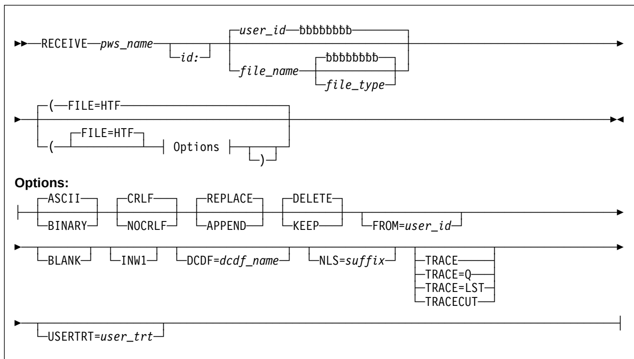
Figure 53 (Part 2 of 2). Send/Receive Workstation Files to/from the Host Transfer File - FILE=HTF
