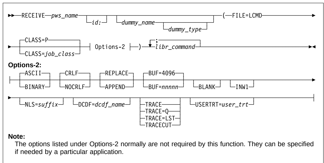
Figure 80. Send a Librarian Command for Execution to the Host - FILE=LCMD:
