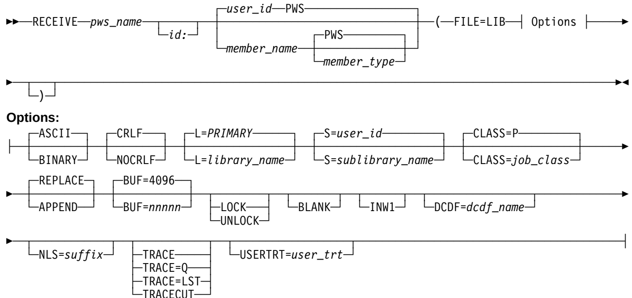
Figure 29 (Part 2 of 2). Send/Receive Workstation Files (fixed-format, string, phase) to/from a VSE Sublibrary
