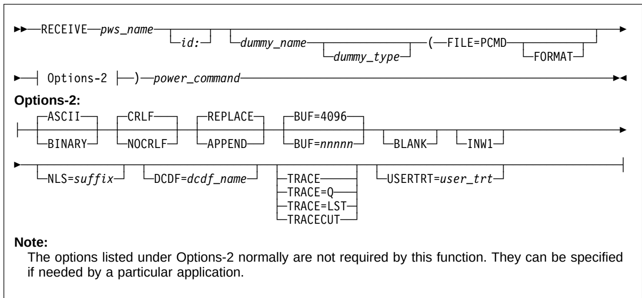
Figure 83. Send a VSE/POWER Command for Execution to the Host - FILE=PCMD
