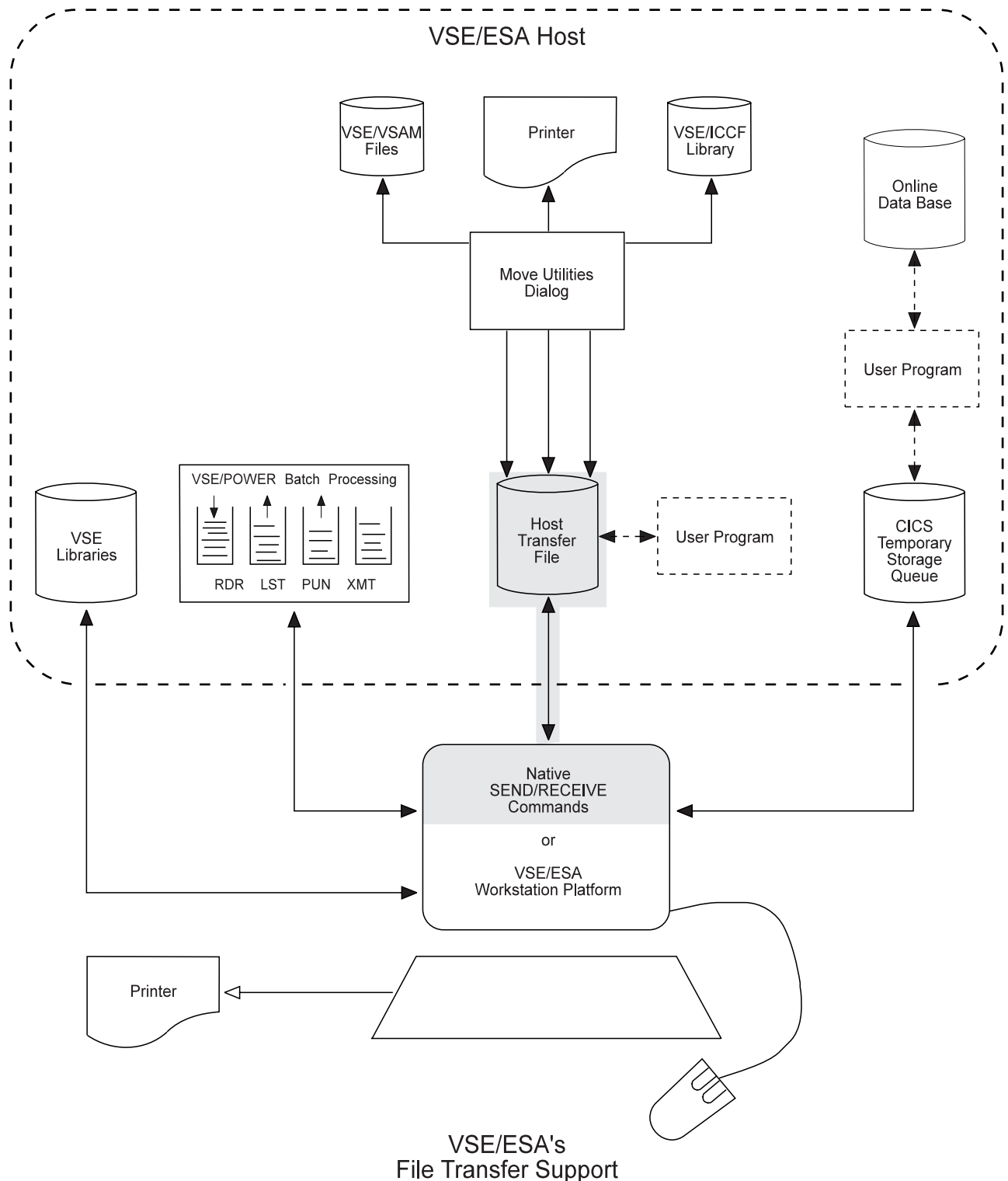
Figure 22. Transferring Data To and From the HTF
