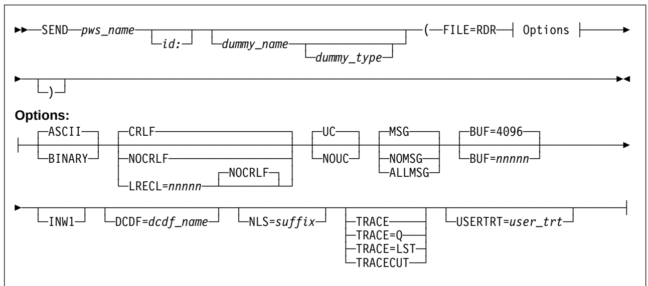
Figure 33. Send a Job to the VSE/POWER RDR Queue - FILE=RDR
