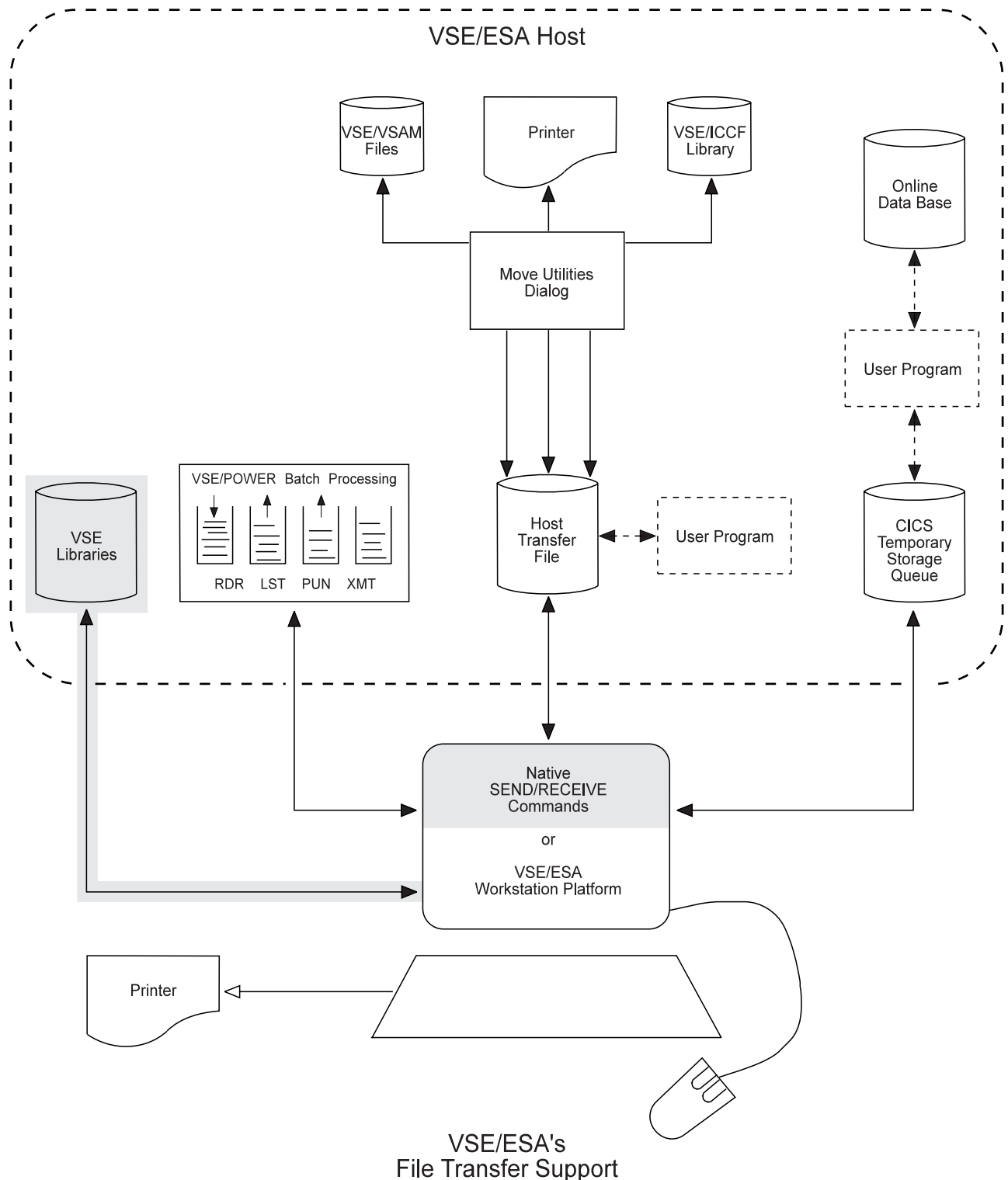
Figure 20. Transferring Data To and From VSE Libraries
