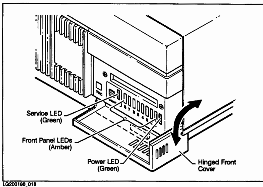
Figure 6-1. LED Array
