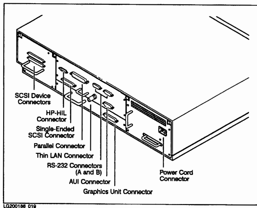
Figure 1-6. The Rear Panel of the System Unit
