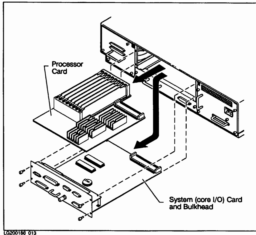
Figure 5-2. Processor Card Removal
