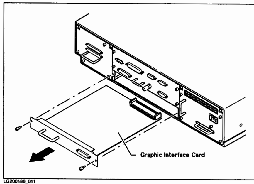
Figure 5-11. Graphics Card Replacement
