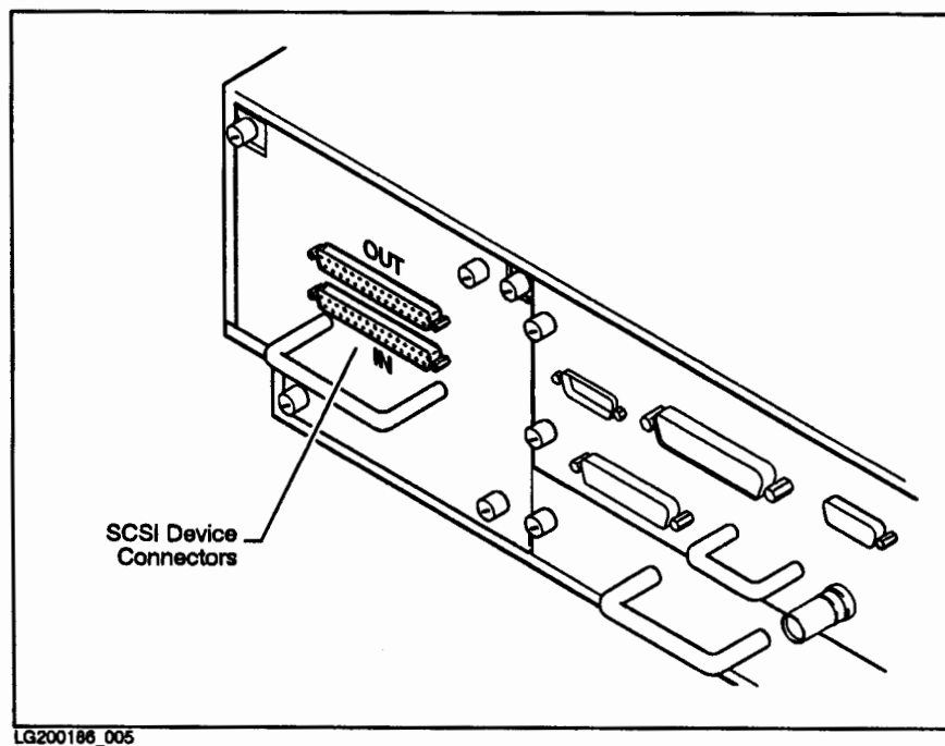
Figure 1-7. SCSI Connectors on the Disk Tray
