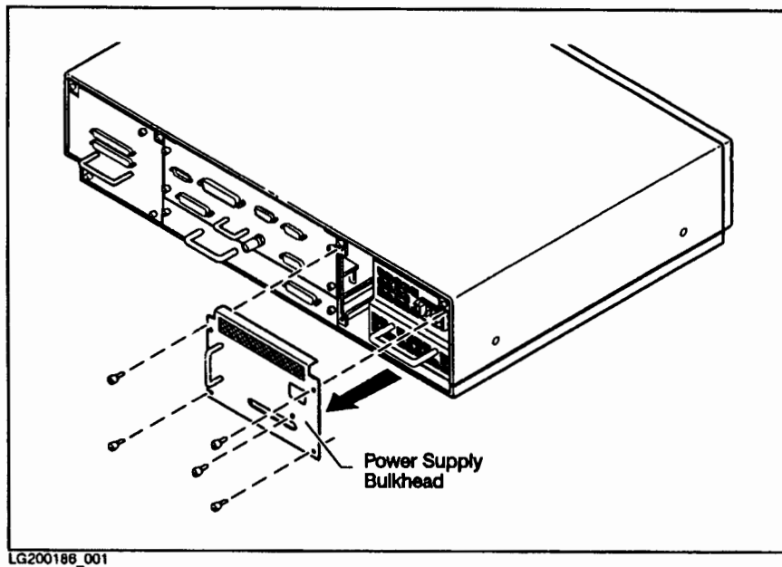
Figure 5-12. Power Supply Bulkhead Removal
