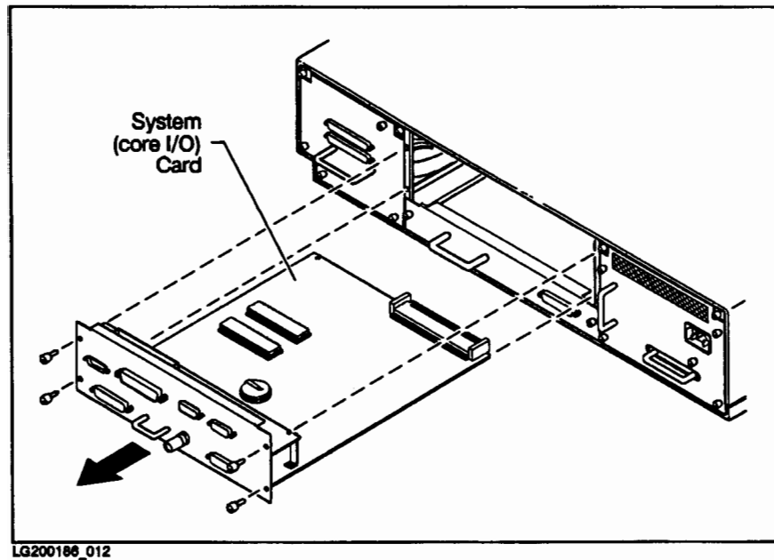
Figure 5-1. Core I/O Card Removal
