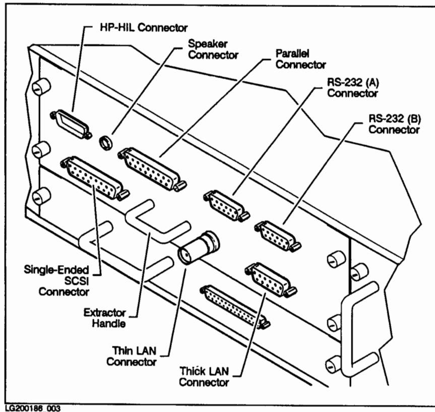
Figure 1-8. Connectors Mounted on the I/O Bulkhead
