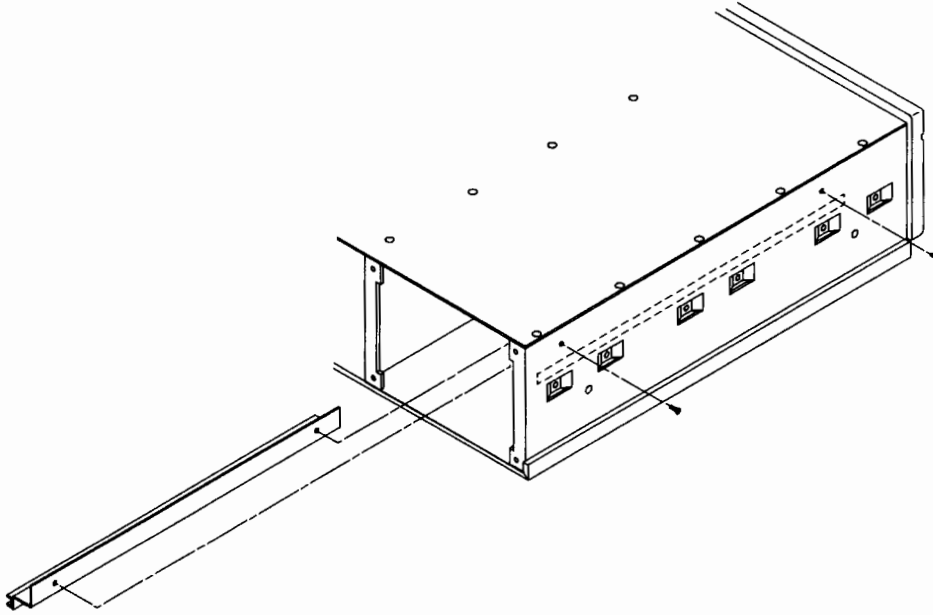
Figure 5-9. Installing the ISA Rail
