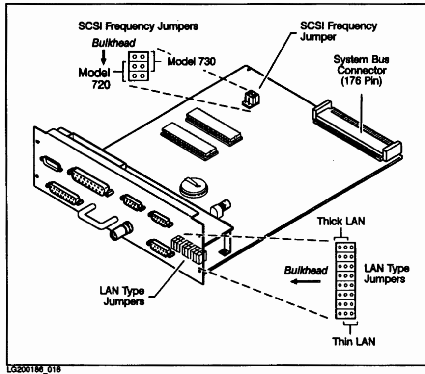
Figure 5-5. Location of the LAN Type Jumpers and SCSI Frequency Jumpers
