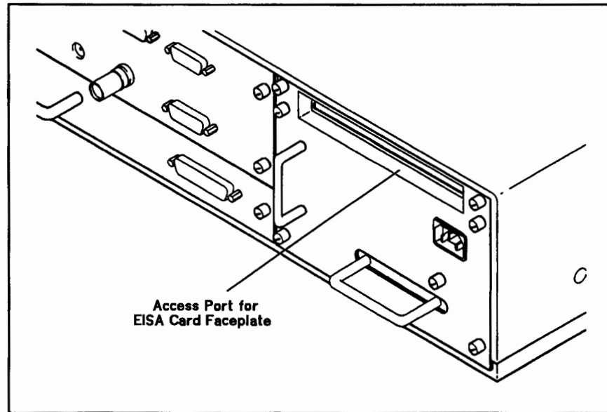
Figure 1-10. Power Supply Bulkhead with Opening for EISA Card Faceplate
