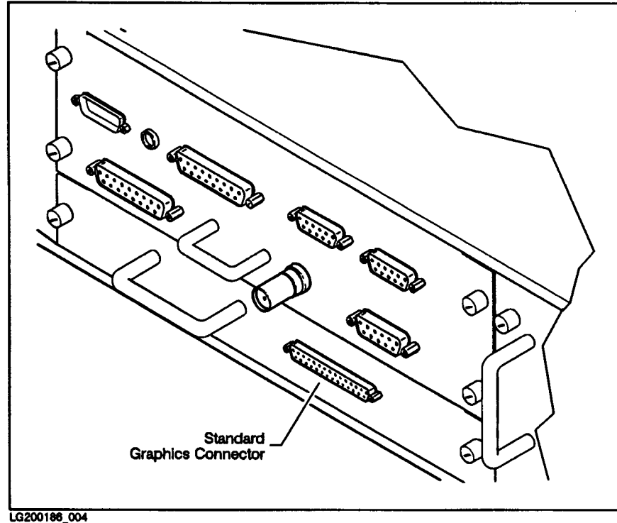
Figure 1-11. Graphic Interface Card Bulkhead
