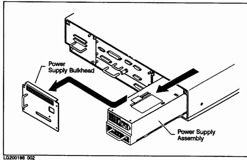
Figure 5-13. Power Supply Removal
