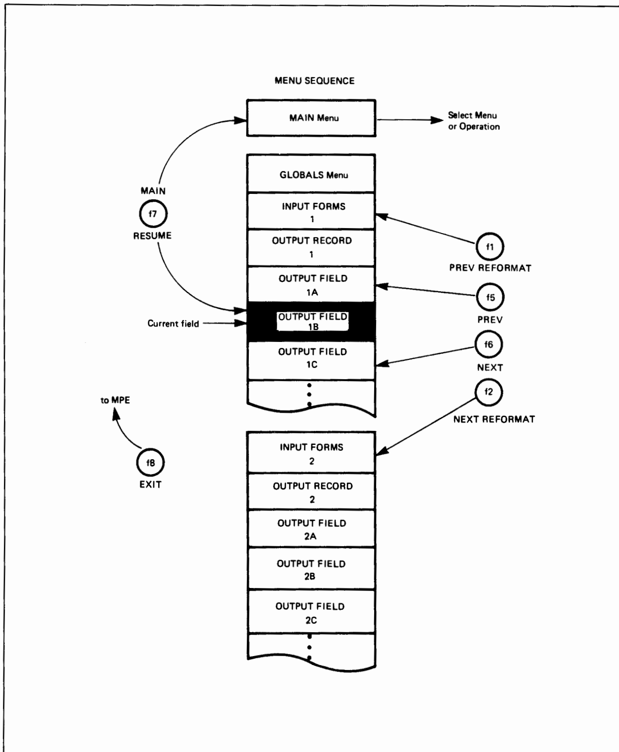
Figure 5-9. Relation of REFSPEC Menus to Function Keys
