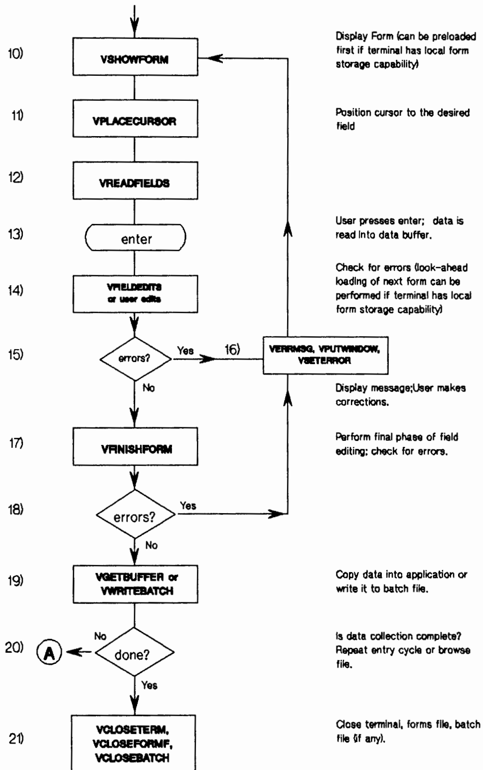
Figure 6-2. Intrinsic Flow (continued)
