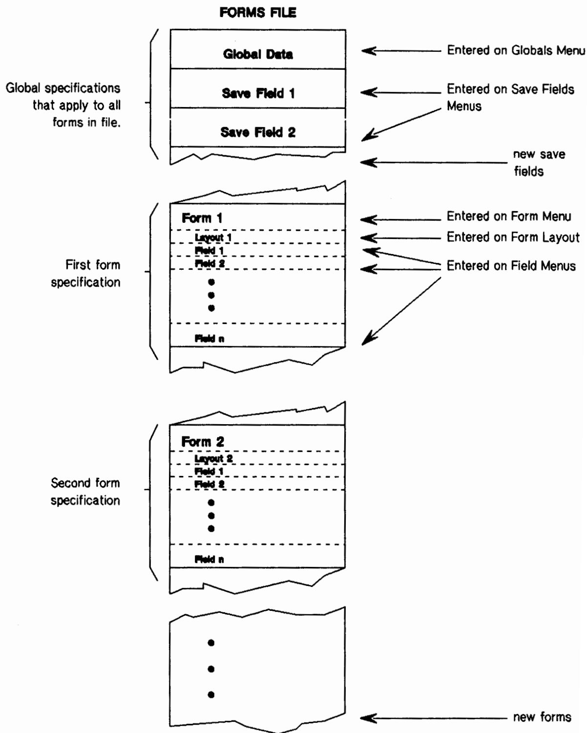
Figure 3-12. Forms File Prototype
