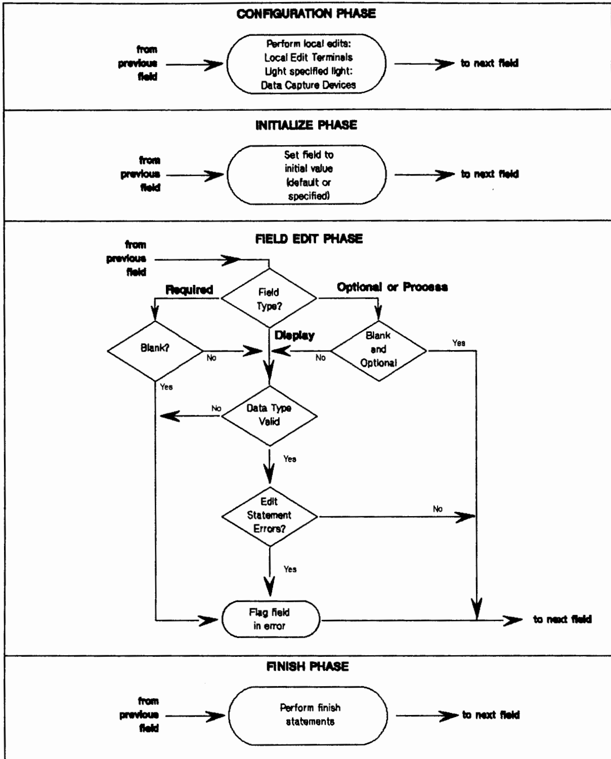
Figure 4-4. Flow of Phase Execution for ENTRY
