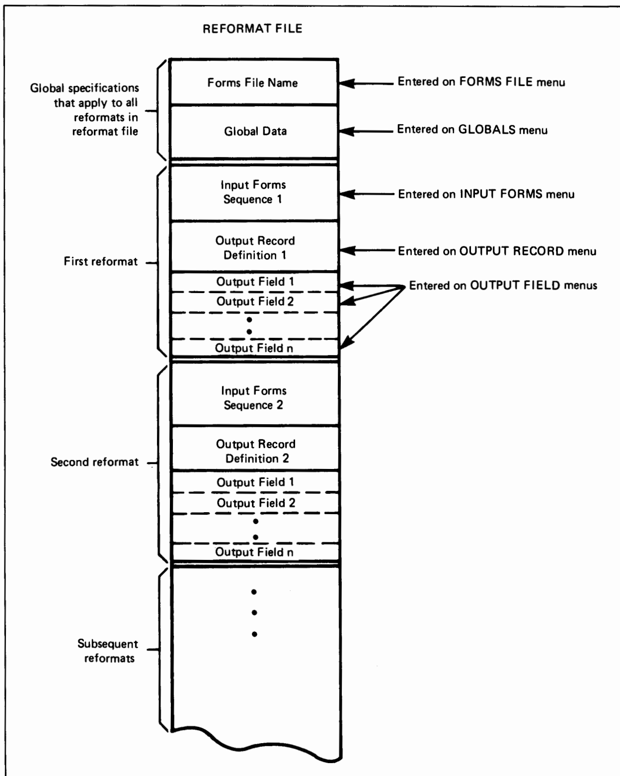
Figure 5-2. Prototype of REFORMAT File
