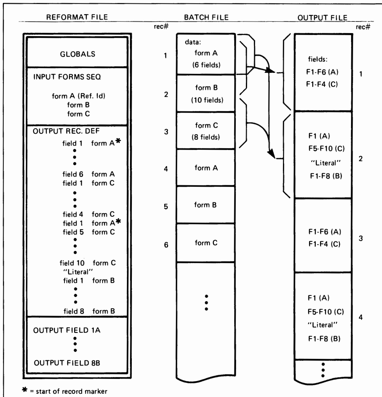
Figure 5-4. Reformat Data From 3 Forms into 2 Output Records
