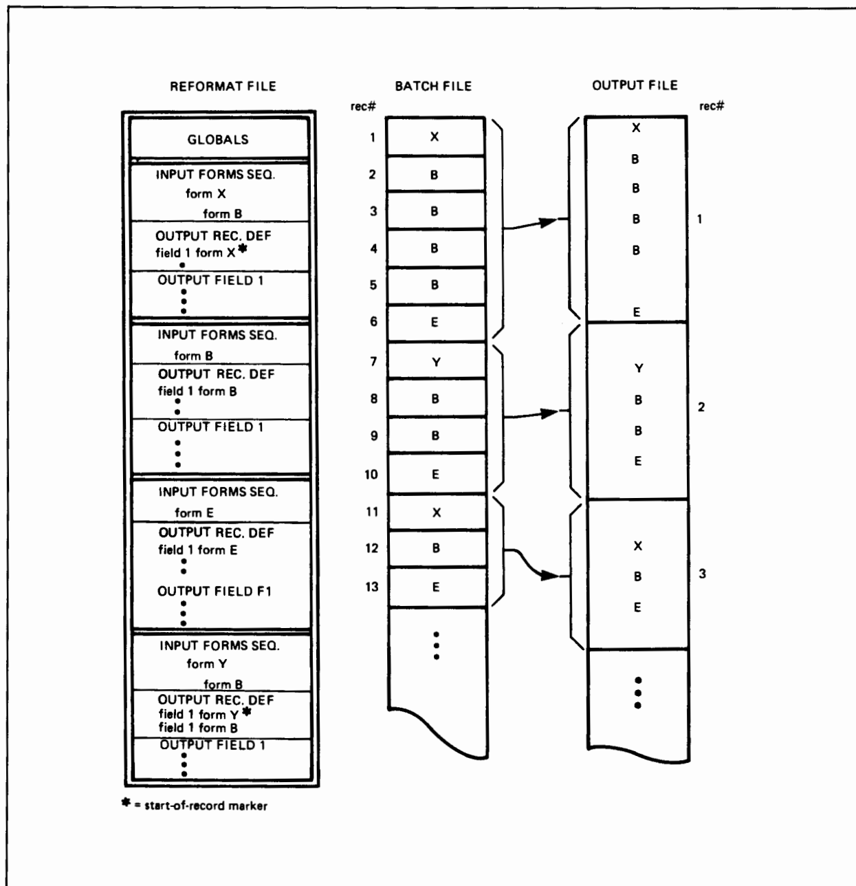
Figure 5-7. Reformatting Data Based on Form Sequence
