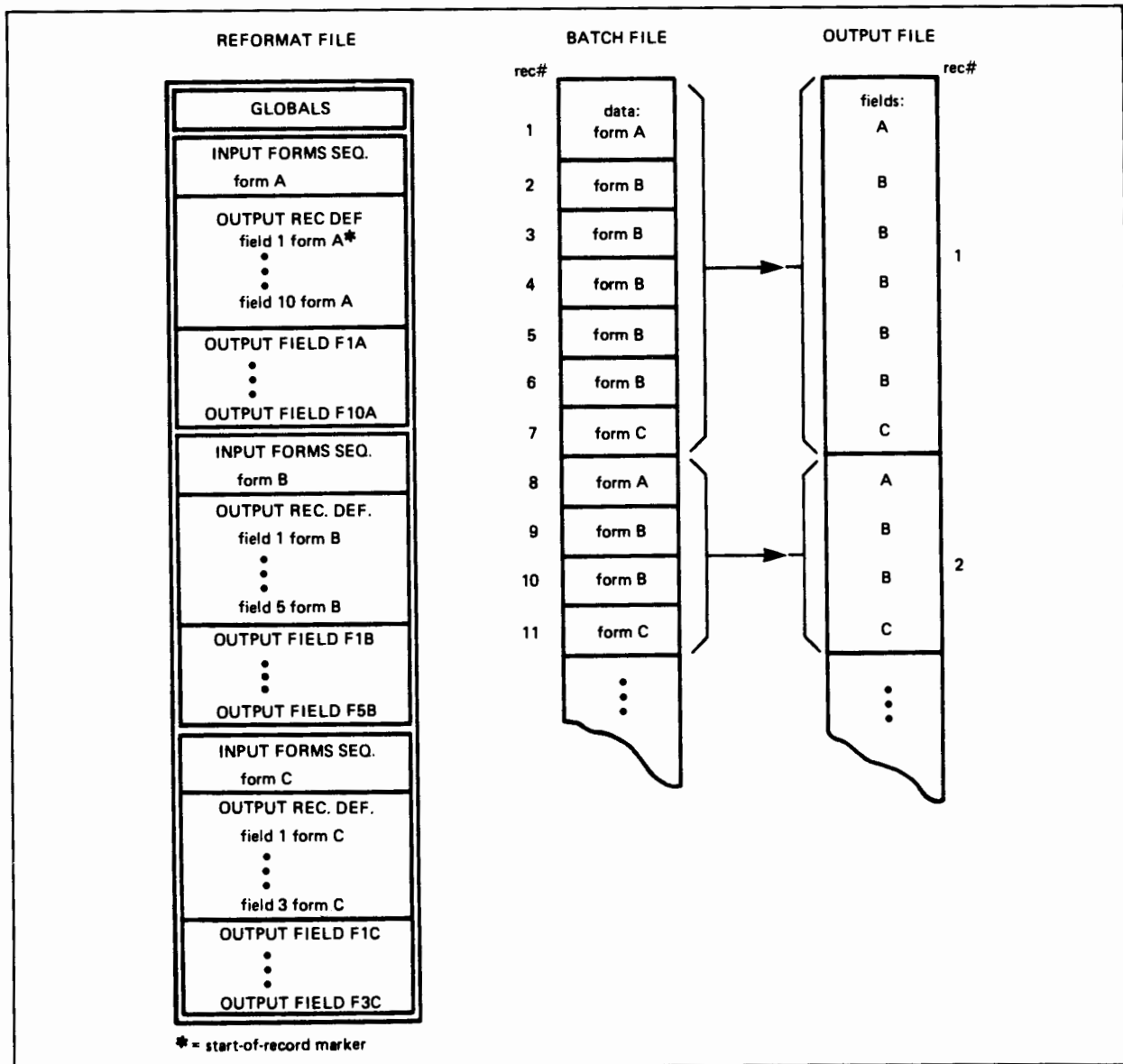
Figure 5-6. Reformatting Data From Repeating Forms
