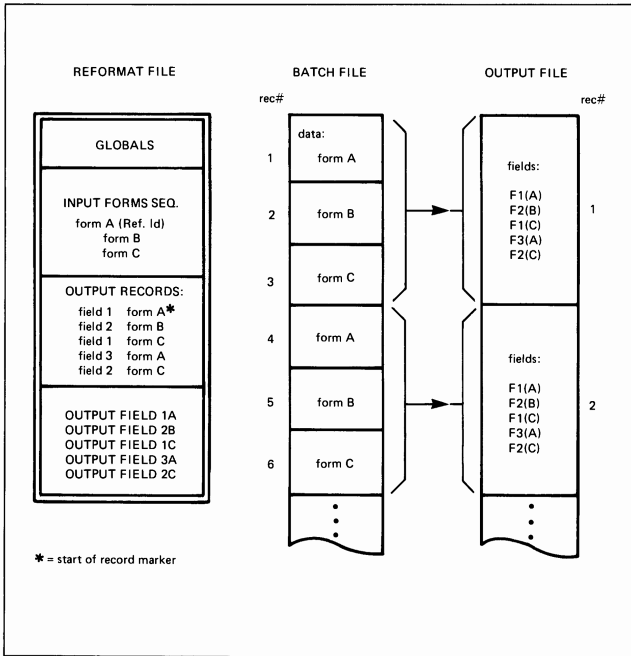
Figure 5-3. Combining Data From 3 Forms into 1 Output Record
