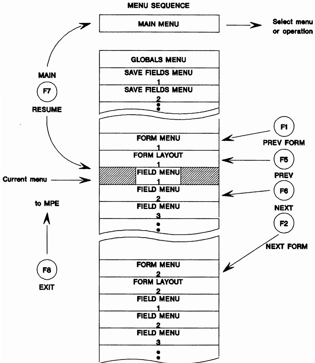
Figure 3-3. Relation Between Menus & Function Keys
