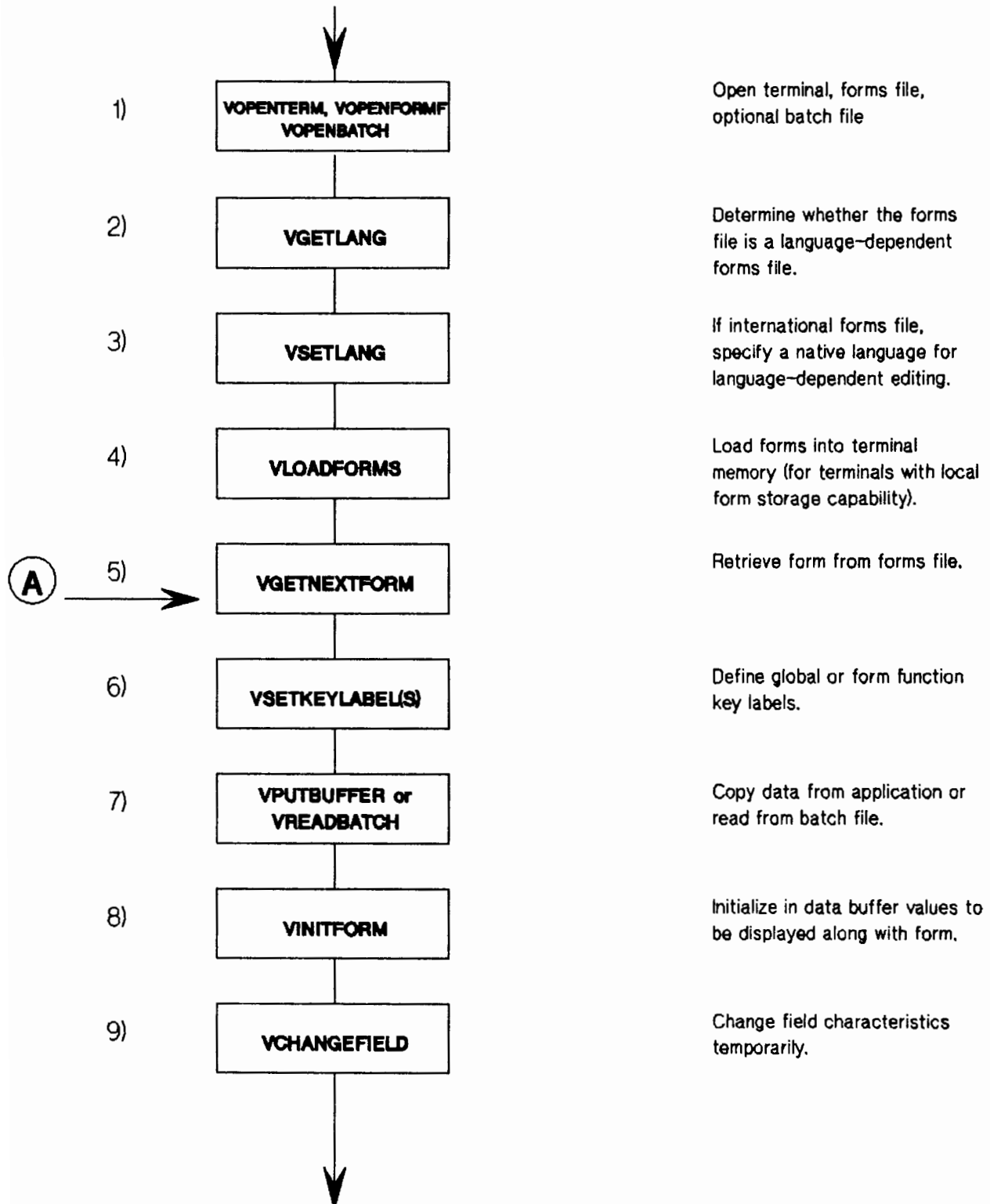
Figure 6-2. Intrinsic Flow
