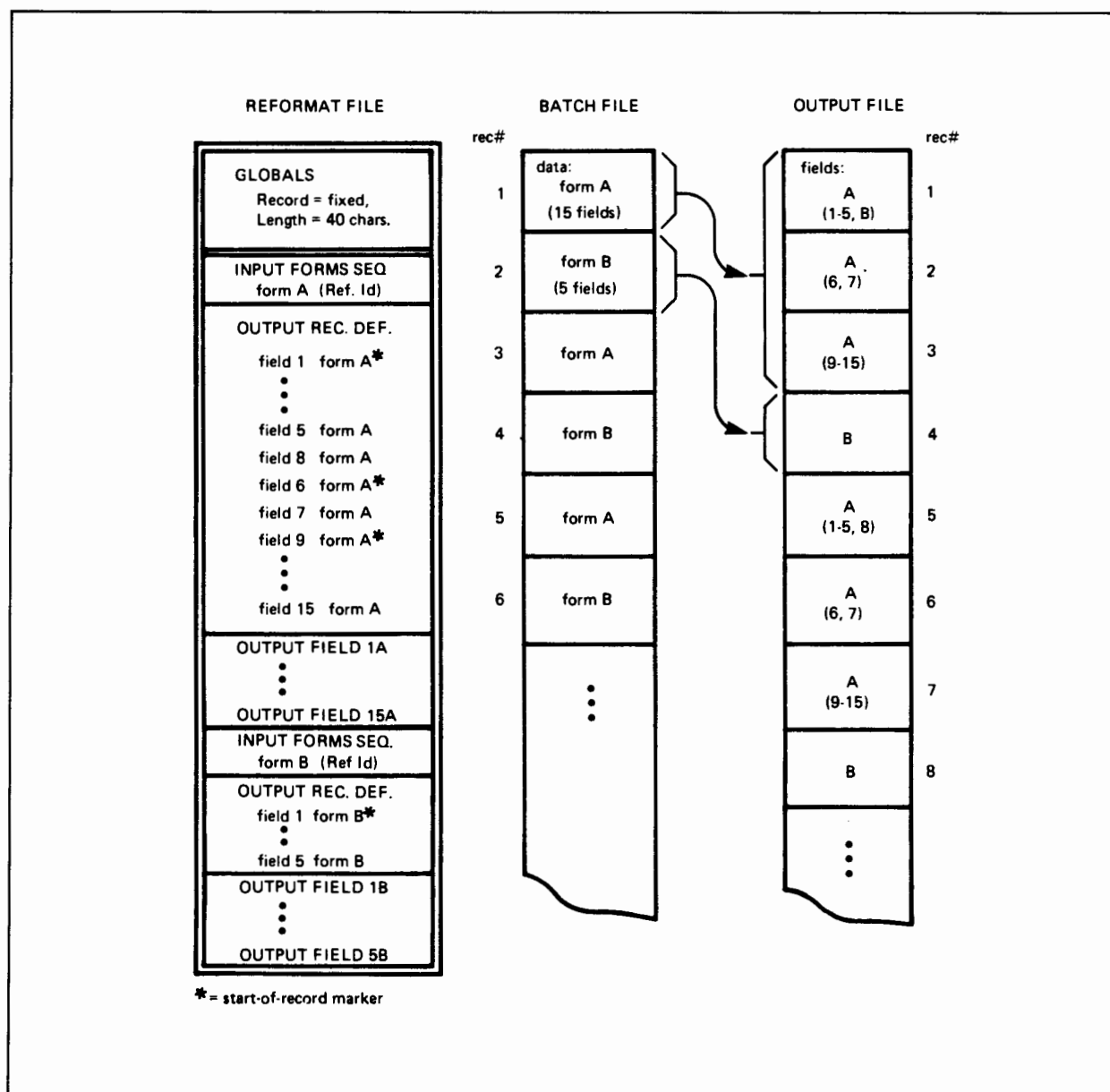
Figure 5-5. Separating Data From 1 Form into Several Records
