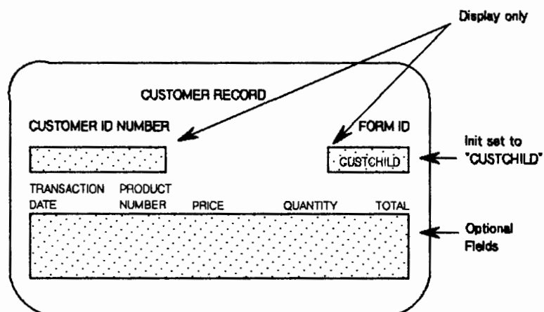
Figure 3-16. Child Form
