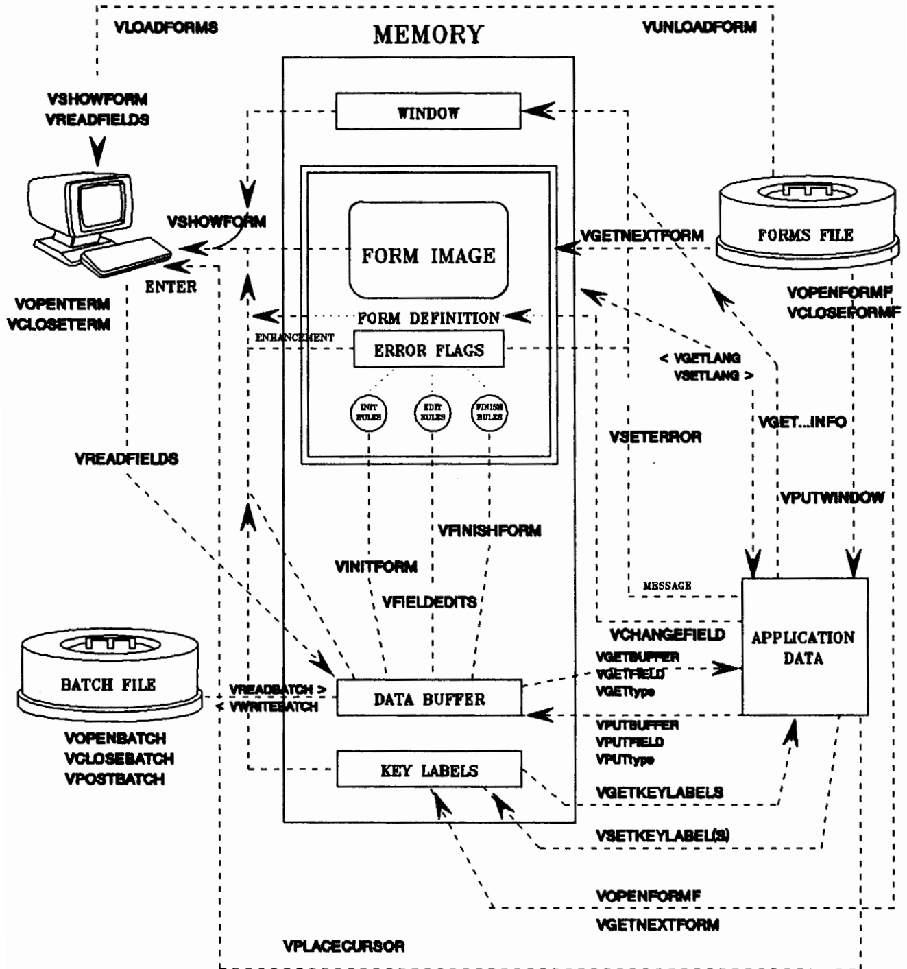
Figure 6-1. Operation of VPLUS/V Intrinsic
