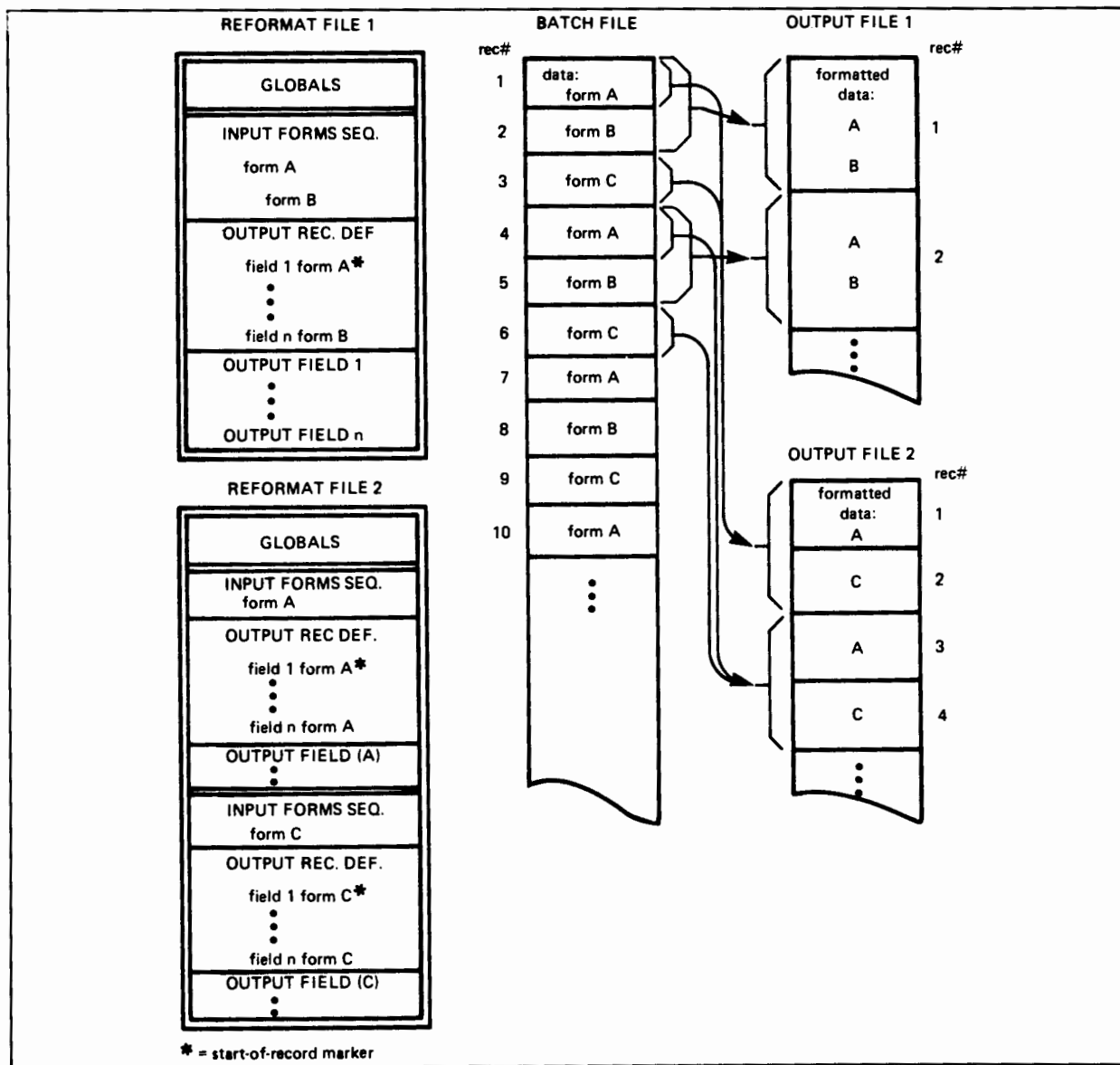
Figure 5-8. Generating 2 Output Files From 1 Batch file
