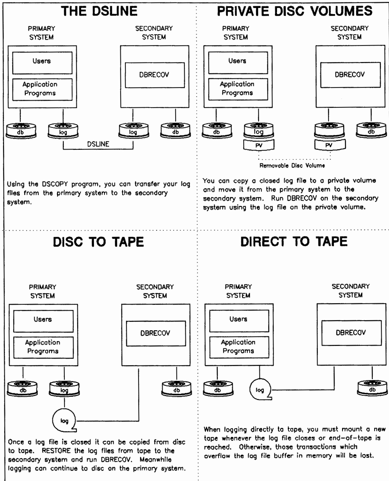
Figure 7-4. Transferring Log Files to the Secondary System
