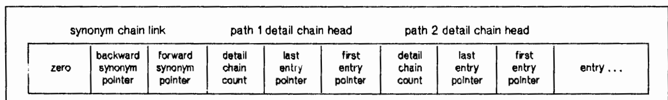
Figure 10-3. Media Record for Secondary Entry
