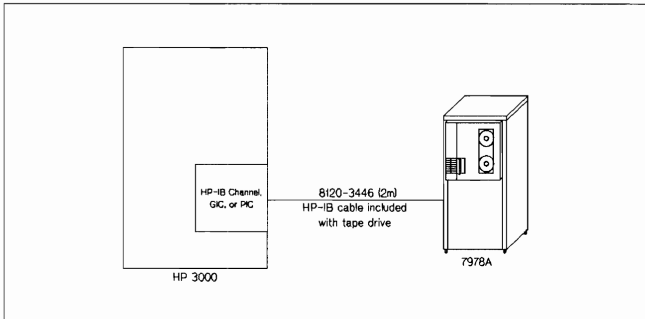
Cable Configuration for 7978A/B Tape Drive
