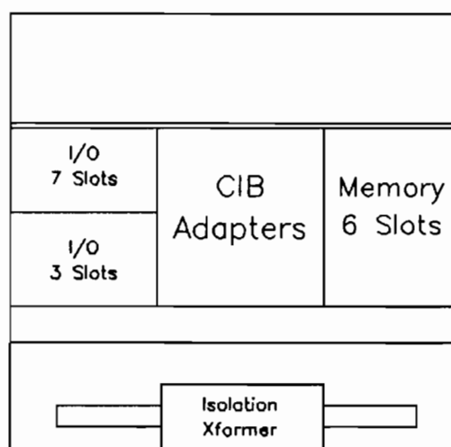
Rear View
