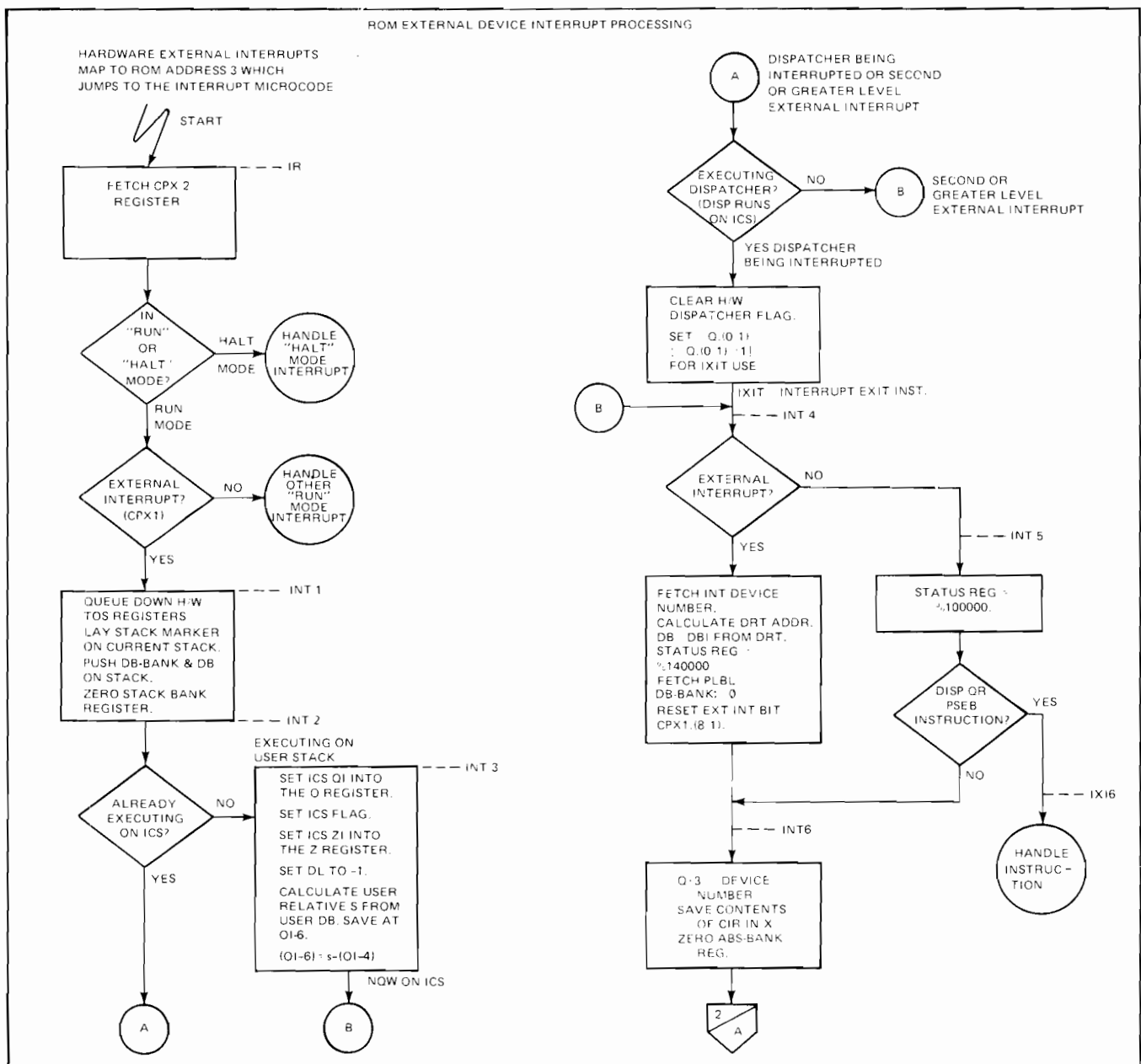
Figure 6-8. Interrupt Handler
