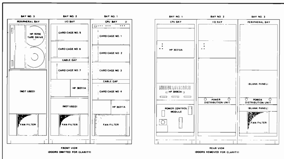
Figure 1-2. 3-Bay Computer System
