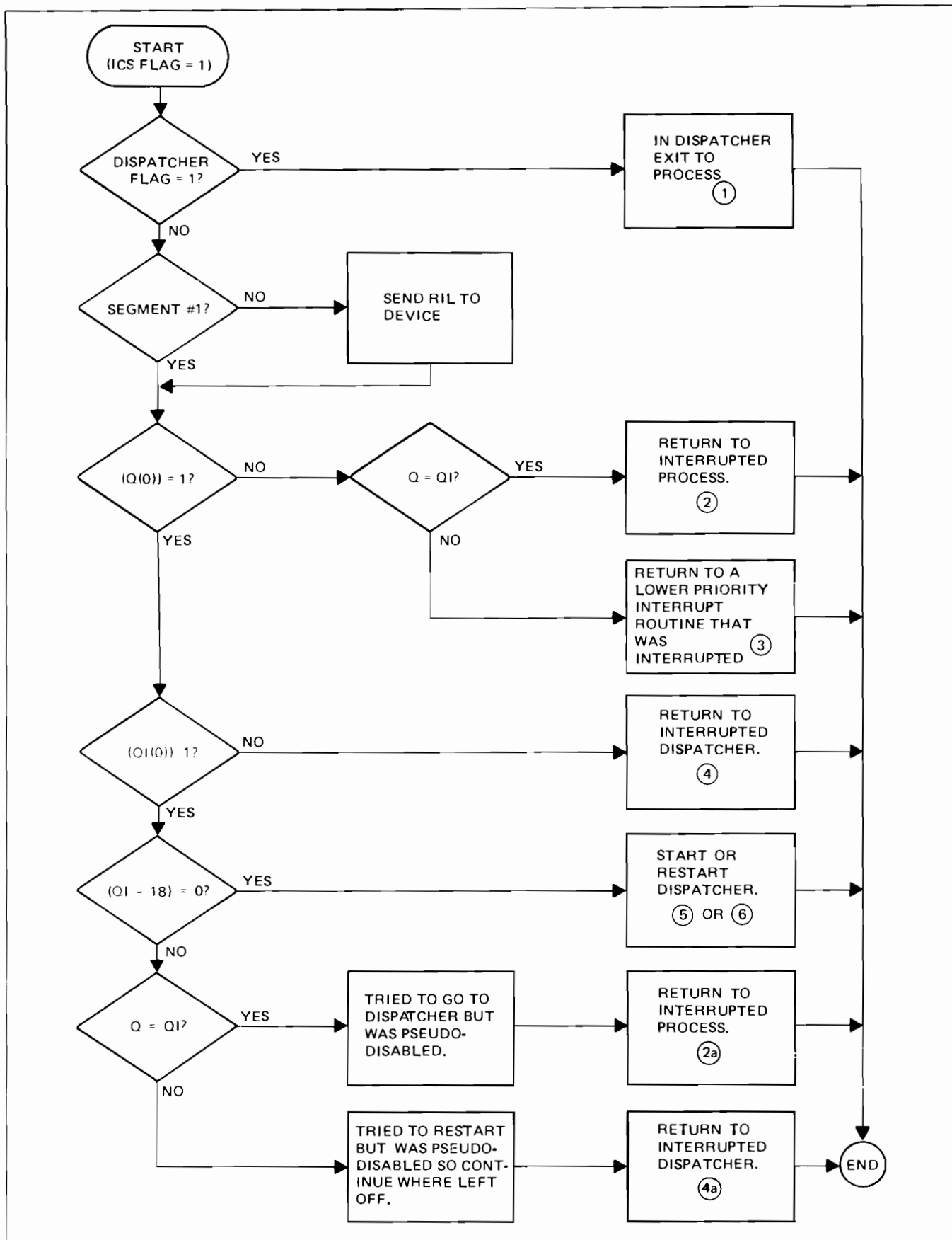
Figure 6-9. IXIT Instruction
