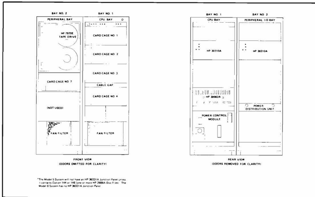
Figure 1-1. 2-Bay Computer System
