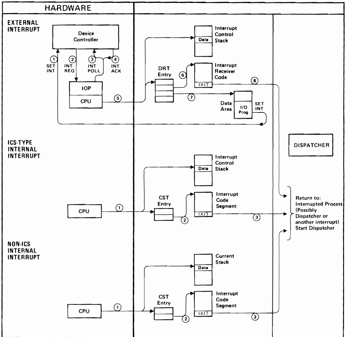
Figure 6-2. Interrupt System Overview
