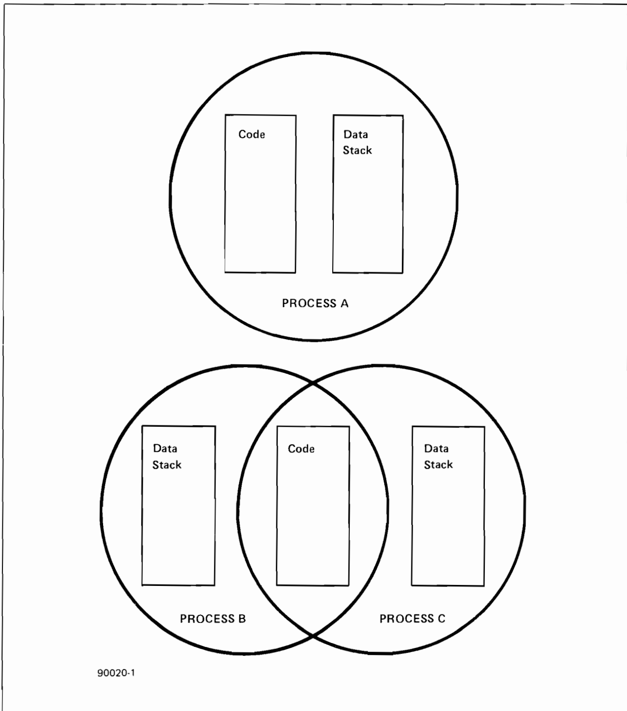
Figure 4-1. Code Sharing and Data Privacy
