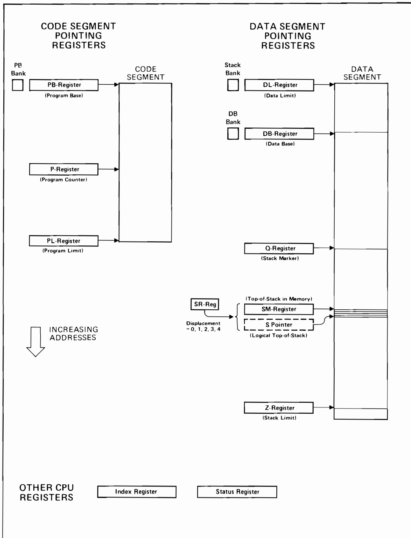
Figure 3-6. CPU Registers
