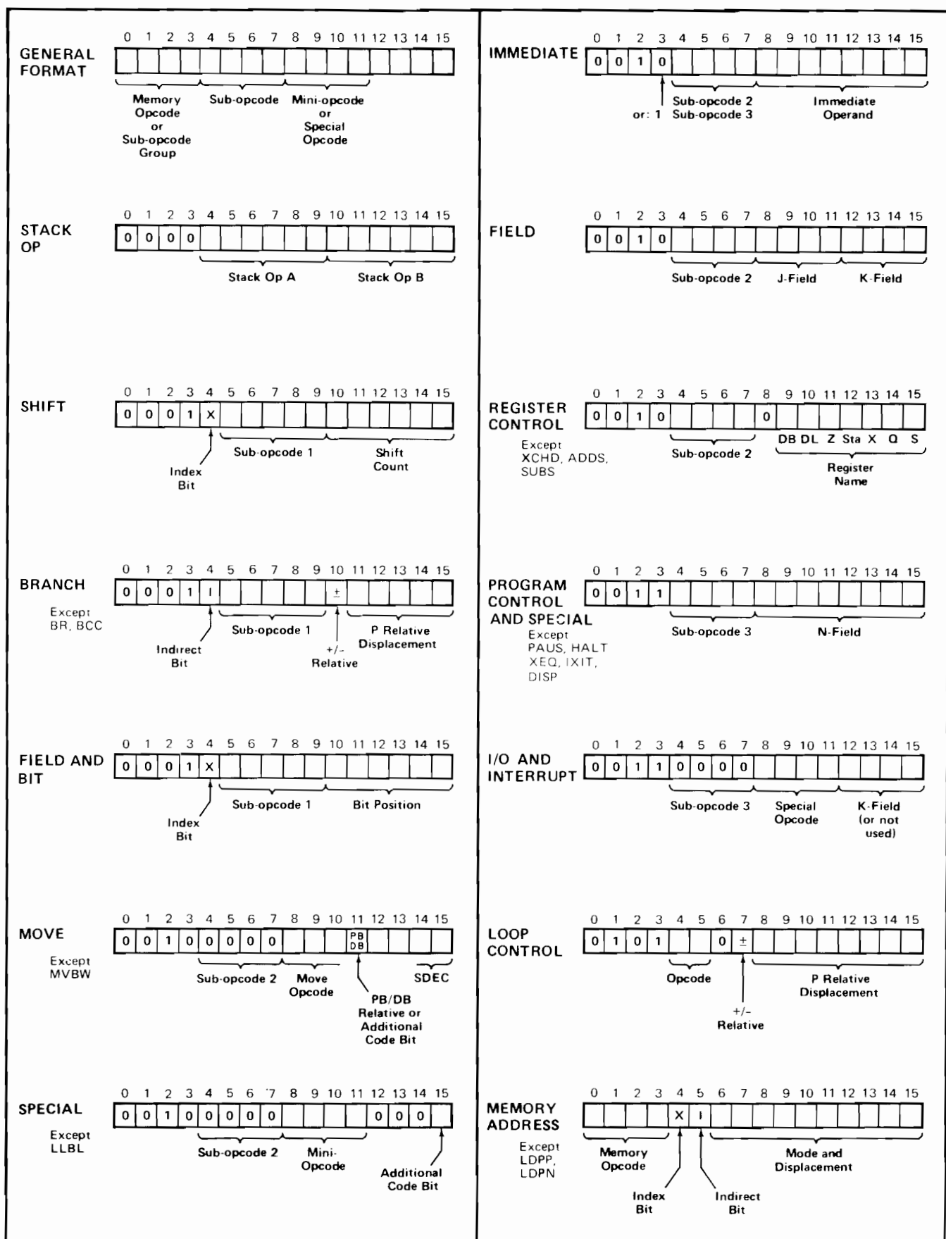
Figure 3-4. Instruction Groups
