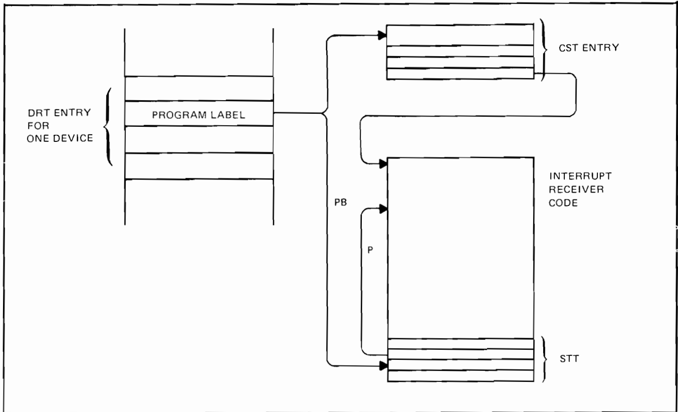
Figure 6-3. Device Controller
