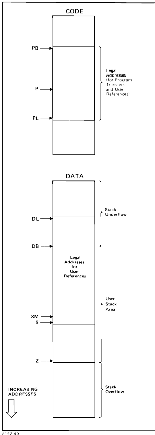
Figure 3-11. Addressing and Stack Bounds
