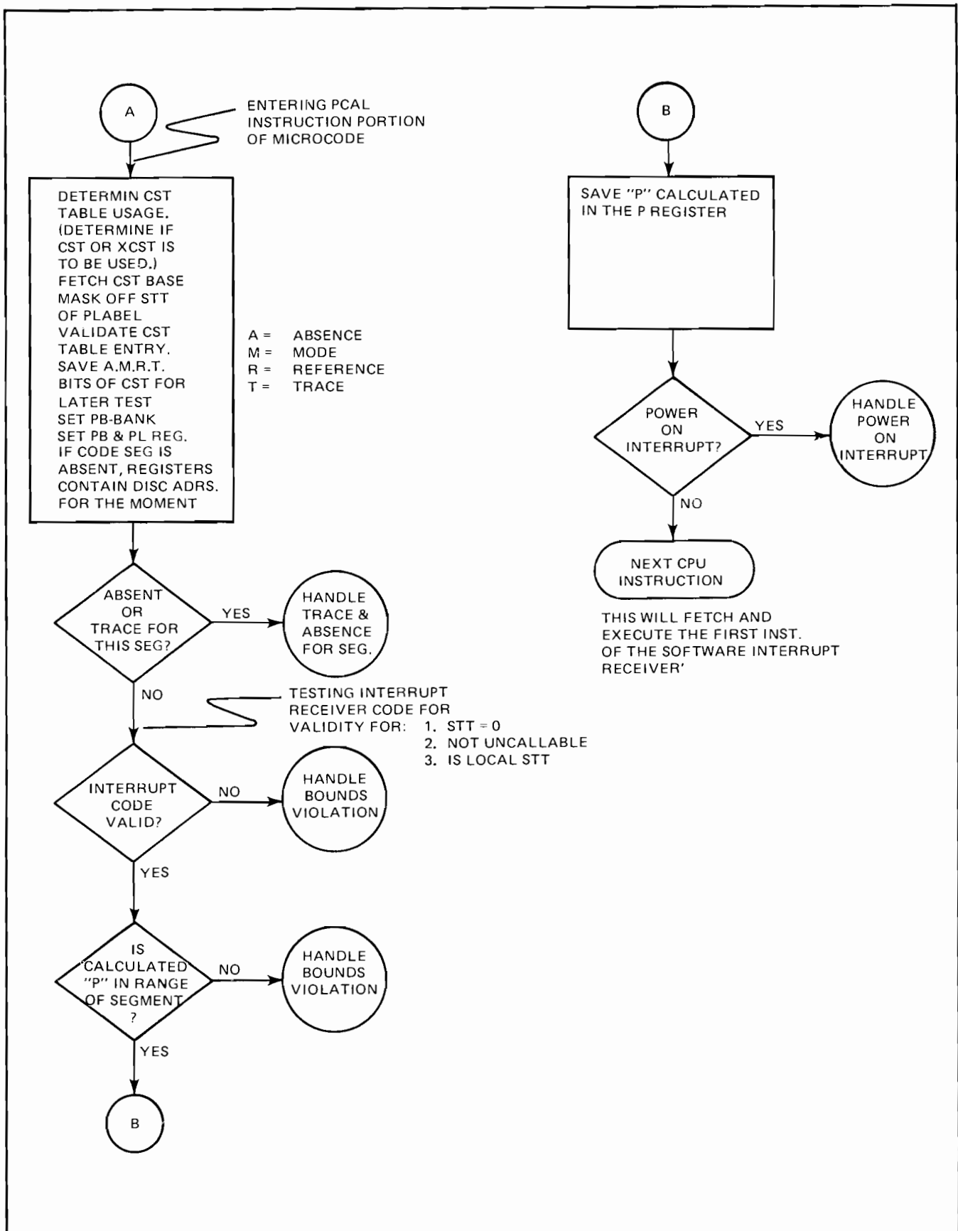
Figure 6-8. Interrupt Handler (Continued)
