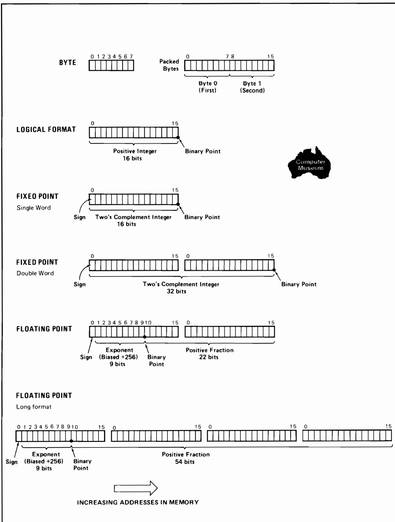
Figure 3-2. Data Formats
