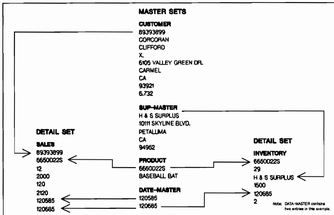
Figure 1-2. Sample Entry Values
