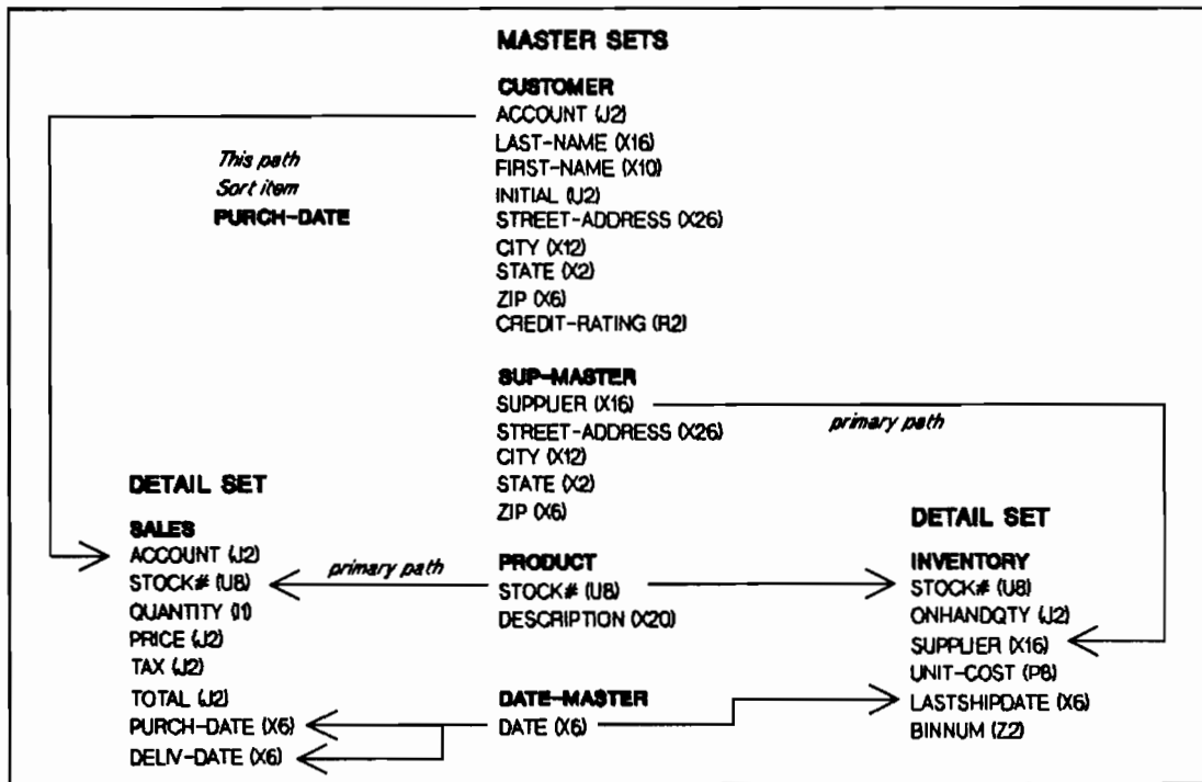
Figure 1-1. ORDERS Data Base Structure
