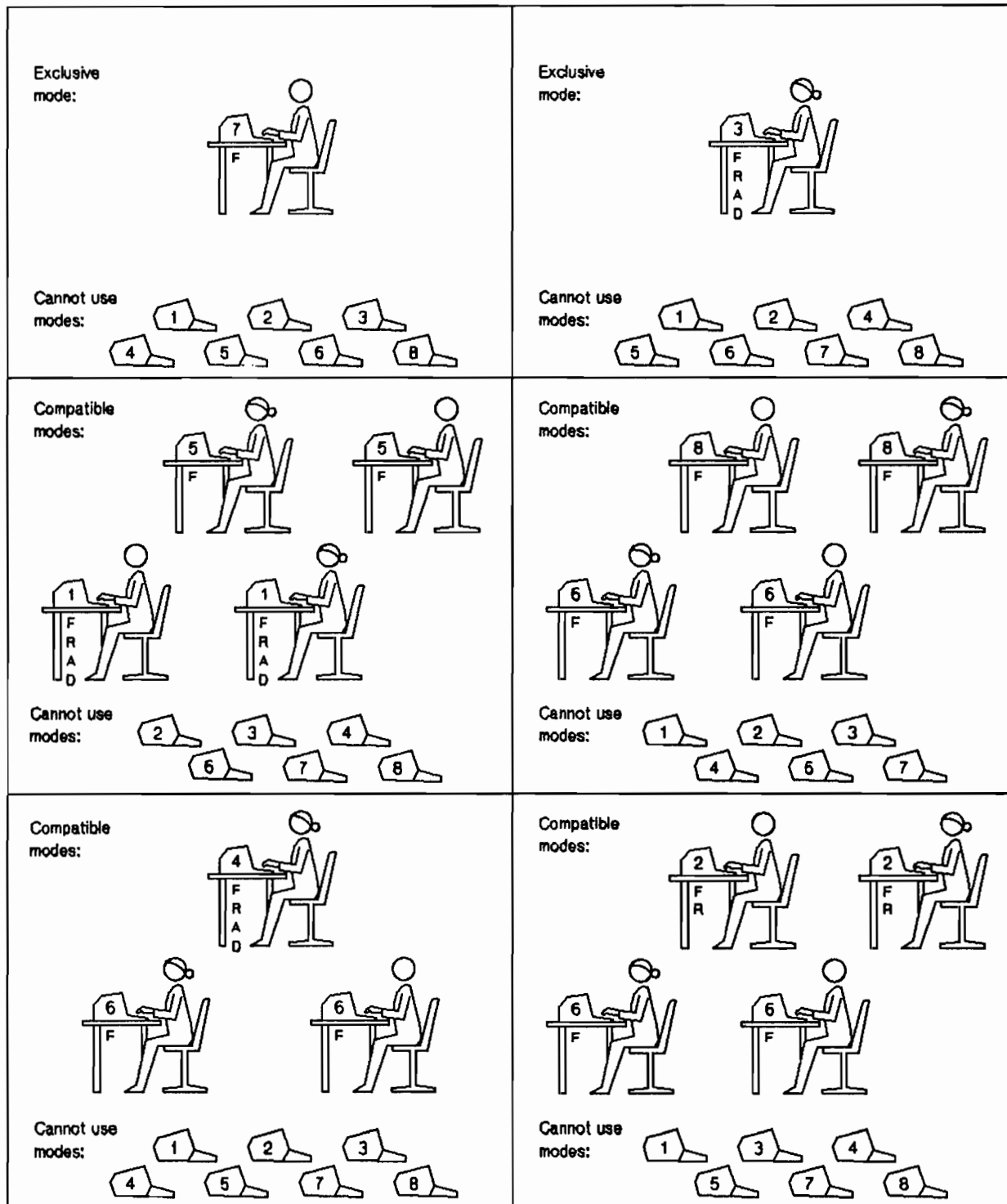
Figure 1-3. IMAGE/QUERY Environments
