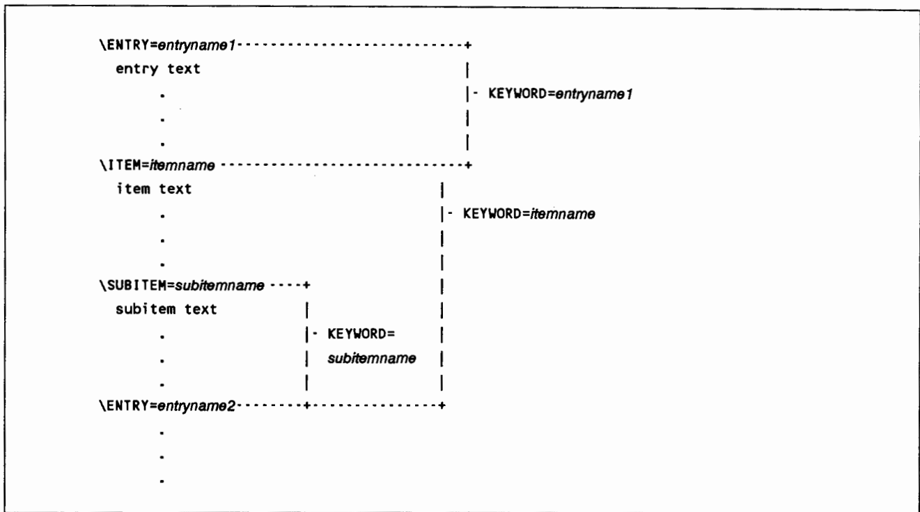
Figure 2-6. Keyword Subdivisions
