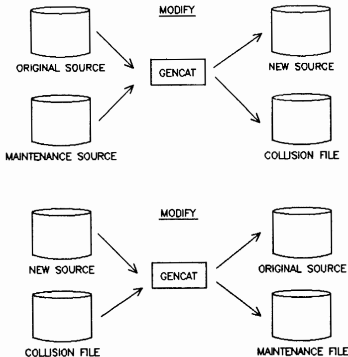
Figure 2-3. Collision Files
