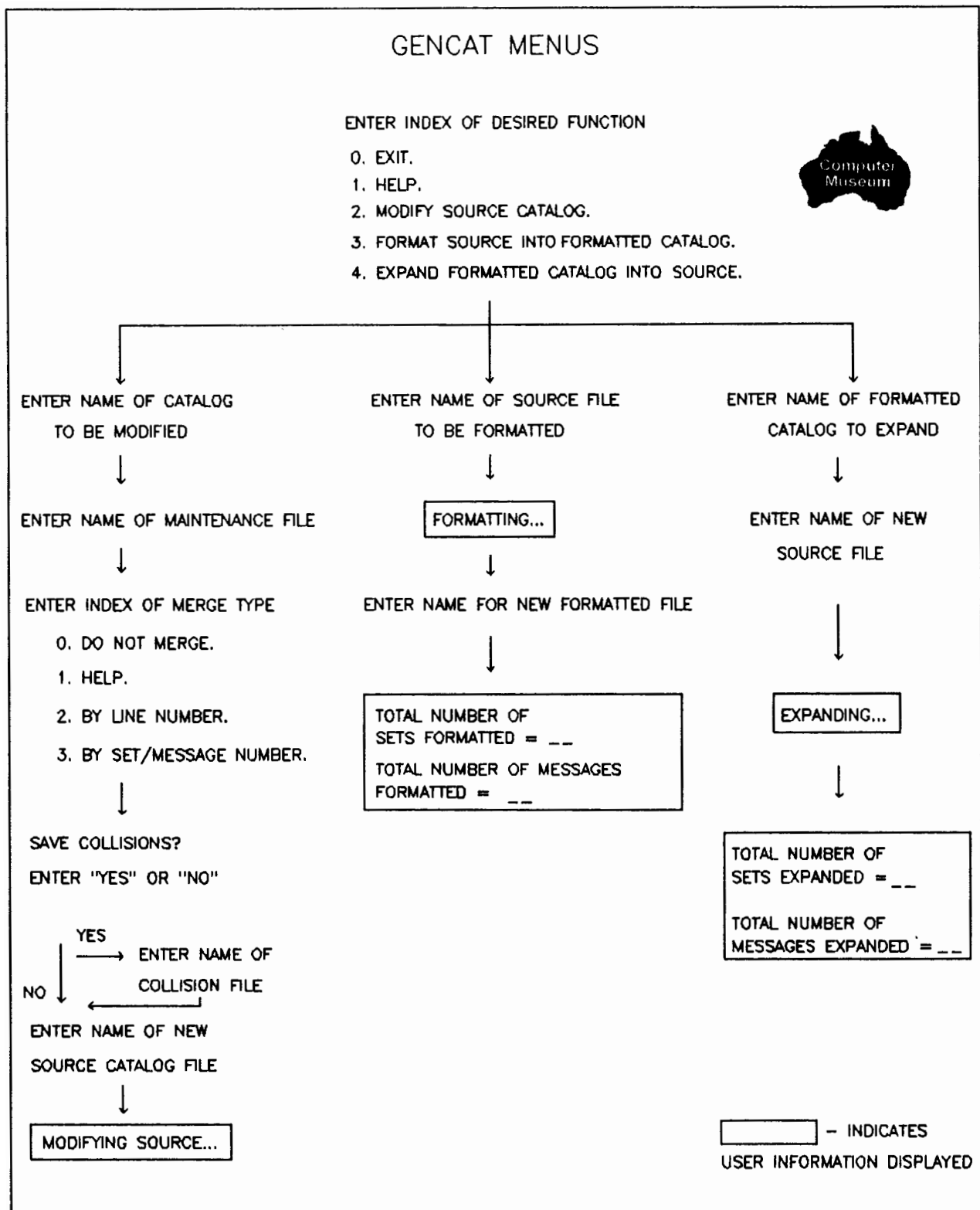
Figure 2-2. GENCAT Functions
