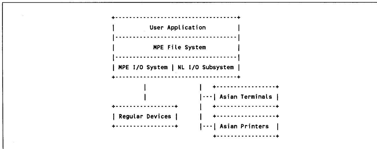
Figure 3-2. NL I/O Subsystem Structure
