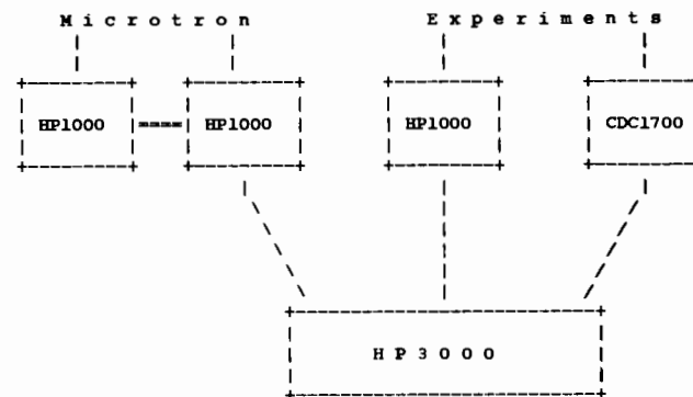
Fig. 1: Overview of our distributed computer system (the CDC1700 will be replaced by a PE3220 system).
