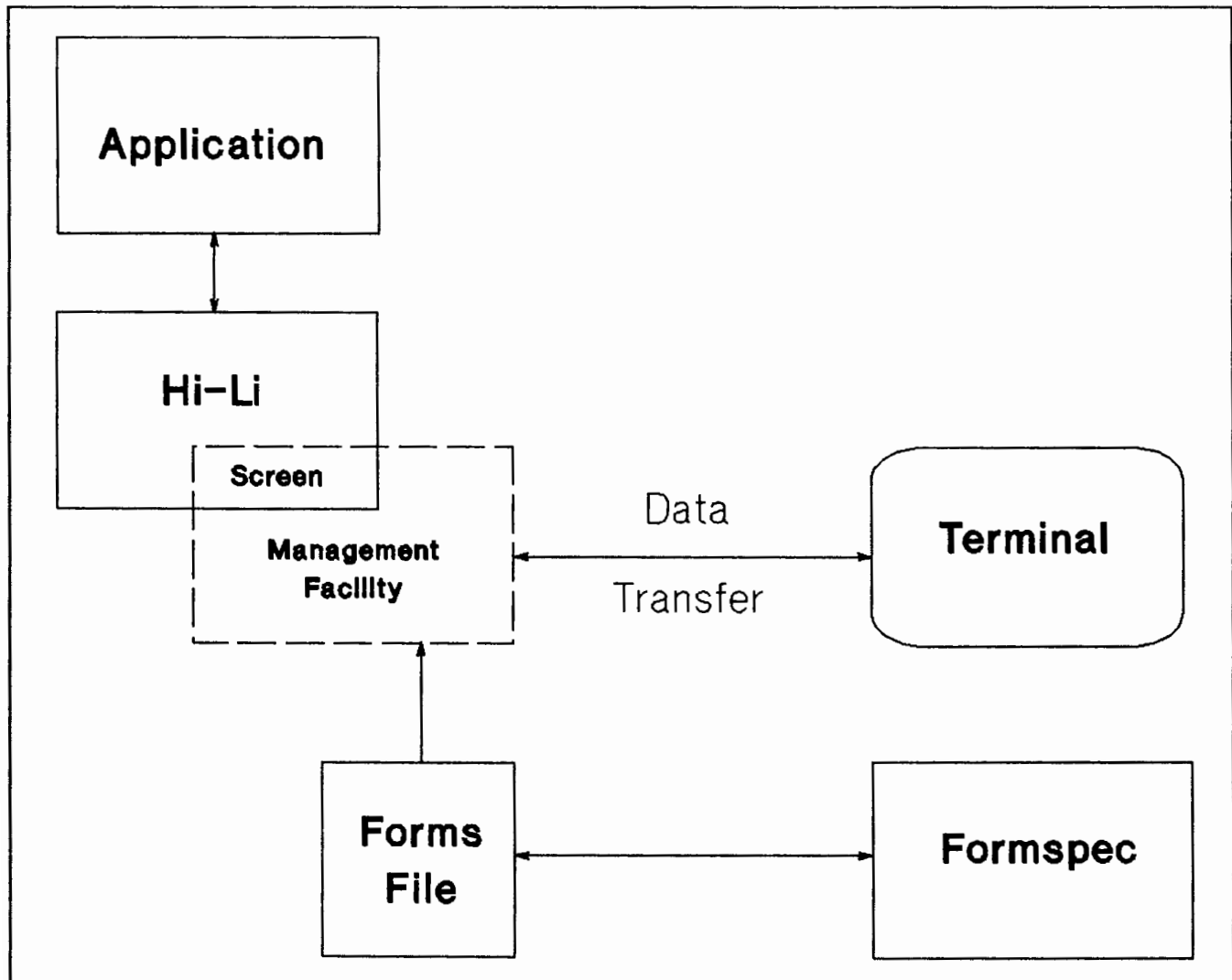
Figure 1-2. Hi-Li and the Transfer of Data
