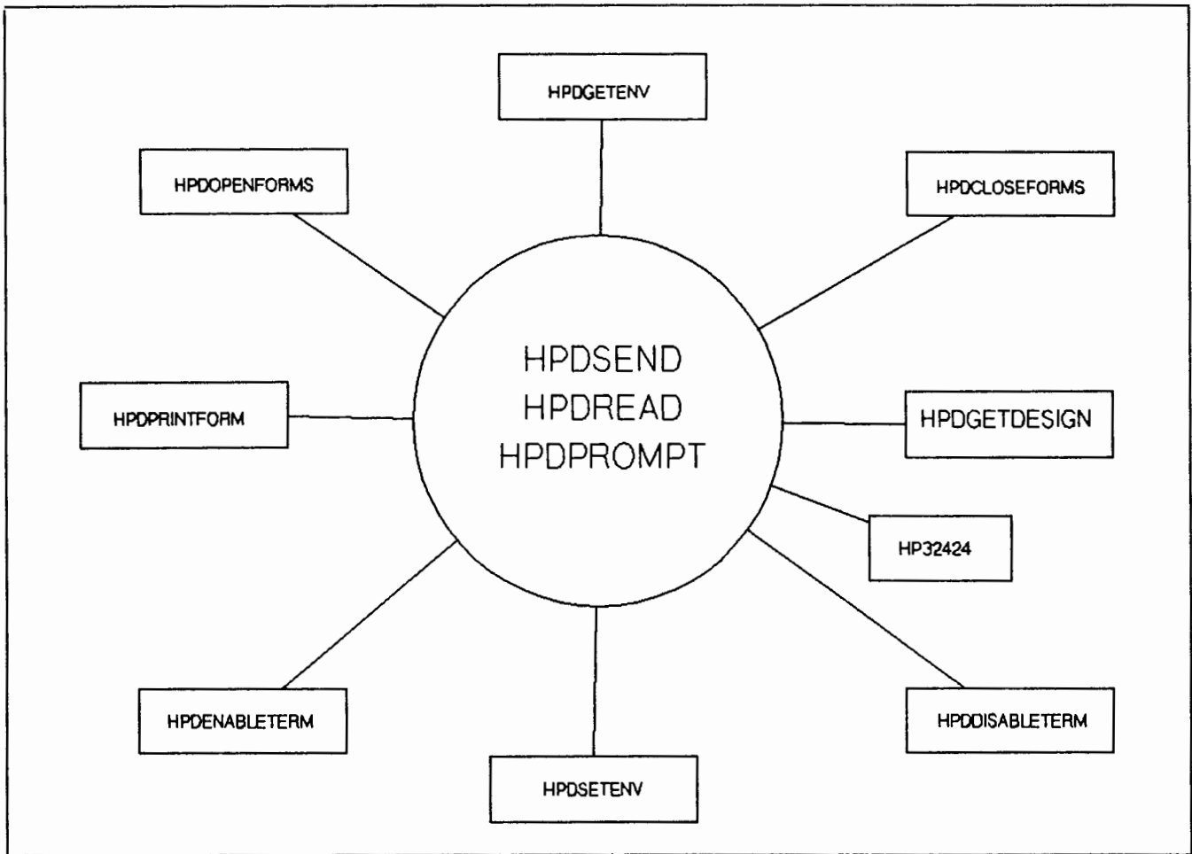
Figure 2-1. Core and Supporting Intrinsics
