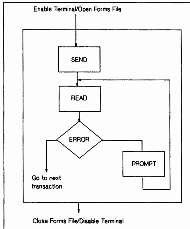
Figure 2-2. The Hi-Li Model
