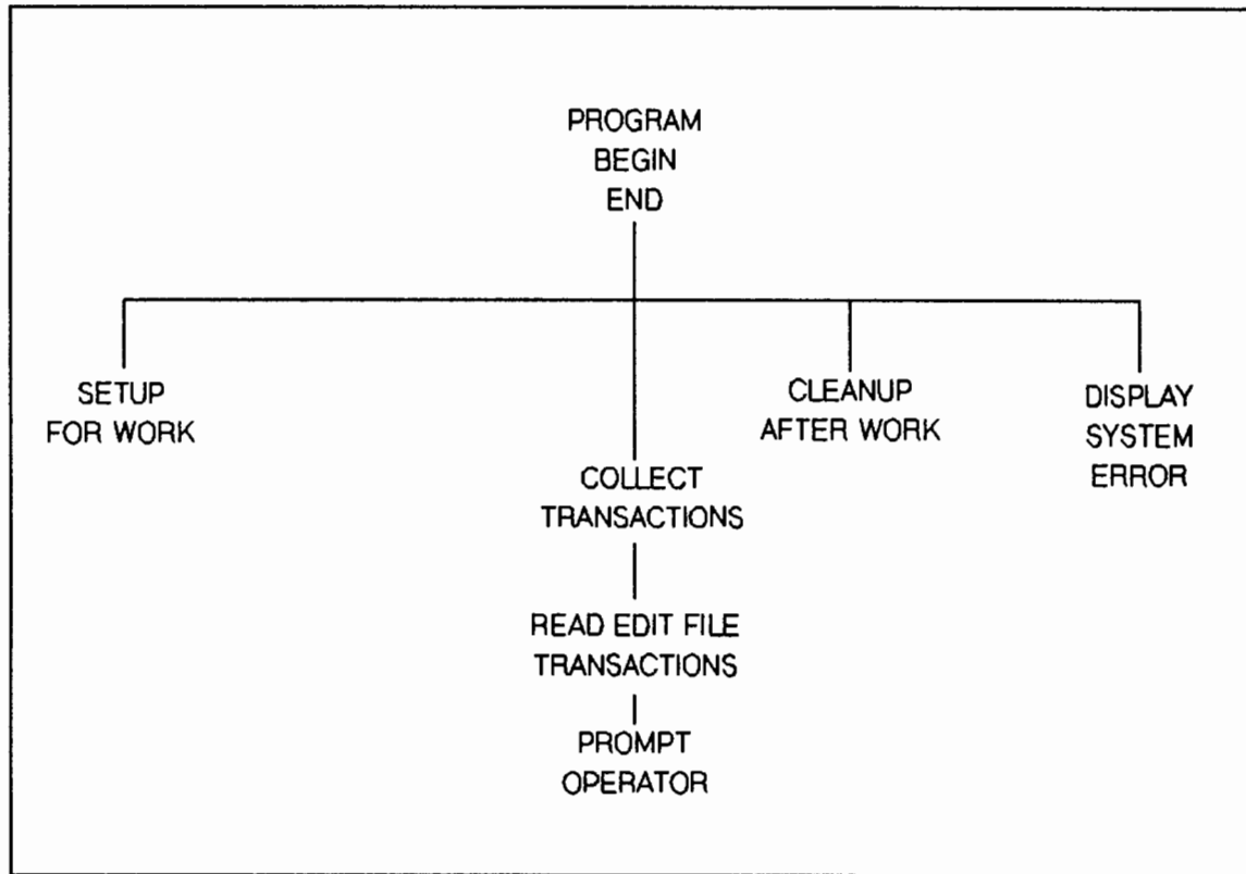
Figure C-1. Structure of the Application Program
