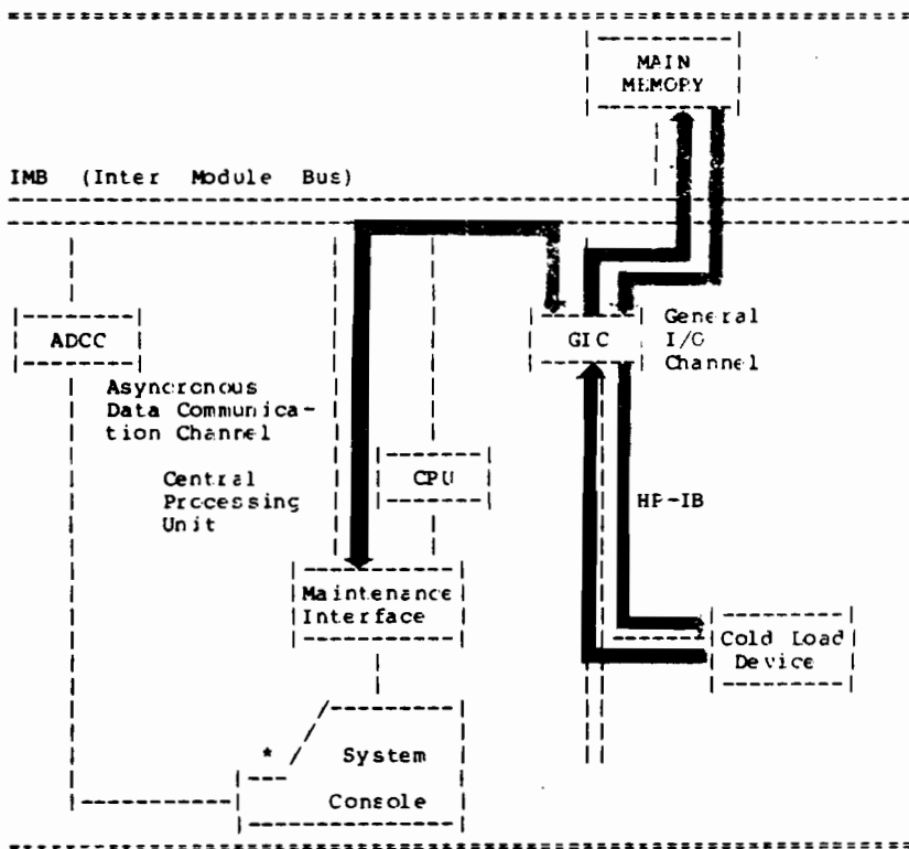
Figure 4-5. Test Write/Read Loopback
