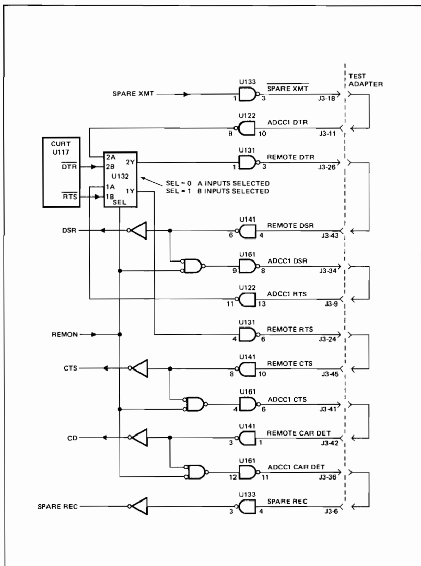
Figure 3-8. Data Comm Test Adapter Configuration
