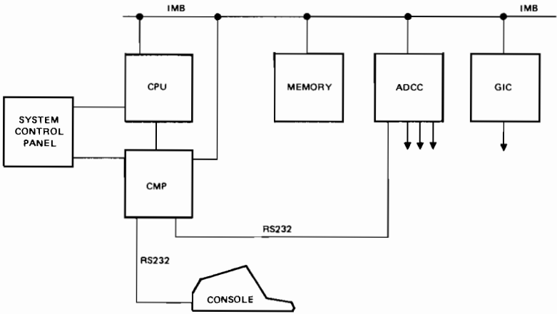
Figure 1-1. System Architecture for CMP/SYSTEM Selftest
