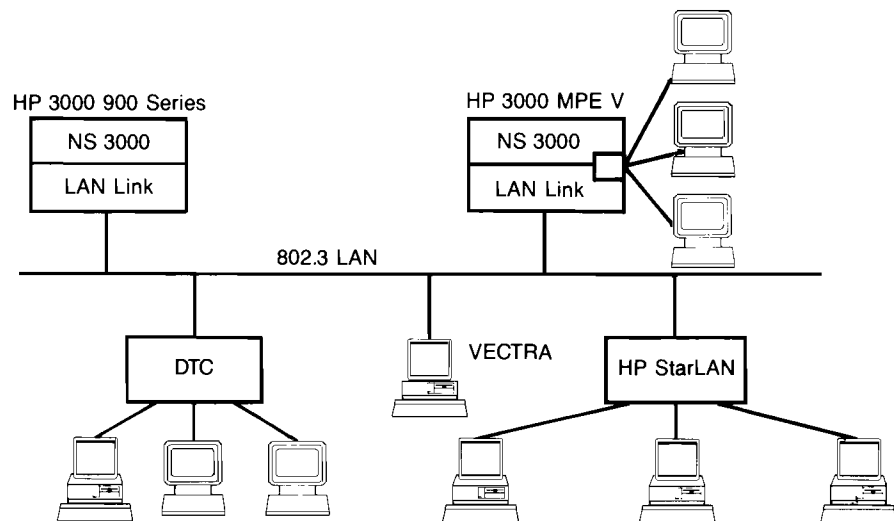
Figure 6-6. NS3000 over a LAN
