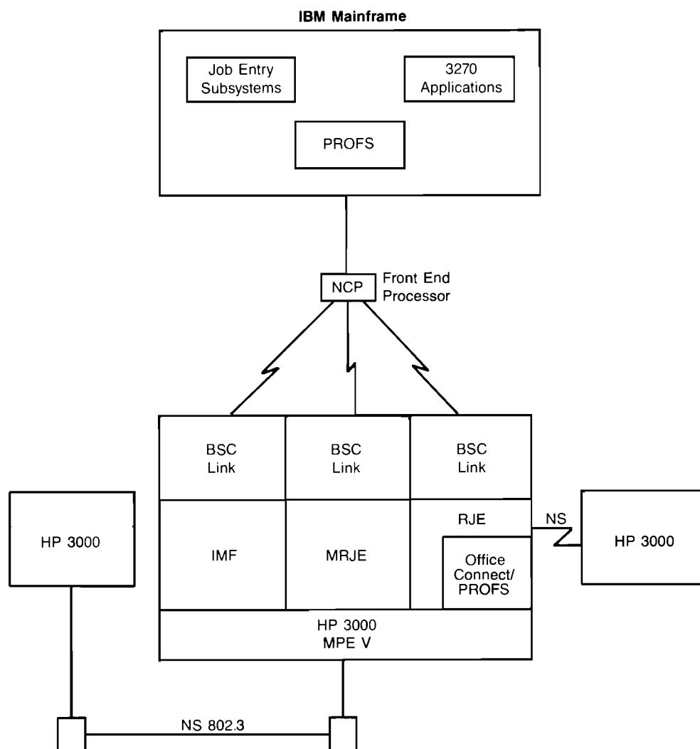
Figure 6-10. BSC Communication
