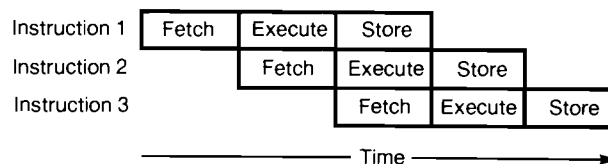
Figure 4-4. Instruction Pipeline
