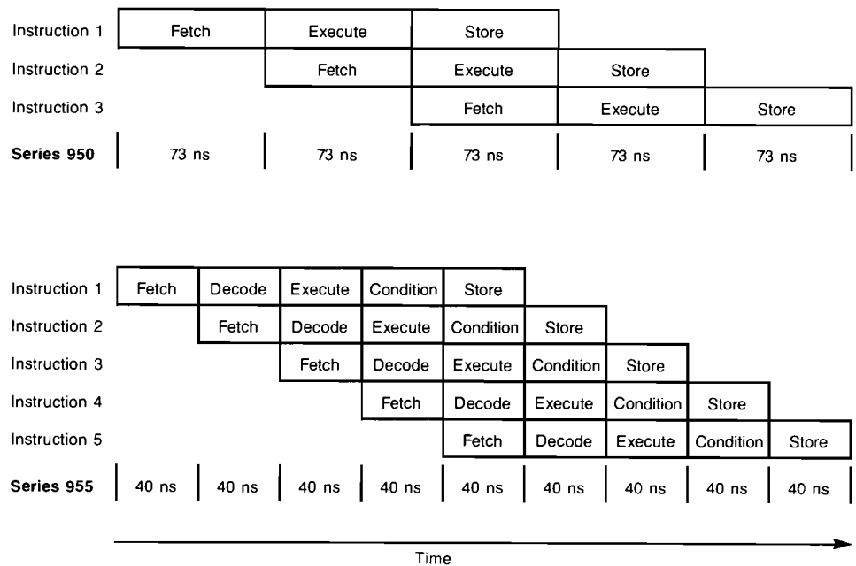
Figure 5-20. Instruction Pipelining
