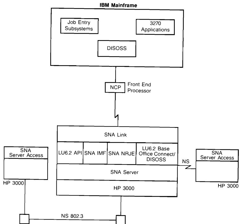
Figure 6-9. SNA Communication
