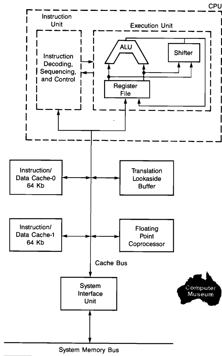
Figure 5-19. The Series 950 Processor
