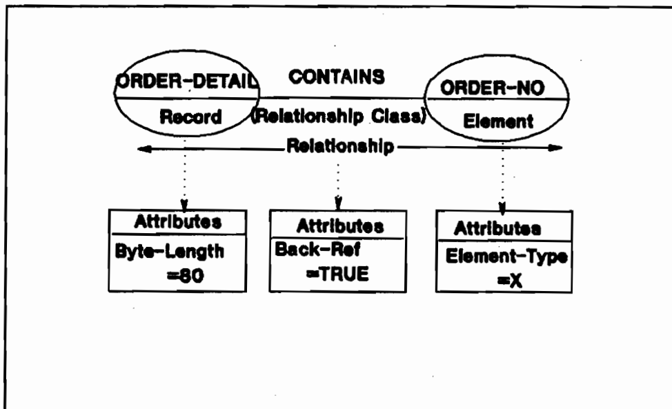
Diagram 1: Entity-Relationship Model
