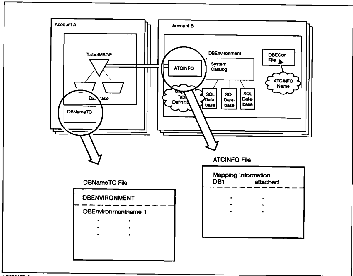
Figure 3-1. Files Created by IMAGE/SQL
