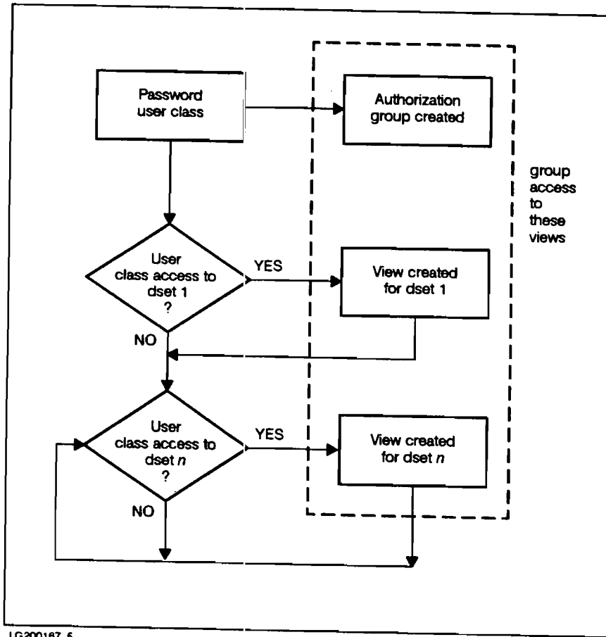
Figure 3-4. IMAGE/SQL Security Mapping
