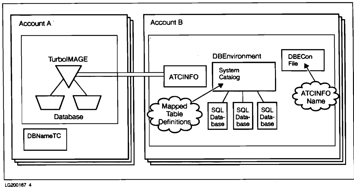
Figure 3-3. An Attached TurboIMAGE/XL Database
