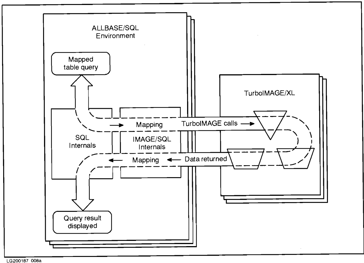
Figure 3-5. IMAGE/SQL at Run Time
